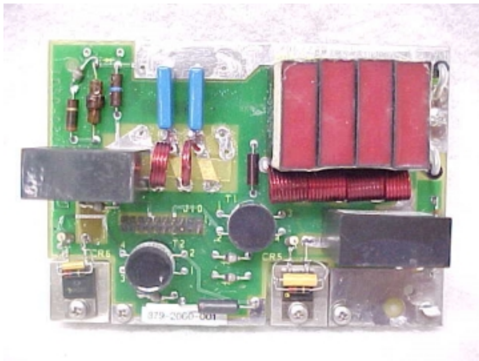
Internal Modulator Front
