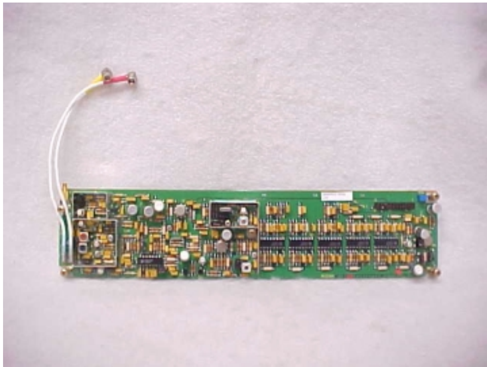
Internal Rx Front
