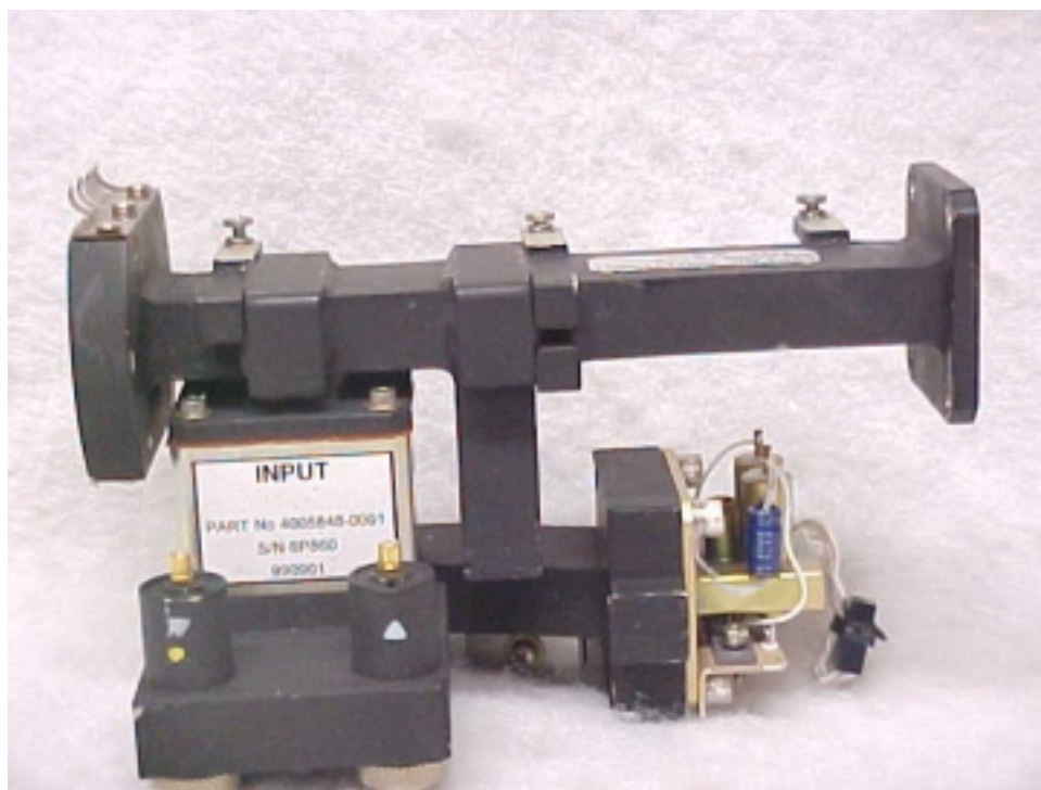
Internal Waveguide Assembly Side
