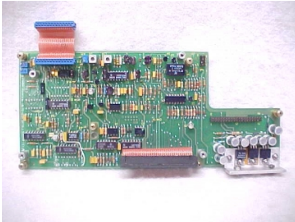
Internal Analog Video Front
