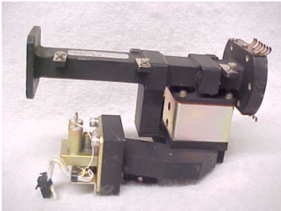
Internal Waveguide Assembly
