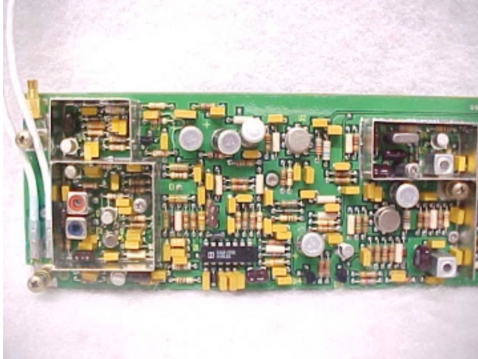
Internal Rx Close up Half
