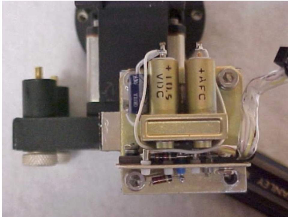
Internal VCO
