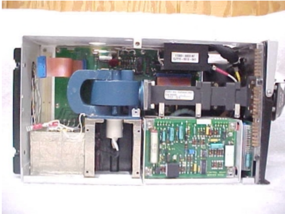
Internal Magnatron Waveguide in place
