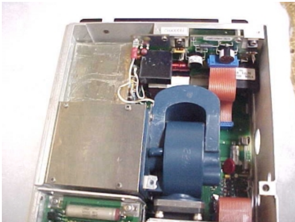
Internal Tx Section in place
