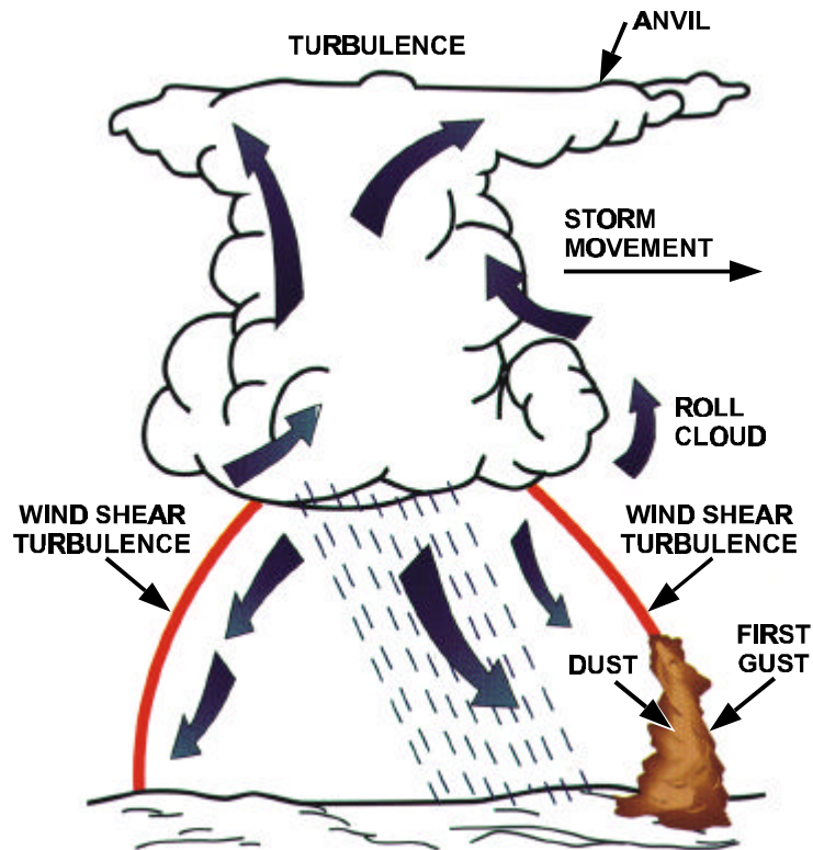
Figure 6.5-1. Storm Components
