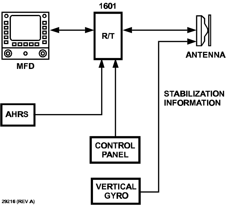
Figure 2-1. Typical System Block Diagram
