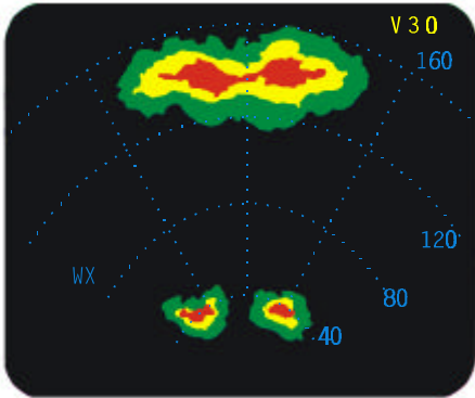
Figure 6.5.8-1. Azimuth Resolution
