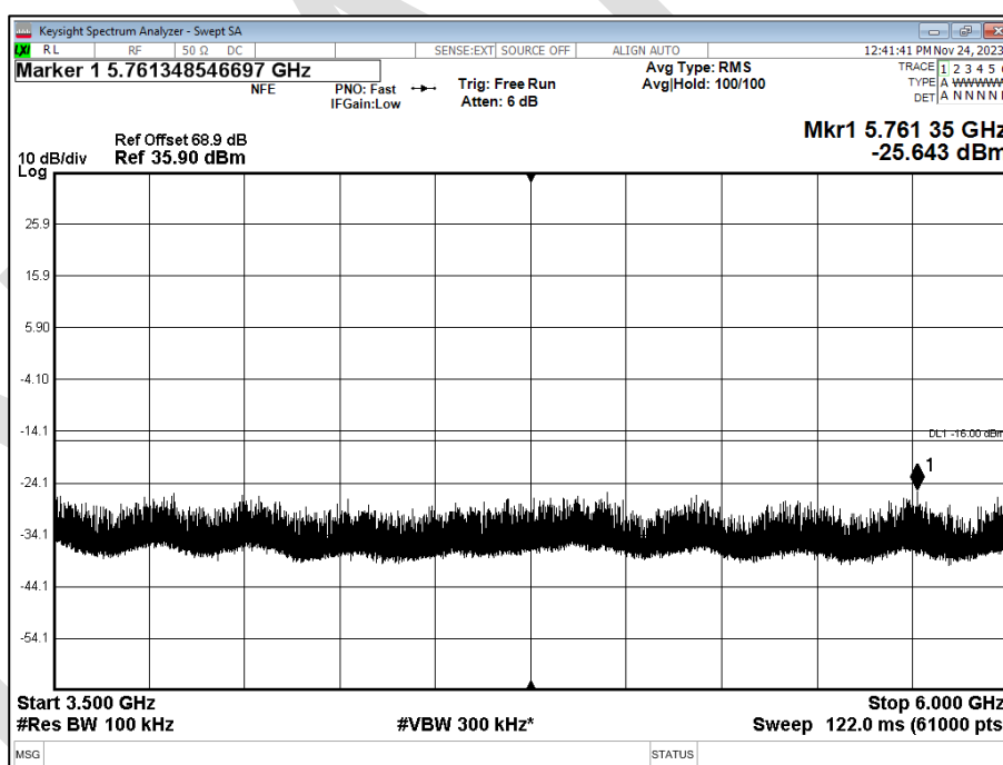
Figure 30 - 850 MHz, 64QAM, 3.5 GHz to 6 GHz, Sector A (TxRx0)
