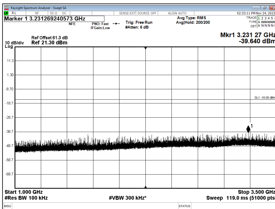
Figure 33 - 850 MHz, QPSK, 1 GHz to 3.5 GHz, Sector A (TxRx1)
