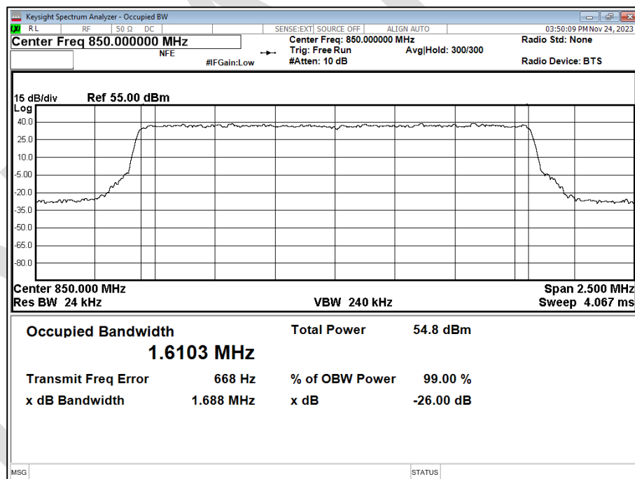
Figure 6 - 850 MHz, 64QAM
