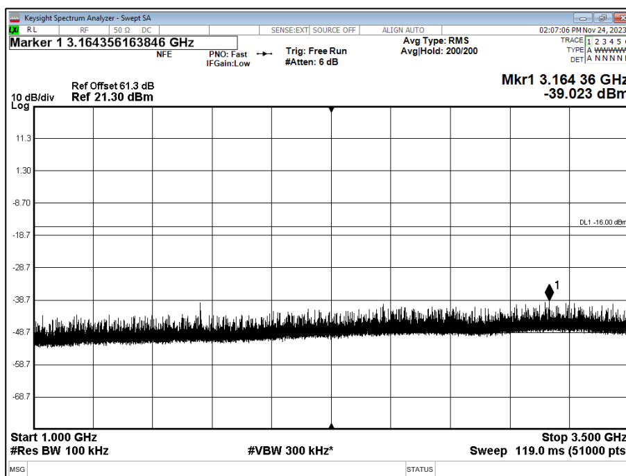
Figure 21 - 850 MHz, QPSK, 1 GHz to 3.5 GHz, Sector A (TxRx0)
