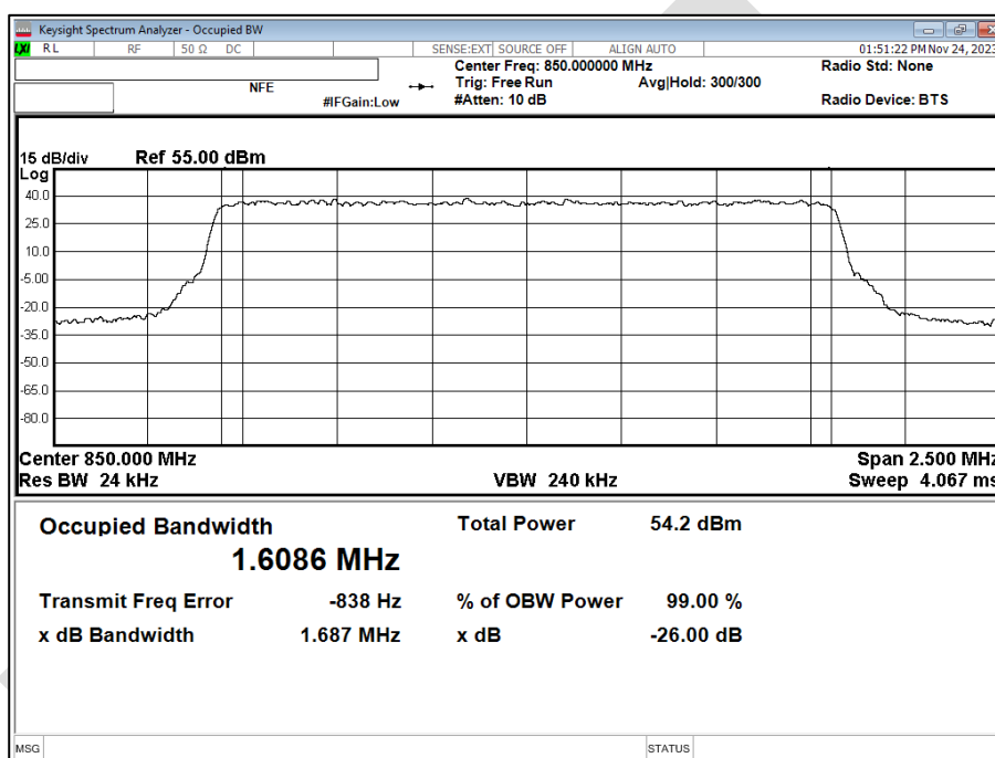
Figure 4 - 850 MHz, QPSK
