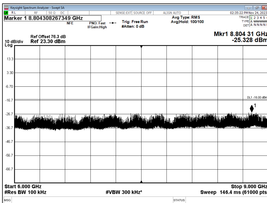
Figure 35 - 850 MHz, QPSK, 6 GHz to 9 GHz, Sector A (TxRx1)
