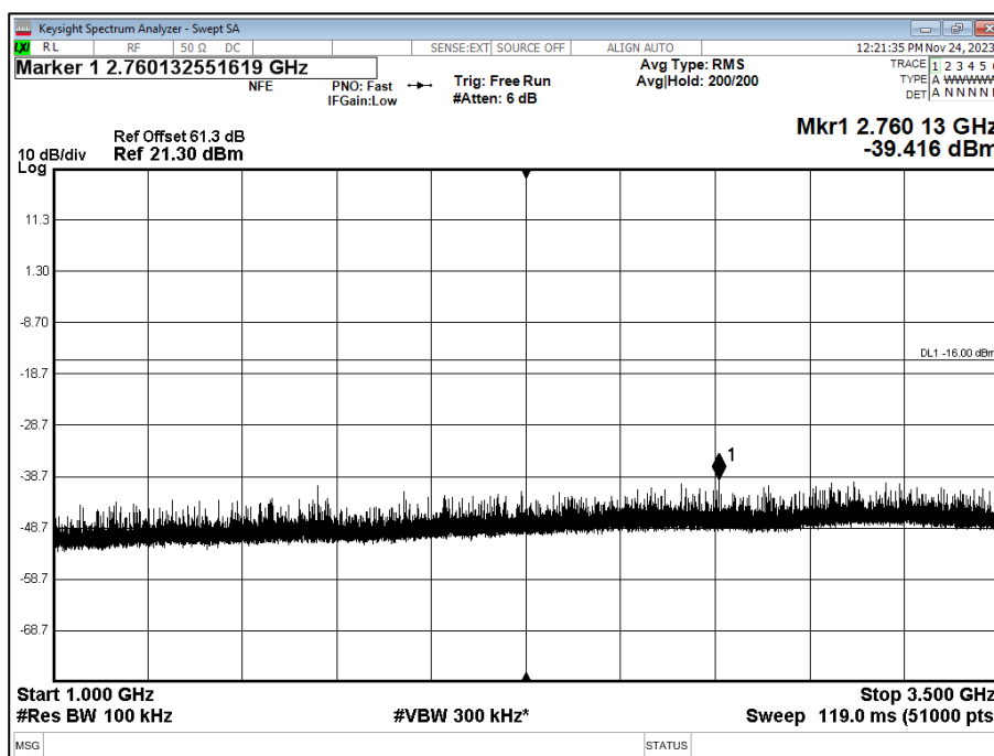
Figure 29 - 850 MHz, 64QAM, 1 GHz to 3.5 GHz, Sector A (TxRx0)
