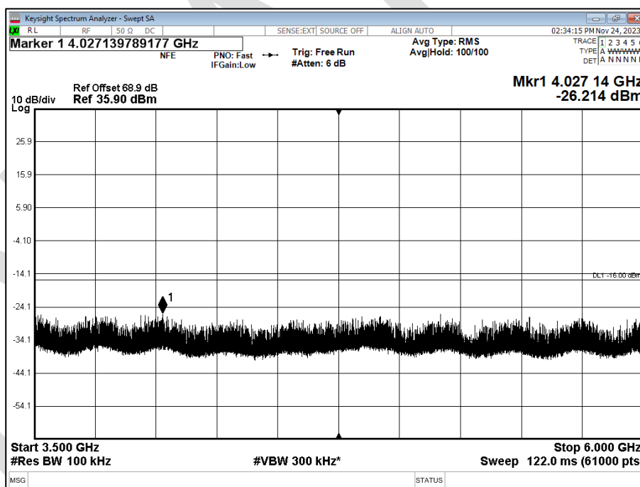
Figure 34 - 850 MHz, QPSK, 3.5 GHz to 6 GHz, Sector A (TxRx1)
