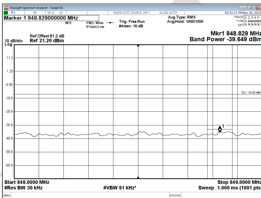
Figure 14 - 850 MHz, QPSK, Band Edge Frequency: 849 MHz. Sector A (TxRx1)
