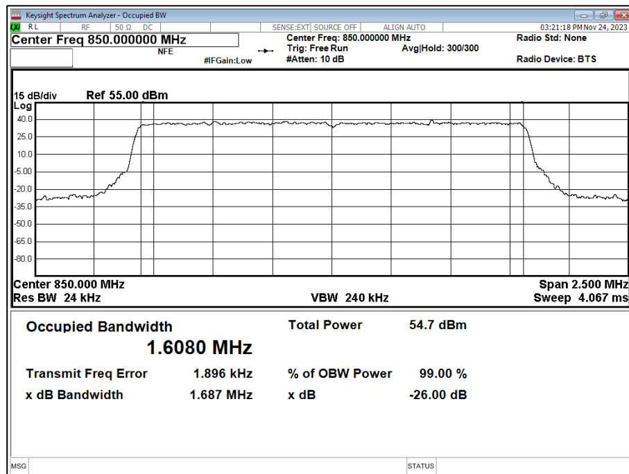
Figure 5 - 850 MHz, 16QAM
