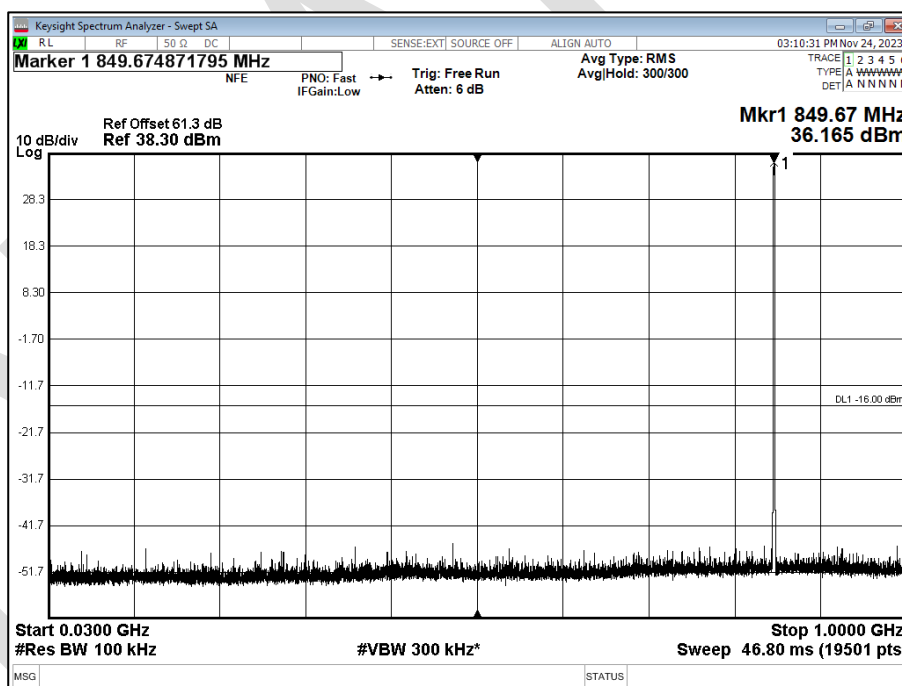
Figure 36 - 850 MHz, 16QAM, 30 MHz to 1 GHz, Sector A (TxRx1)
