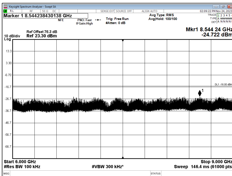
Figure 23 - 850 MHz, QPSK, 6 GHz to 9 GHz, Sector A (TxRx0)
