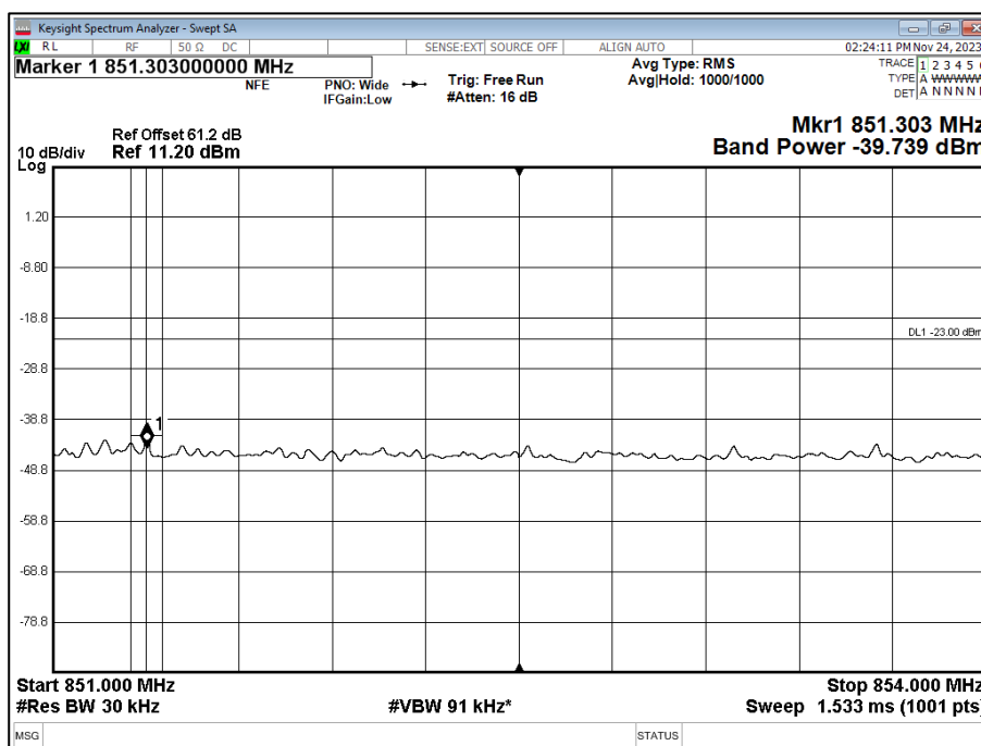
Figure 15 - 850 MHz, QPSK, Band Edge Frequency: 851 MHz. Sector A (TxRx1)
