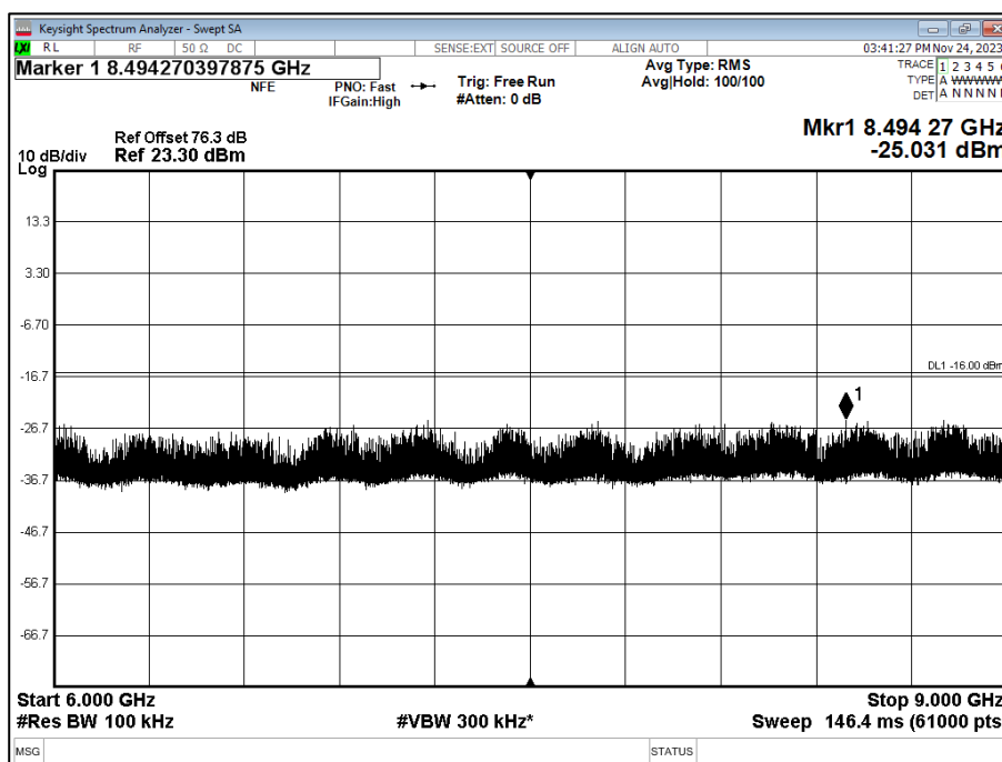
Figure 27 - 850 MHz, 16QAM, 6 GHz to 9 GHz, Sector A (TxRx0)
