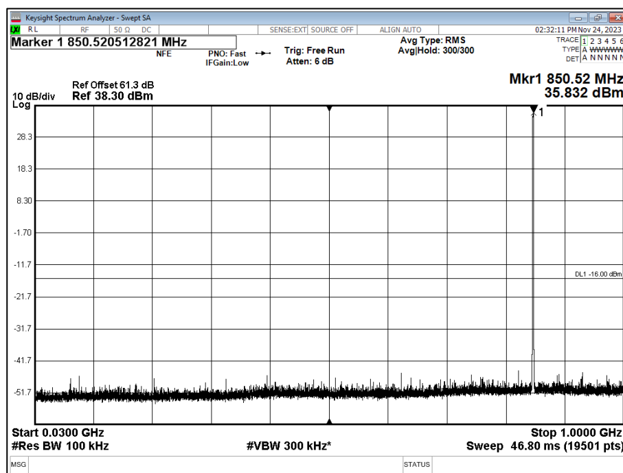
Figure 32 - 850 MHz, QPSK, 30 MHz to 1 GHz, Sector A (TxRx1)
