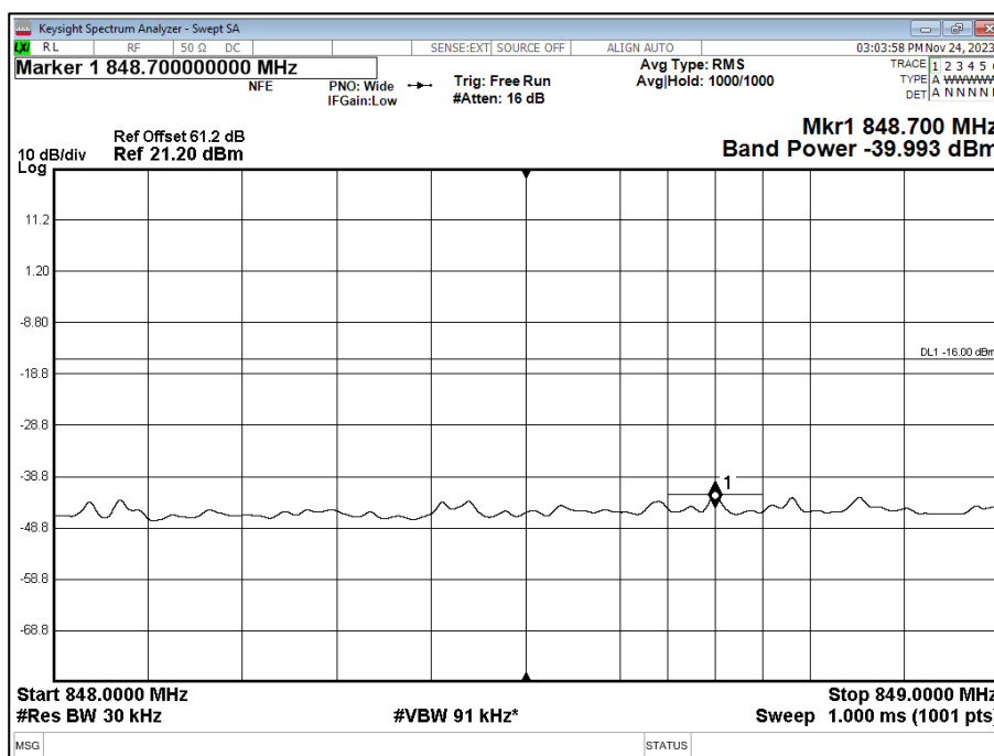
Figure 16 - 850 MHz, 16QAM, Band Edge Frequency: 849 MHz. Sector A (TxRx1)
