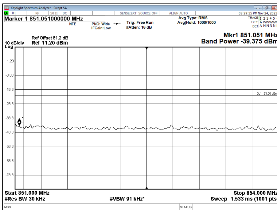
Figure 11 - 850 MHz, 16QAM, Band Edge Frequency: 851 MHz. Sector A (TxRx0)
