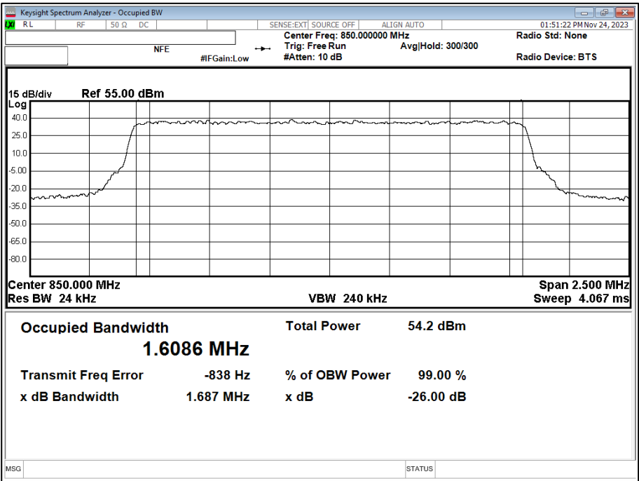
Figure 4 - 850 MHz, QPSK
