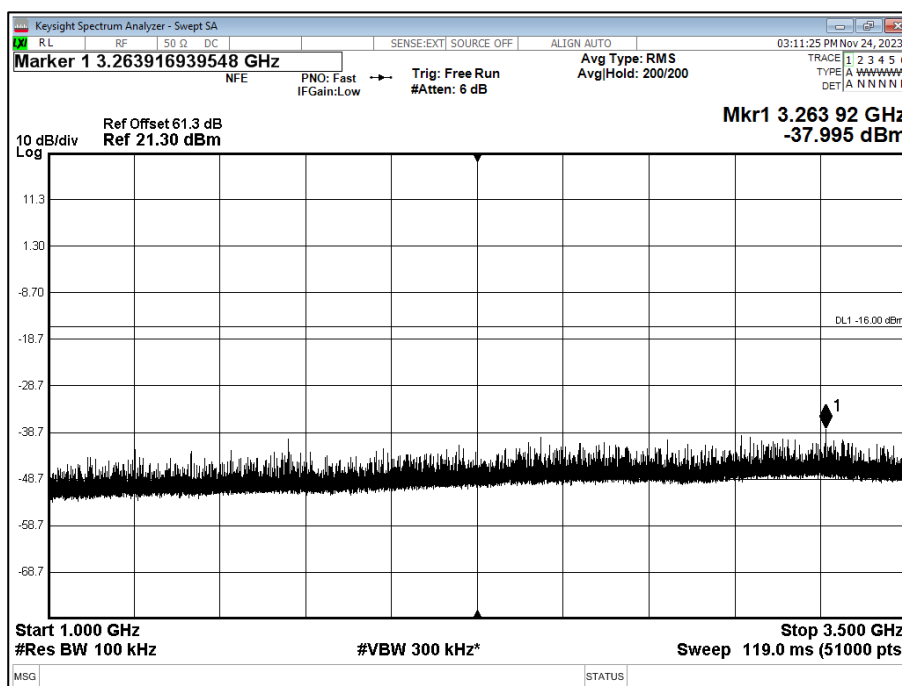
Figure 37 - 850 MHz, 16QAM, 1 GHz to 3.5 GHz, Sector A (TxRx1)
