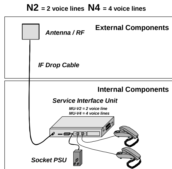
Figure 20. N Series Demand Assigned Subscriber Terminals
