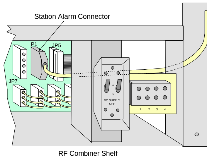
Figure 13. Station Alarm Connection
