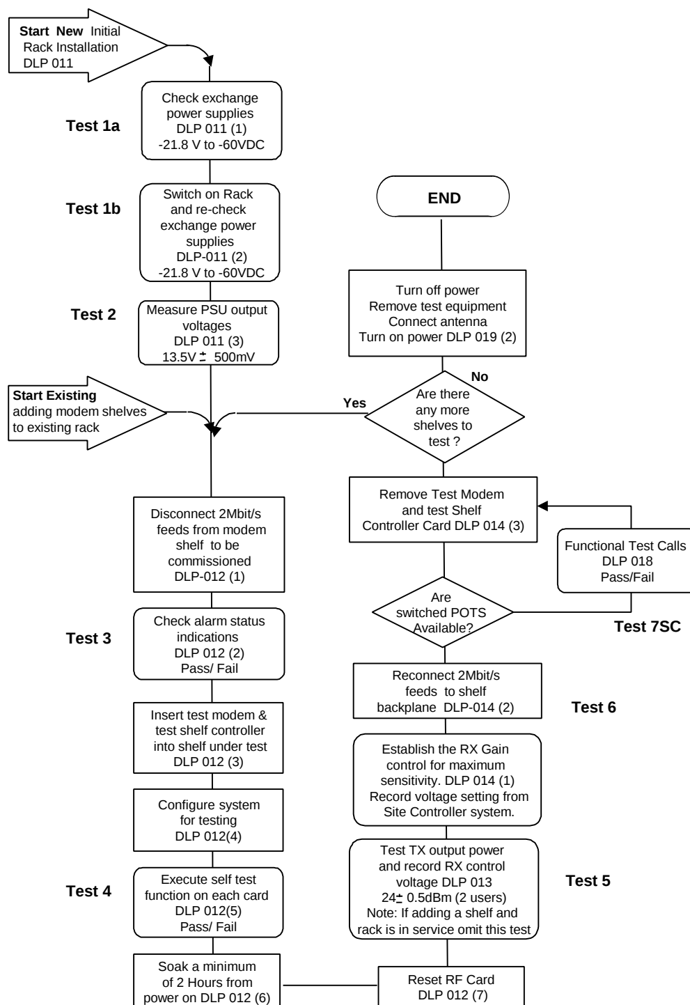
Chart 6. Commissioning ALL-Bands connecting to Sitespan using Level Control Unit.
