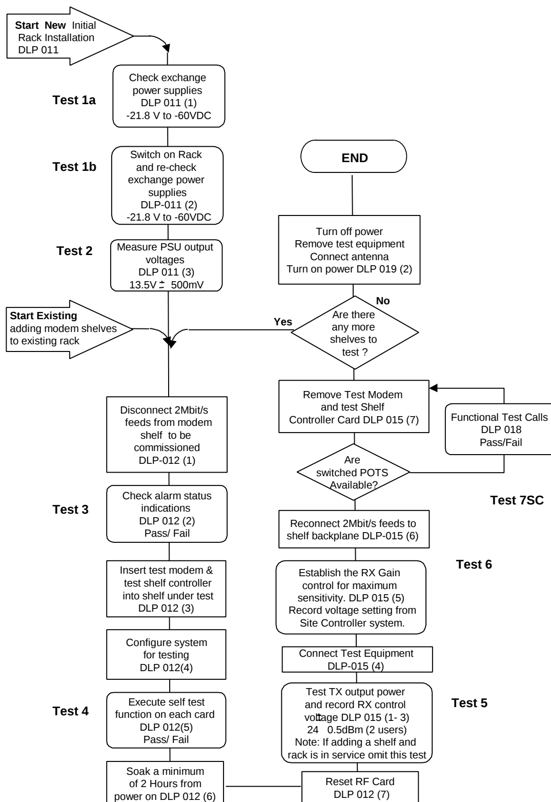
Chart 3. Commissioning 2.0-2.3GHz Band connecting to Sitespan using Test CRU.
