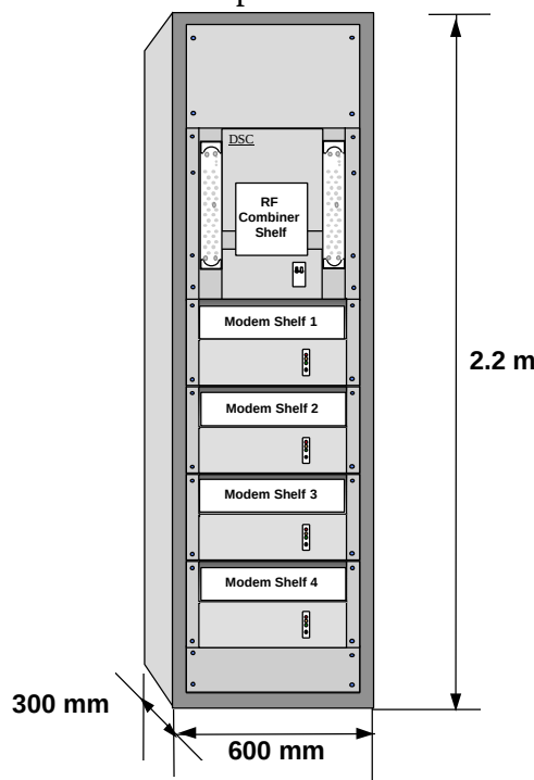
Figure 2. Central Terminal Rack.
