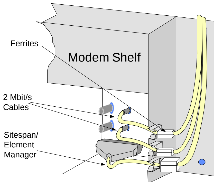
Figure 15. Rack Cabling
