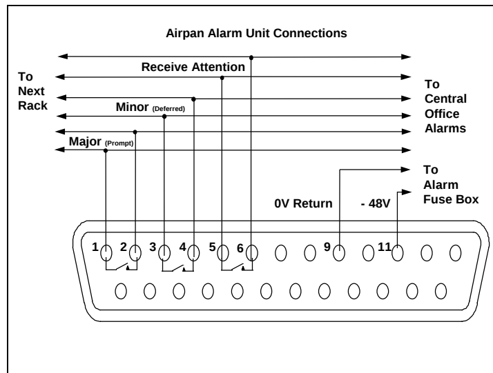
Figure 12. AS4000 Alarm Unit Connections
