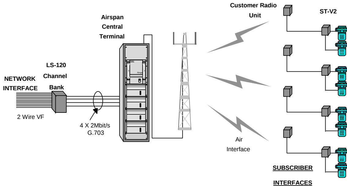
Figure 48. AS4000 using LS120 as a Channel Bank
