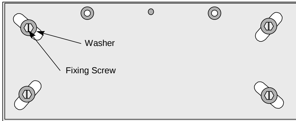
Rack Base
