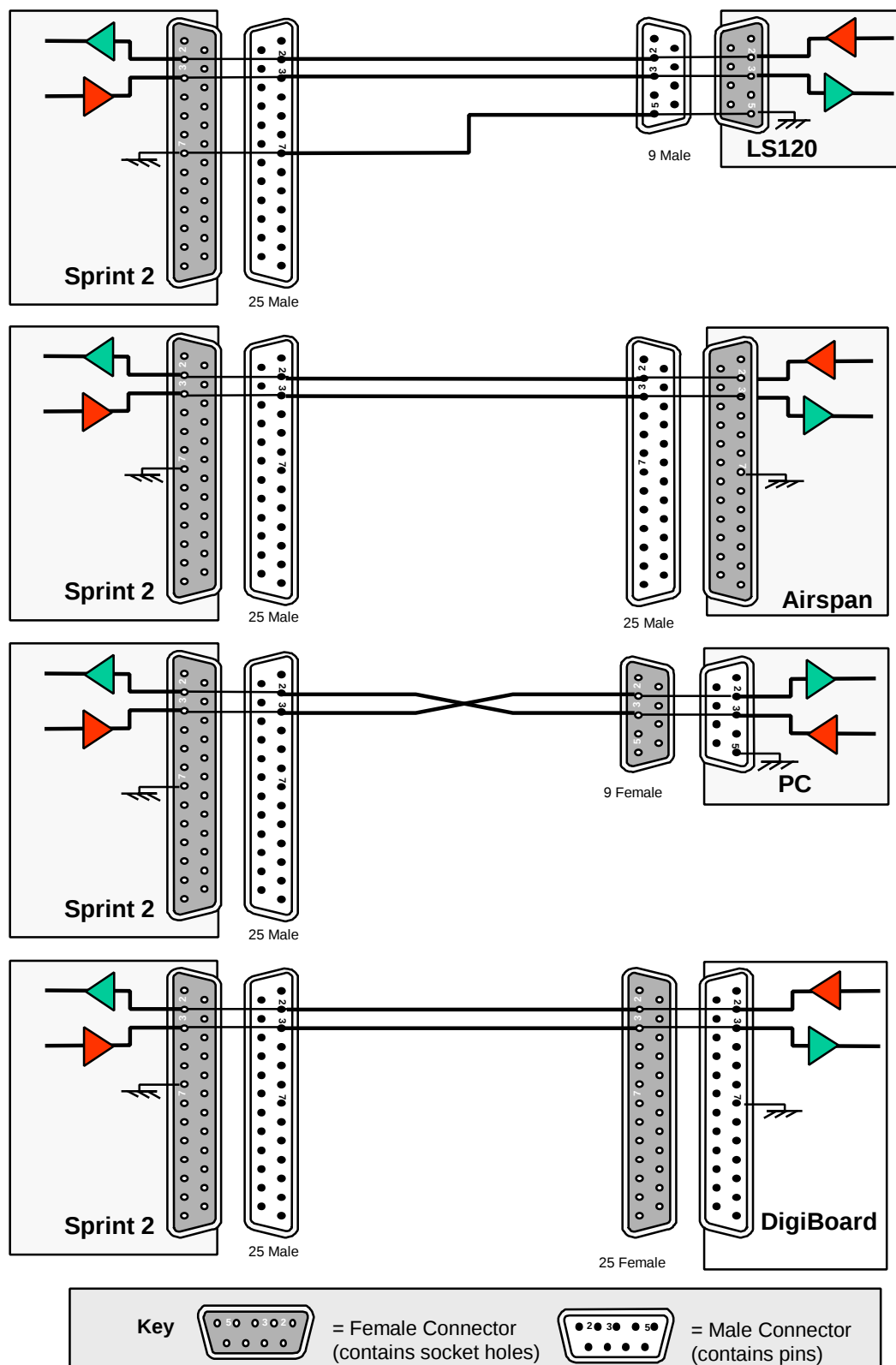
Figure 25. D-Type Wiring Details (2)
