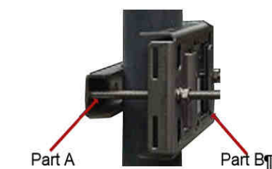
Figure 6: Mounting Bracket
