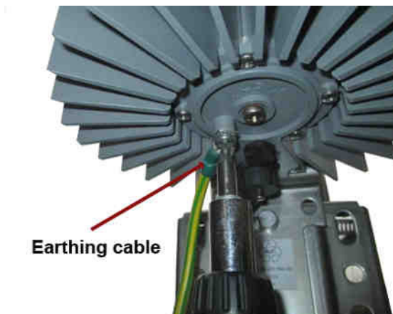
Figure 16: iR460 with Earthing Connection
