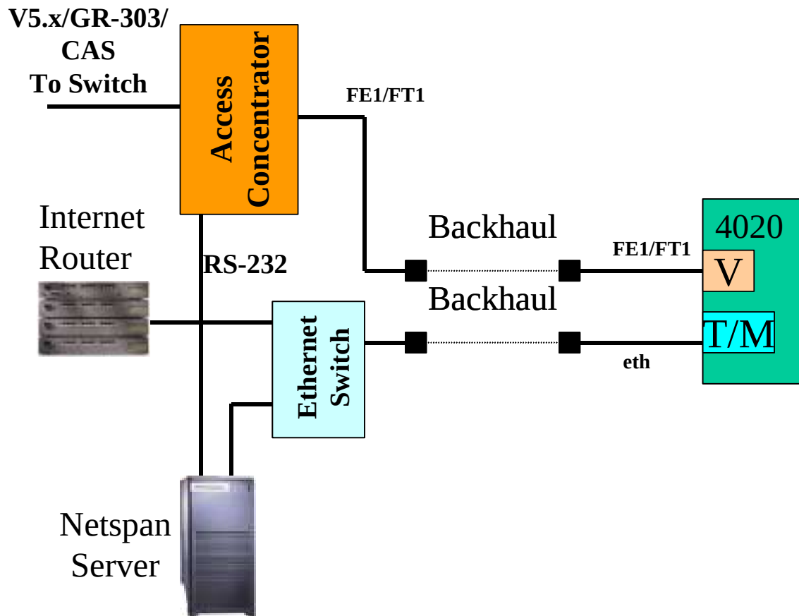
Figure 7 - AS4020 Backhaul Connections
