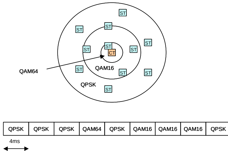
Figure 6 AS4020 per ST Modulation & FEC Adaption
