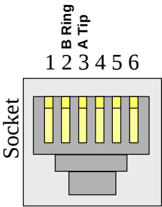
Figure 37. RJ11 Phone port
