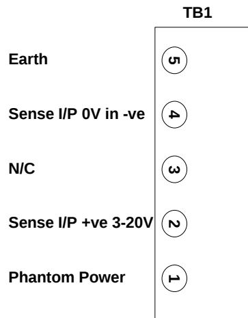
Figure 56. Alarm Connections
