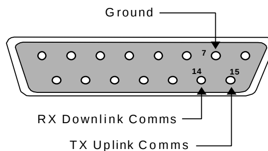
Figure 64. B, L, N, and M series 15 way D-type STMON connections
