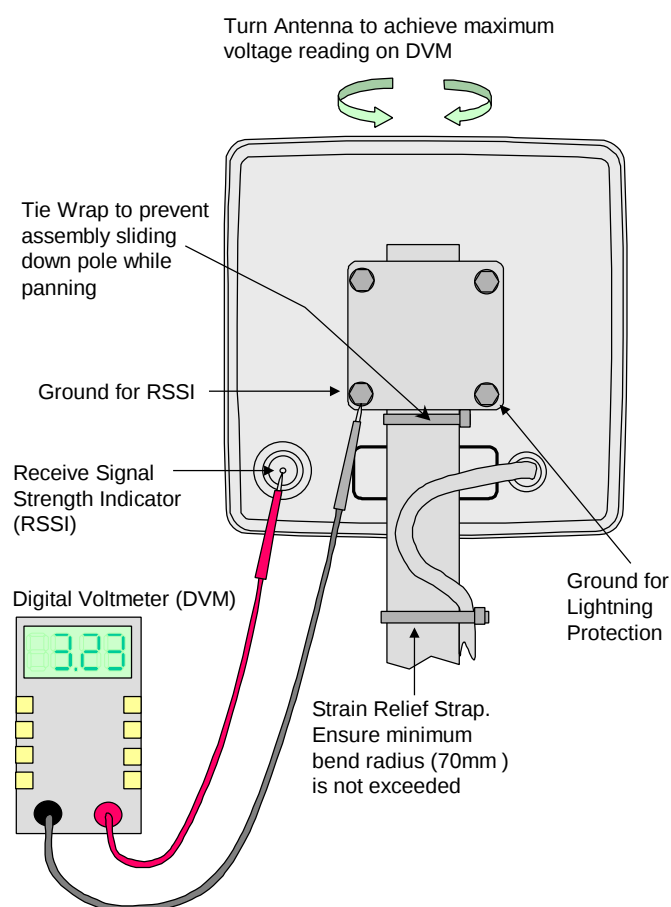
Figure 65. Panning Pole Mount Antenna
