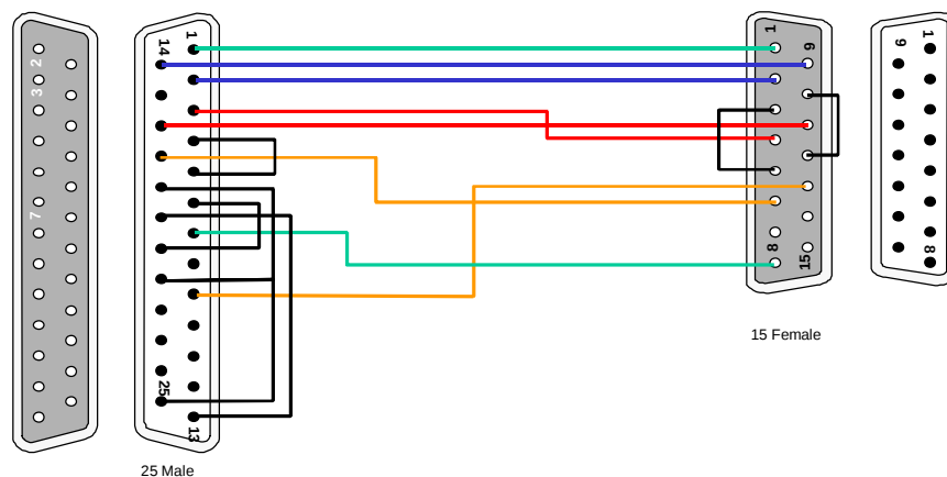
Figure 50. Interconnection of EIA-530 and X21
