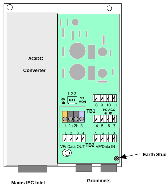
Figure 16. Type 4A Power Supply Unit.
