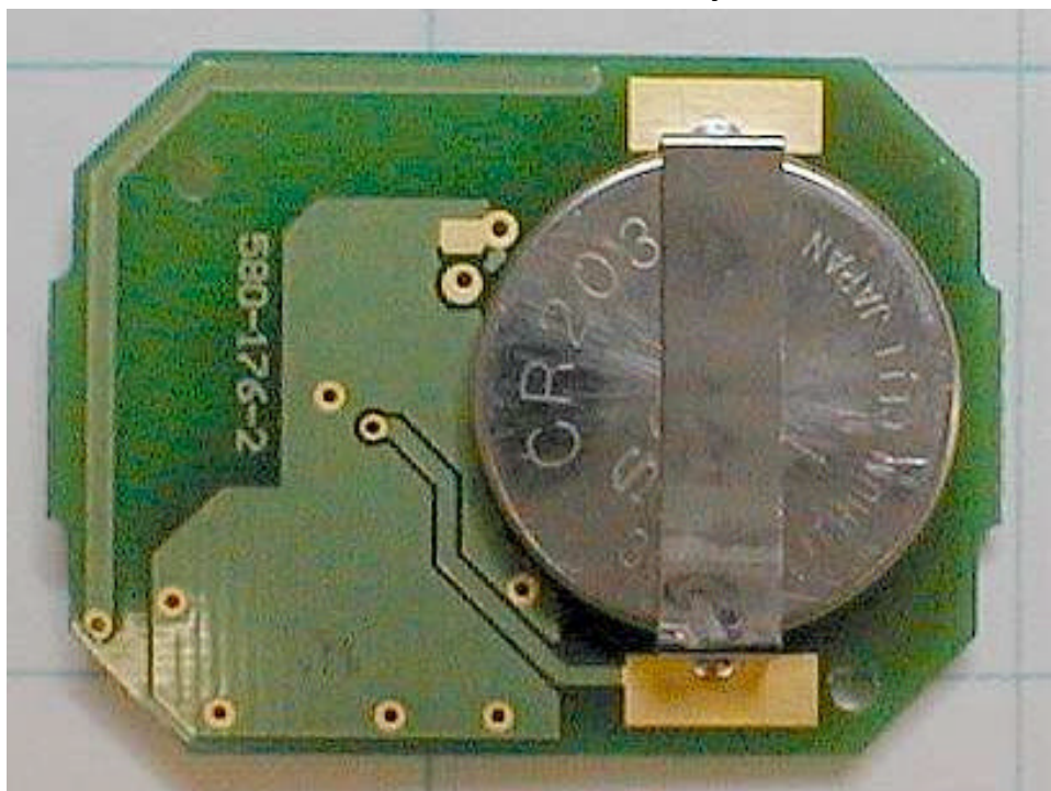
PCB Bottom with Battery
