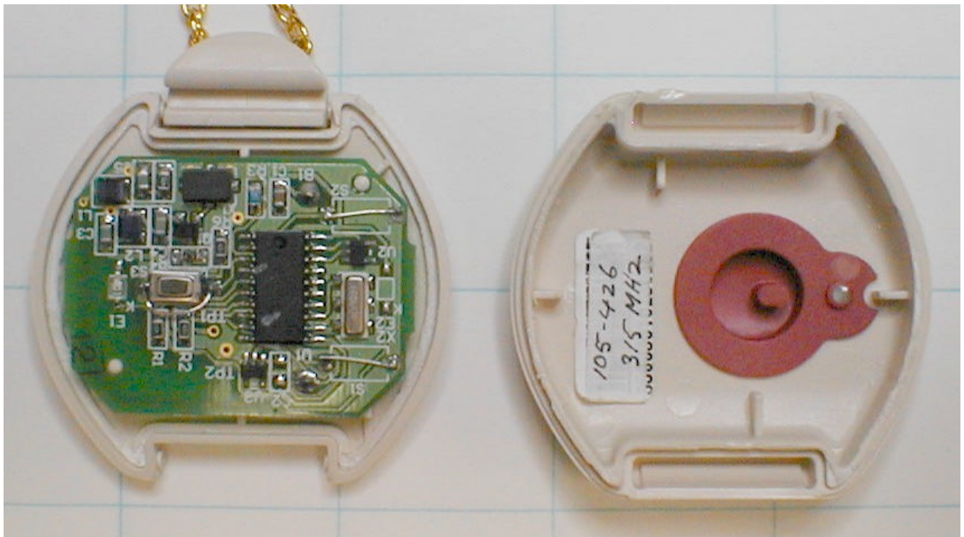
Cover Open
