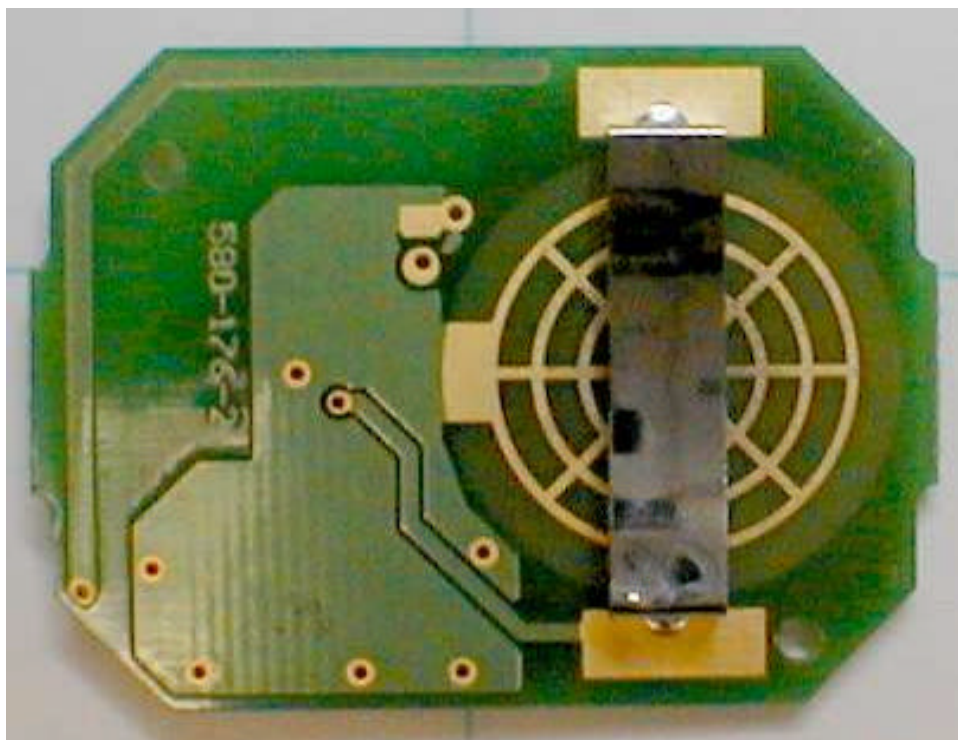
PCB Bottom without Battery
