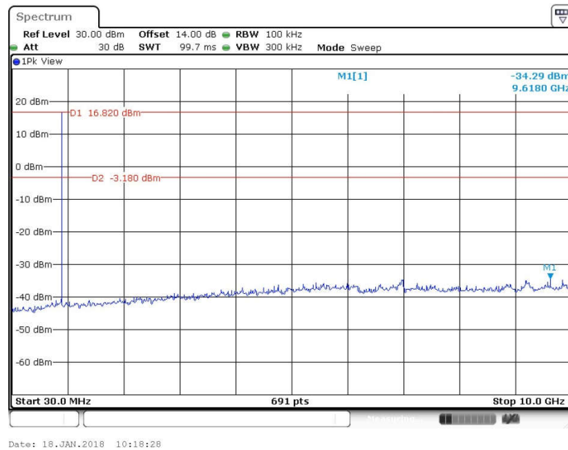
CSE Plot on Ch 12 between 30MHz ~ 10 GHz
