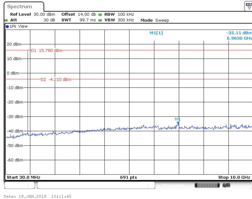
CSE Plot on Ch 24 between 30MHz ~ 10 GHz
