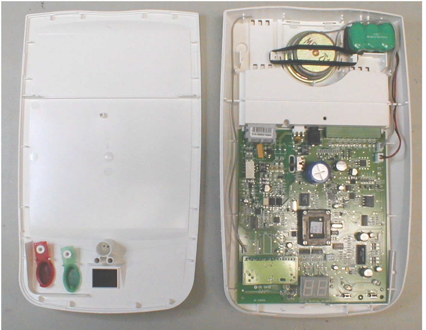
Cover Removed
