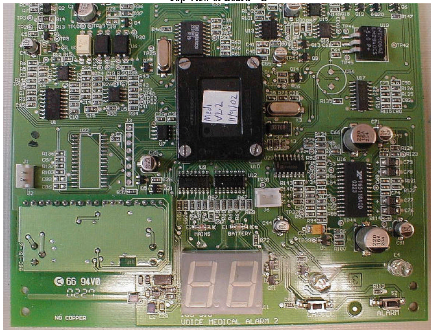
Top View of Board - B
