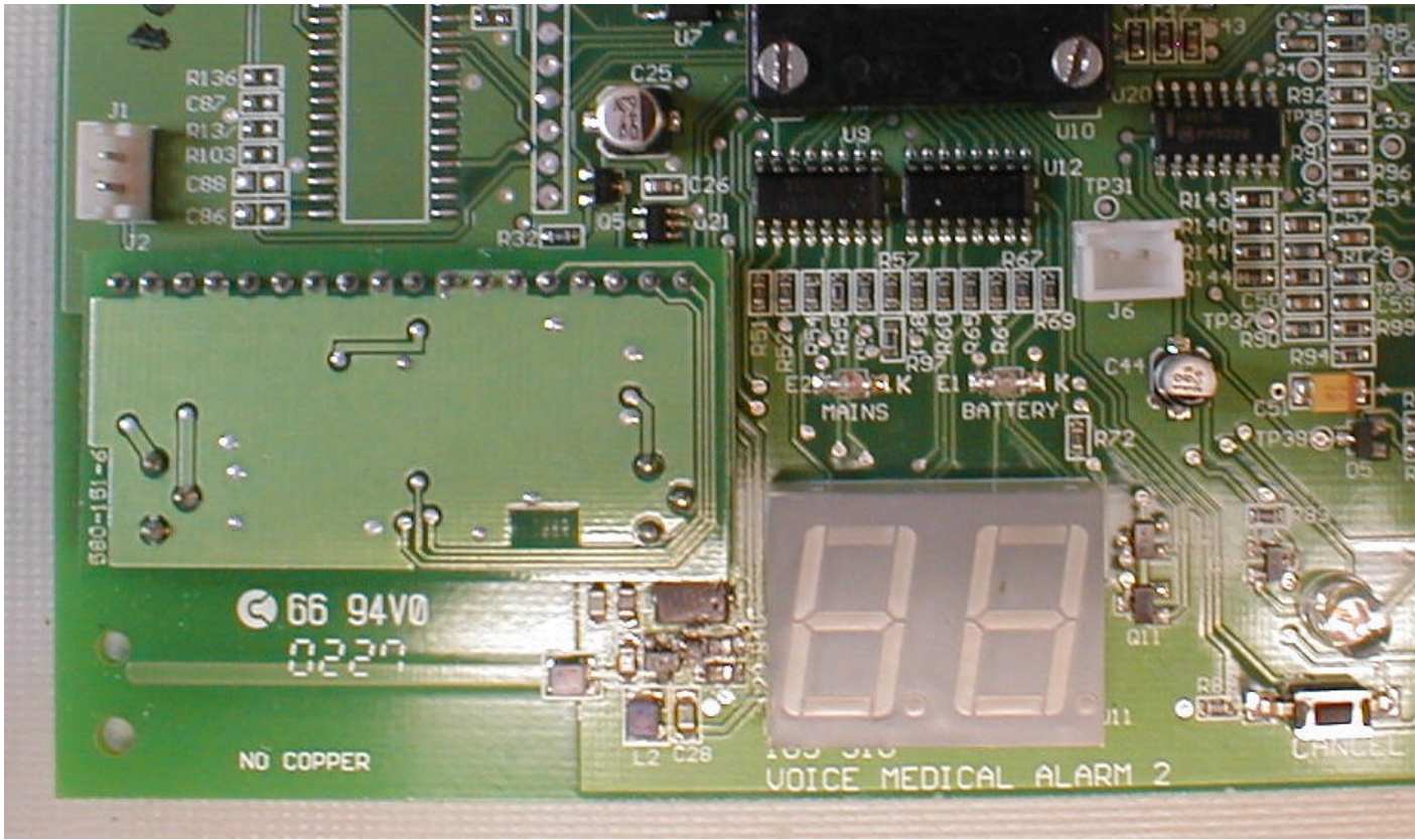
Detail of Small Board – Bottom View
