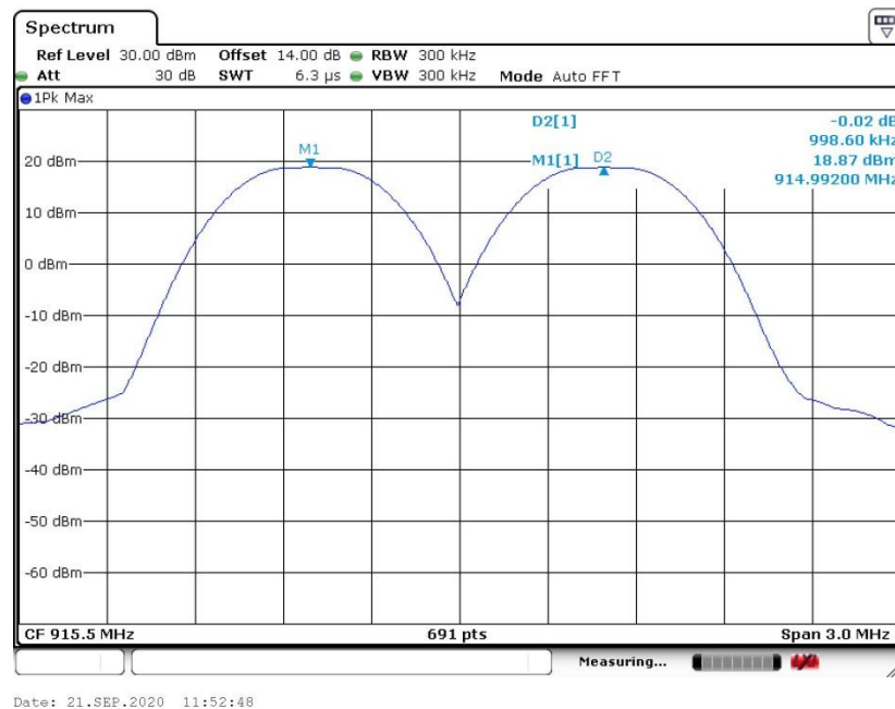
Channel Separation Plot on Channel 12 - 13
