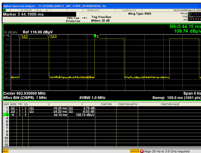
903MHz: on time (Count Pulses) Plot on Channel 00
