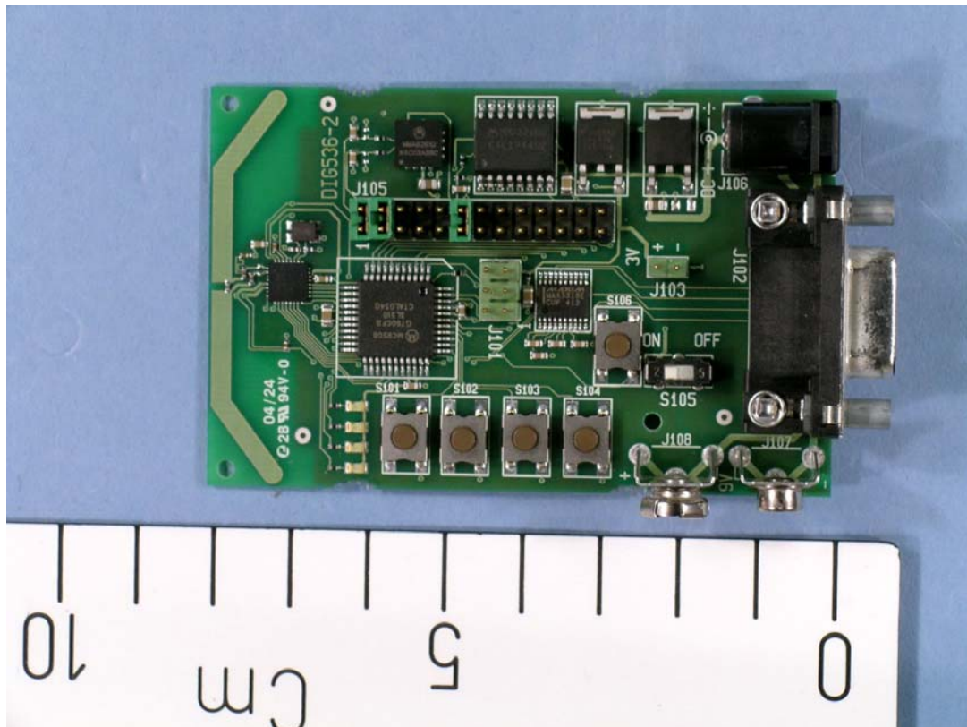
13192-SARD with integrated antenna, top view
