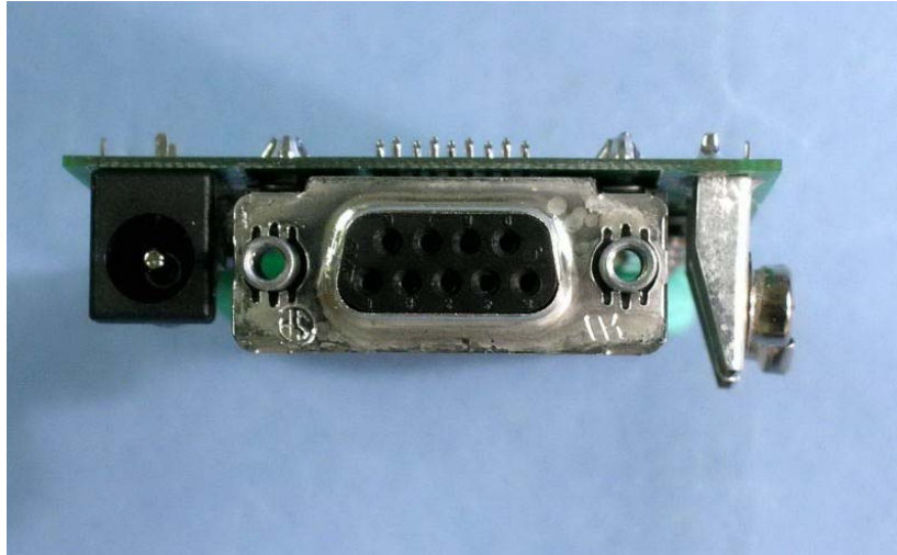
13192-SARD with integrated antenna, view of RS 232 port , AC adapter and DC battery ports
