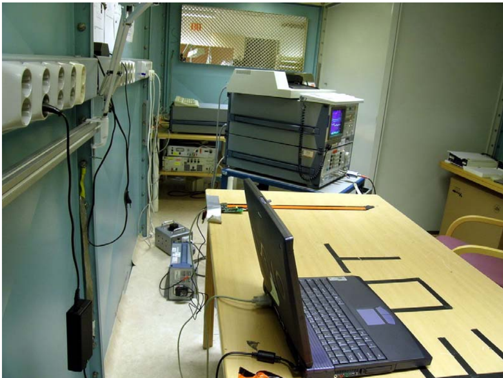
Test setup, Conducted emissions
