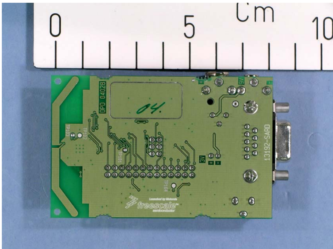
13192-SARD with integrated antenna, rear view
