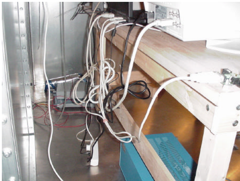
Picture 6 : Setup for conducted emission test on the AC mains (rear view)
