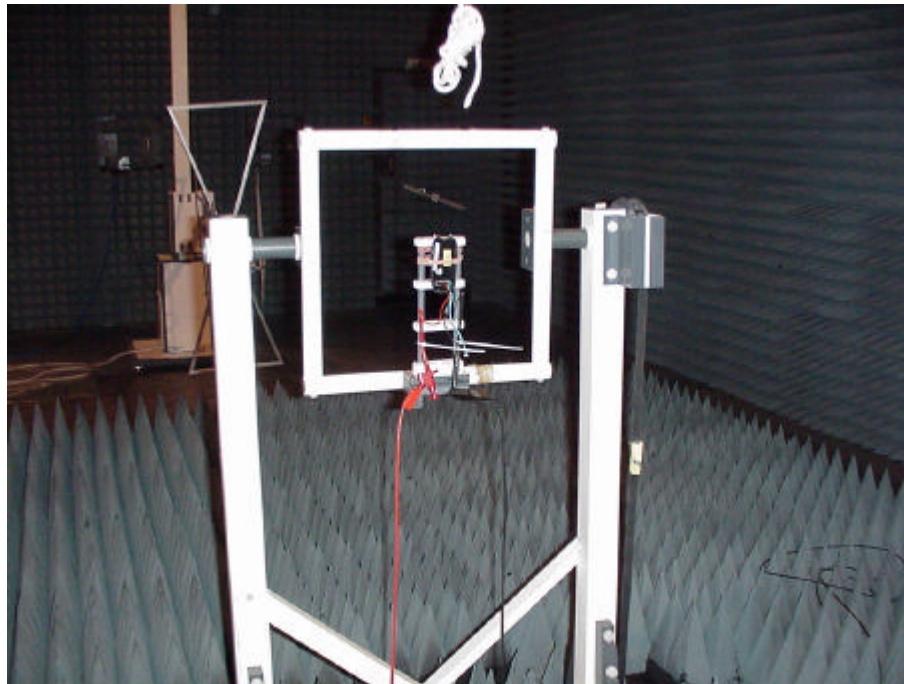
Picture 3 : Setup for radiated tests
