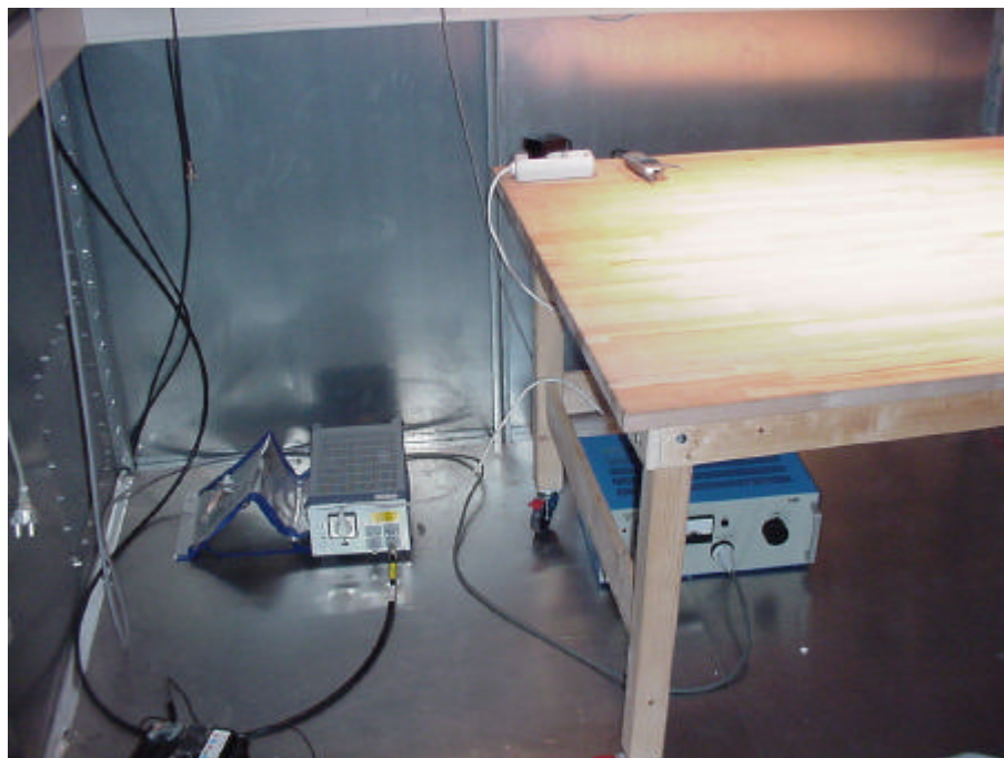
Picture 4 : Setup for conducted emission test on the AC mains
