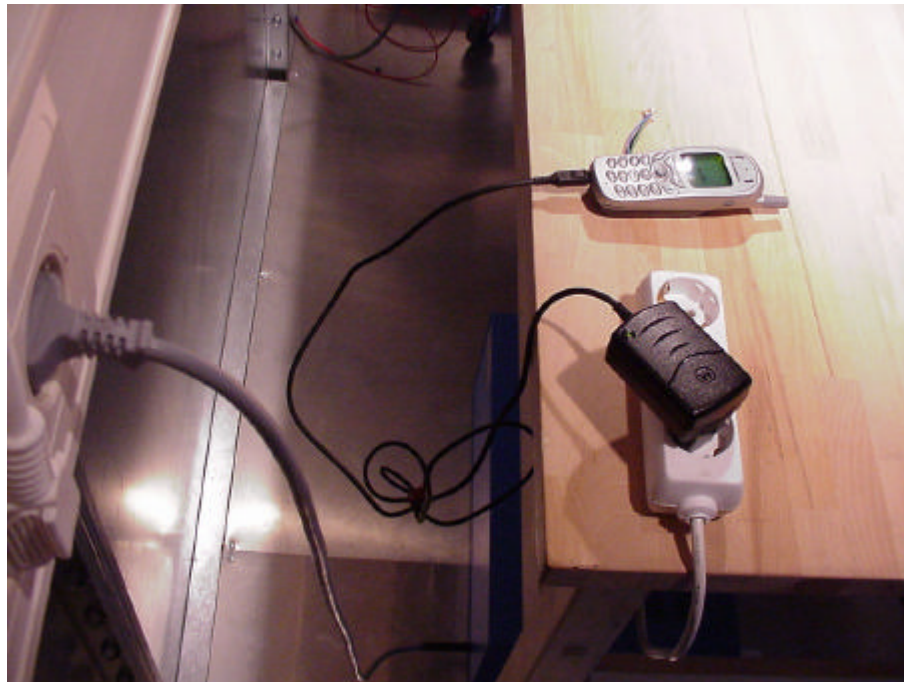
Picture 5 : Setup for conducted emission test on the AC mains (rear view) EUT connected to the Motorola mobile phone.
