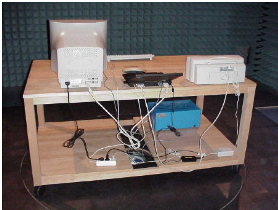
Picture 2 : Setup for radiated measurement, rear view
