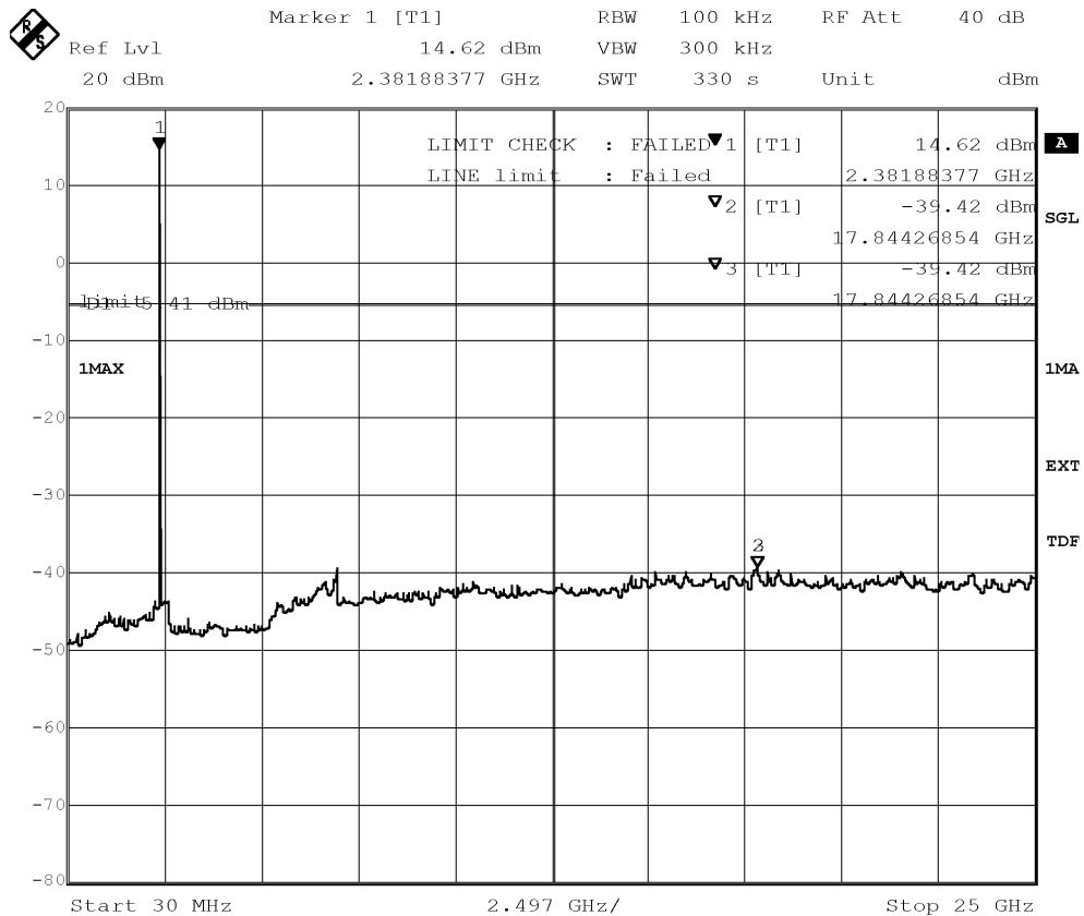
Spurious RF Conducted Emissions
