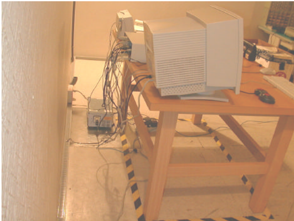
Back View of Conducted Emission (Mode 1)
