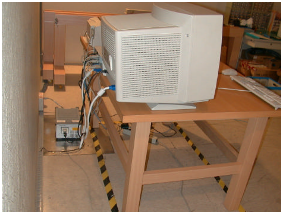
Back View of Conducted Emission
