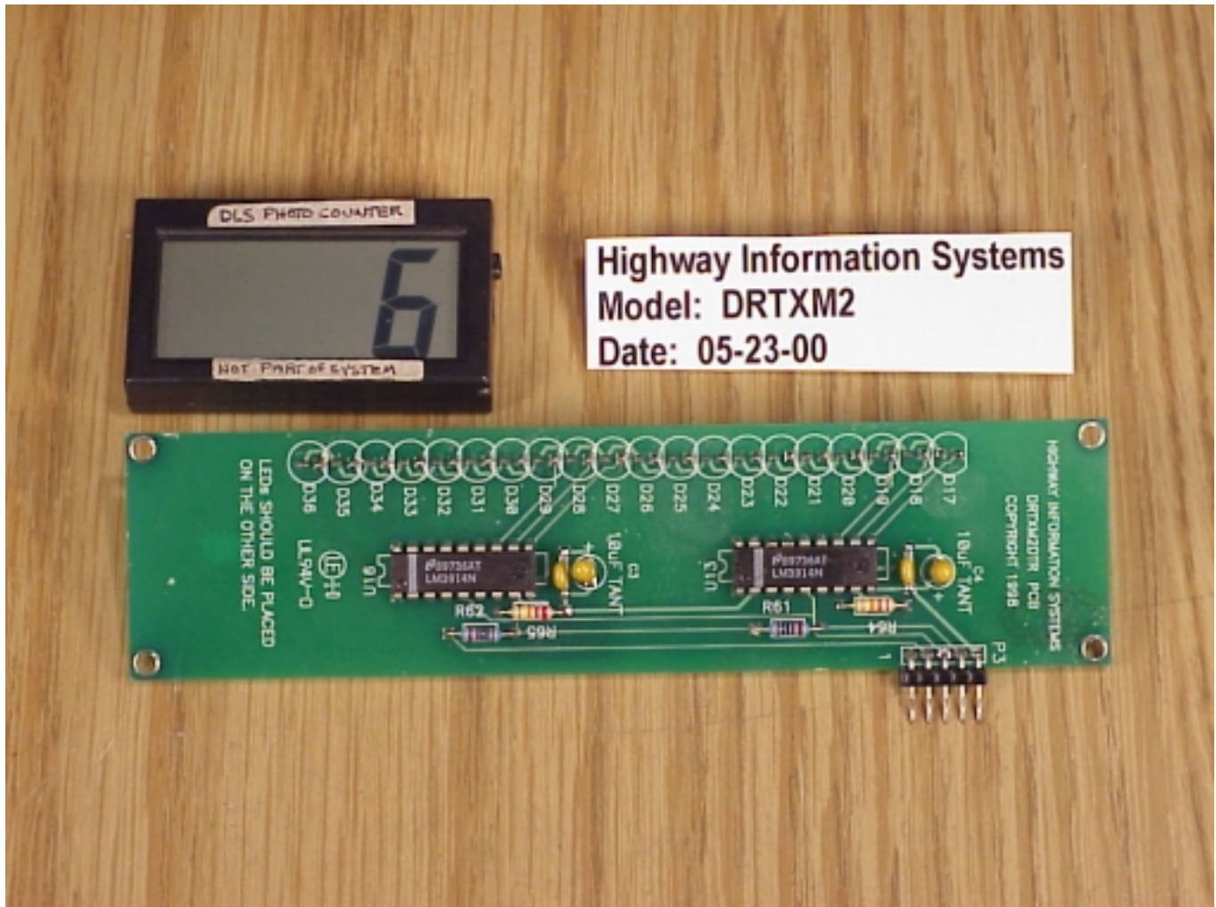
Component Side of DRTXM2DTR Board
