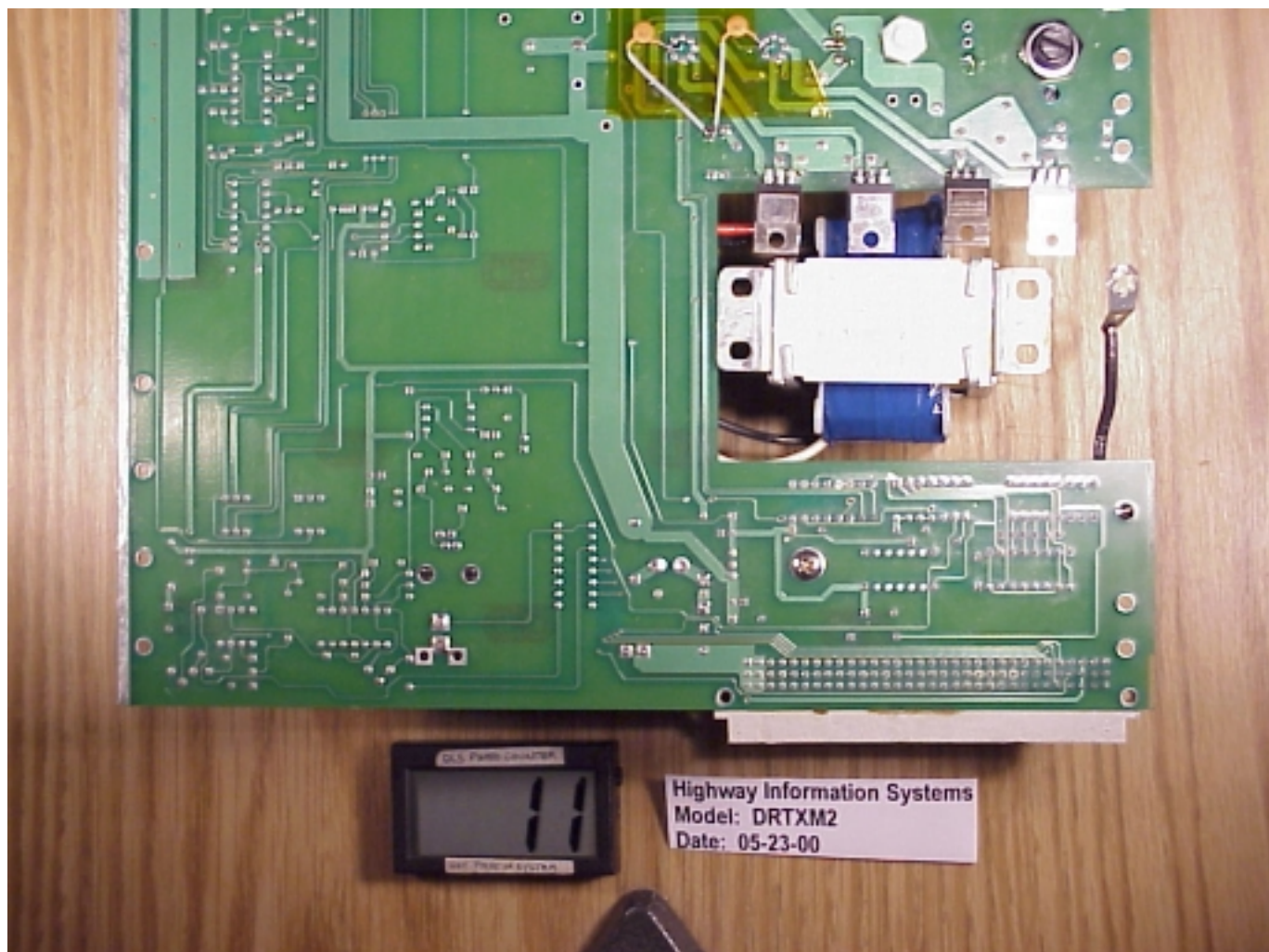
Back Half DRTXM2DTR Main Board Solder Side
