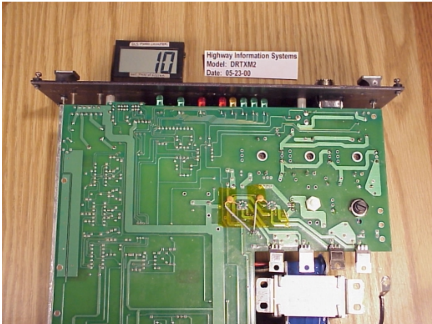
Front Half of DRTXM2DTR Main Board Solder Side
