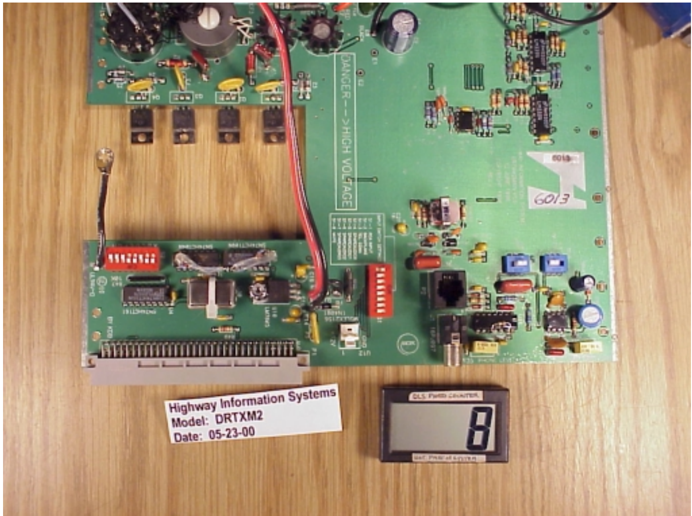
Back Half of DRTXM2DTR Main Board Component Side
