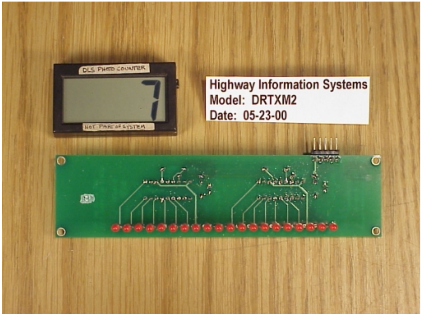
Solder?LED Side of DRTXM2DTR Board
