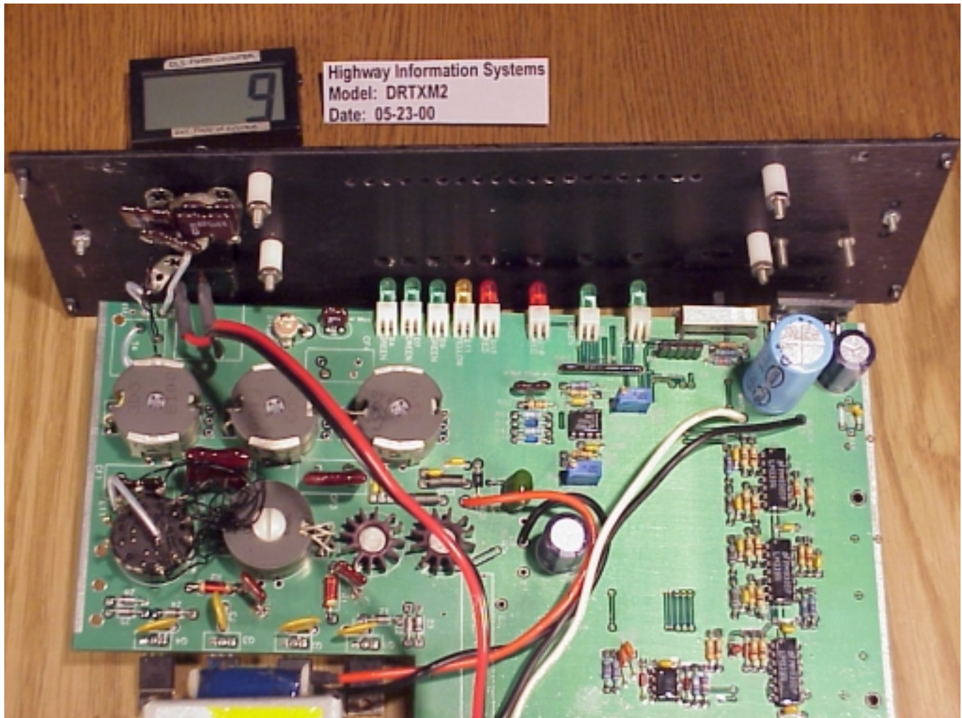
Front Half of DRTXM2DTR Main Board Component Side
