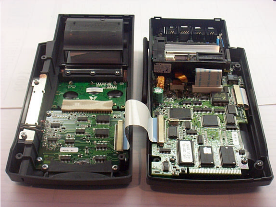
Lipman USA, Ltd. Nurit 3010 CDPD: Open
