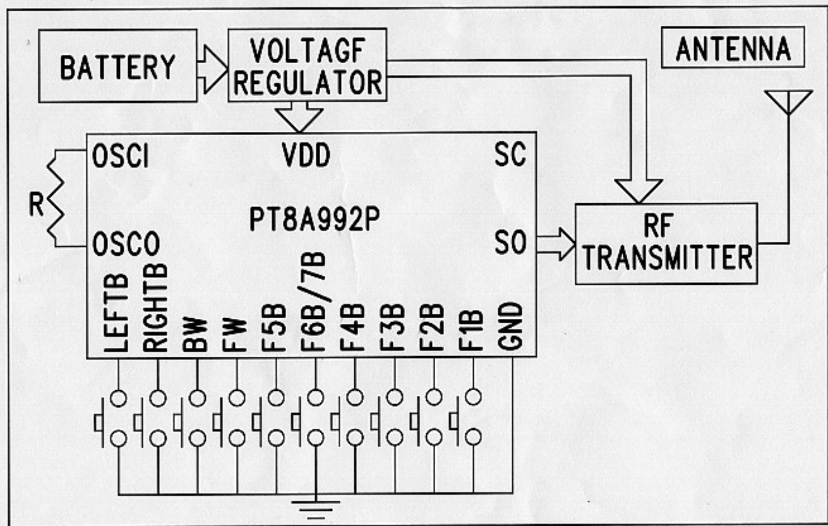
BLOCK DIAGRAM OF THE TRANSMITTER CIRCUIT USING PT8A992P
