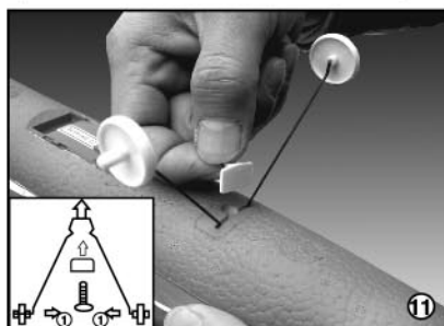
11. Hold the plastic sheet into the slot and fix it with the \phi 2.0 \times 6 PB screw.(Fig.11)
