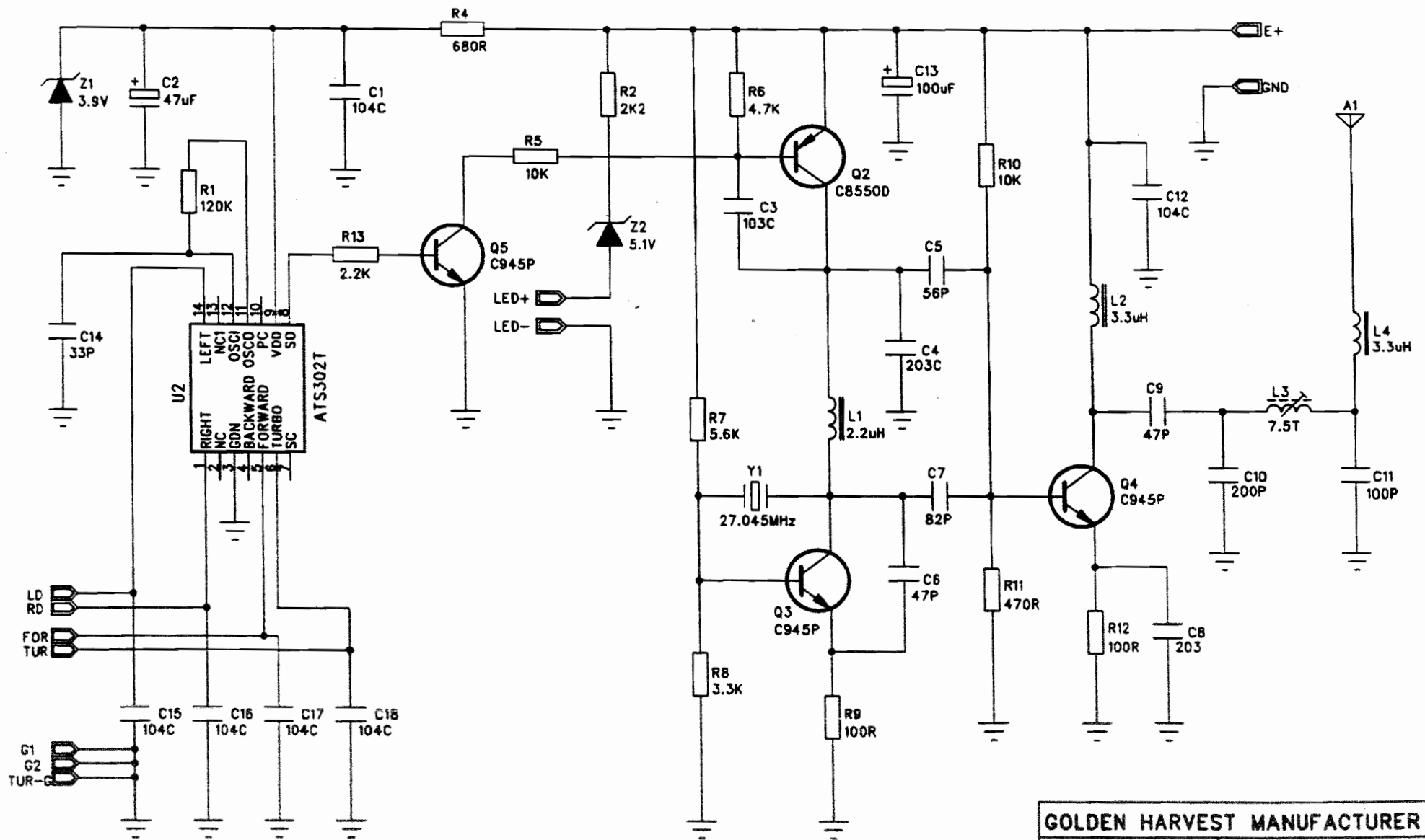
9806/ 9807 TX BLOCK DIAGRAM OF APPLICATION CIRCUIT
