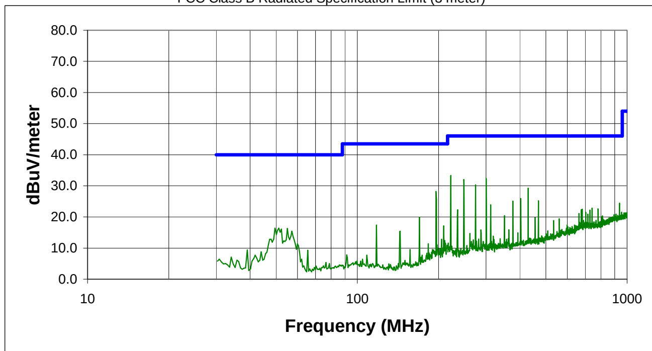
FCC Class B Radiated Specification Limit (3 meter)
