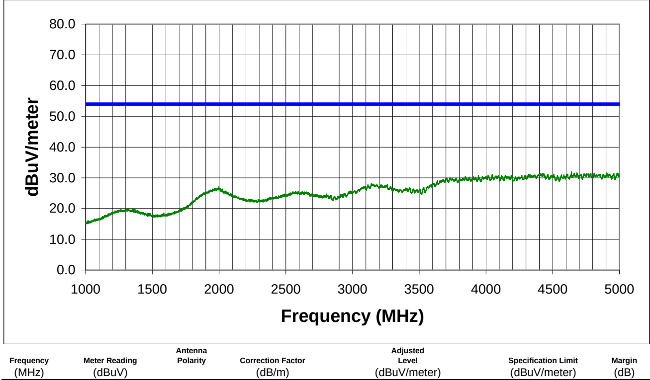
FCC Class B Radiated Specification Limit (3 meter)
