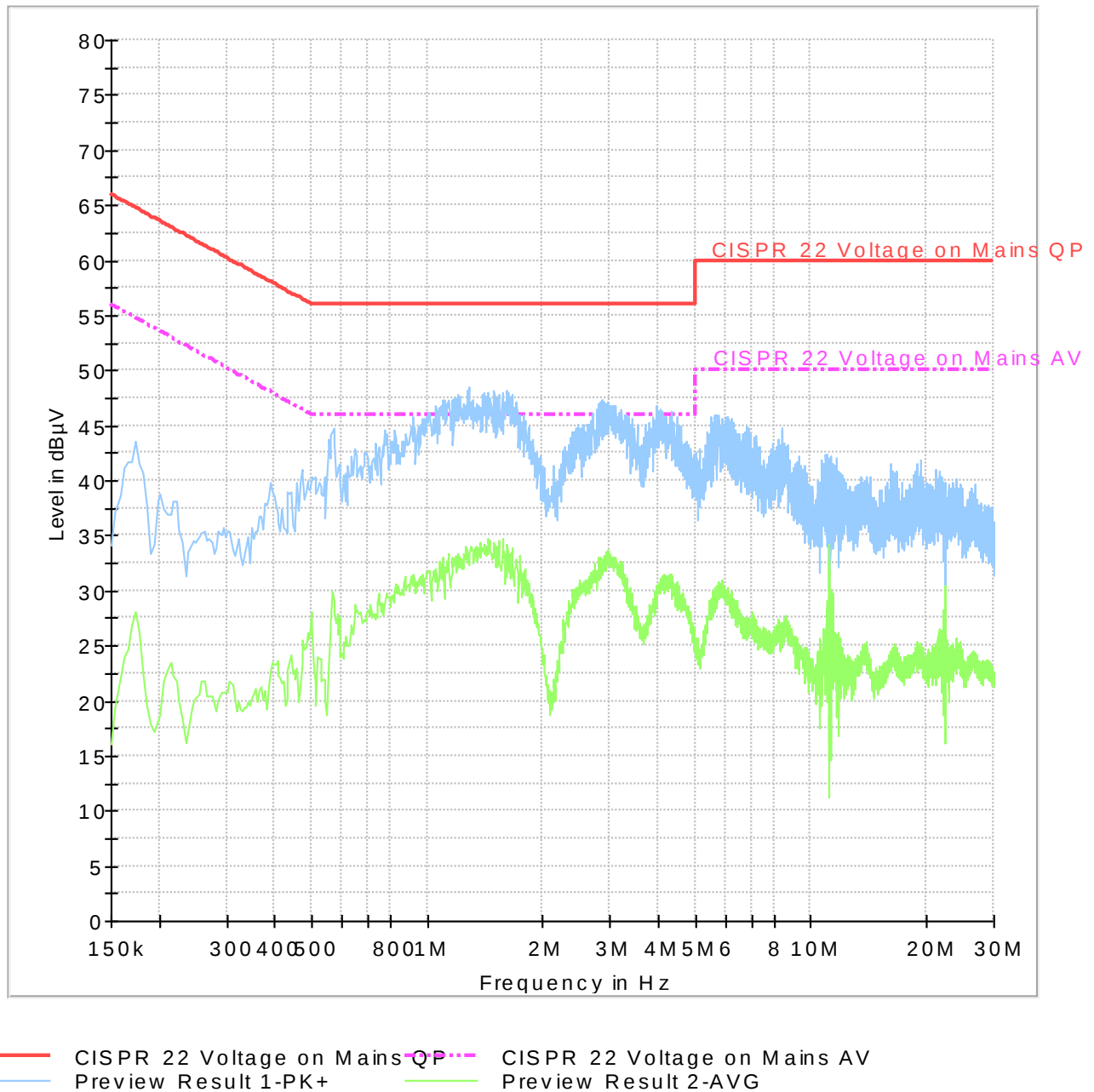
CISPR 22 Conducted Emissions
