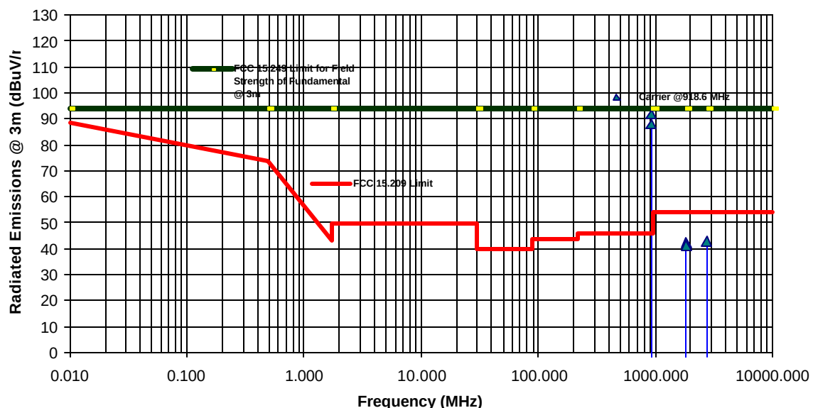
Transmitter Radiated Emissions Measurements at 3 Meters OFTS TRANSMIT Freq.: 918.6MHz IVI Checkmate Inc. Elite 770 Intelligent Base, Model Elite 770 Intelligent Base
