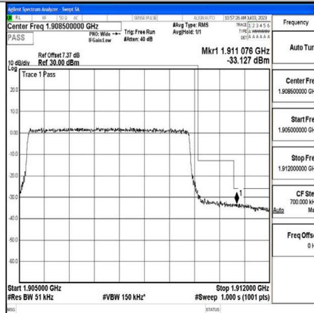
Band2_5MHz_16QAM_19175_25RB#0
