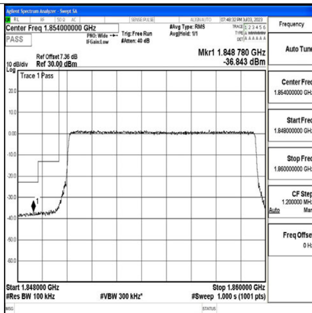
Band2_10MHz_QPSK_18650_50RB#0
