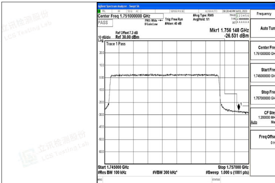
Band4_10MHz_QPSK_20350_50RB#0
