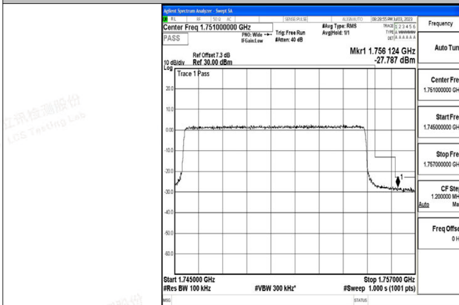
Band4_10MHz_16QAM_20350_50RB#0
