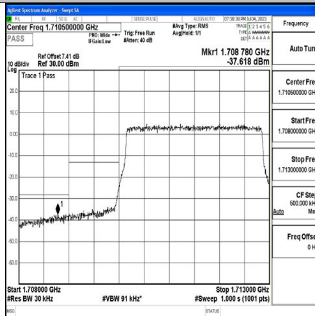
Band4_3MHz_16QAM_19965_15RB#0
