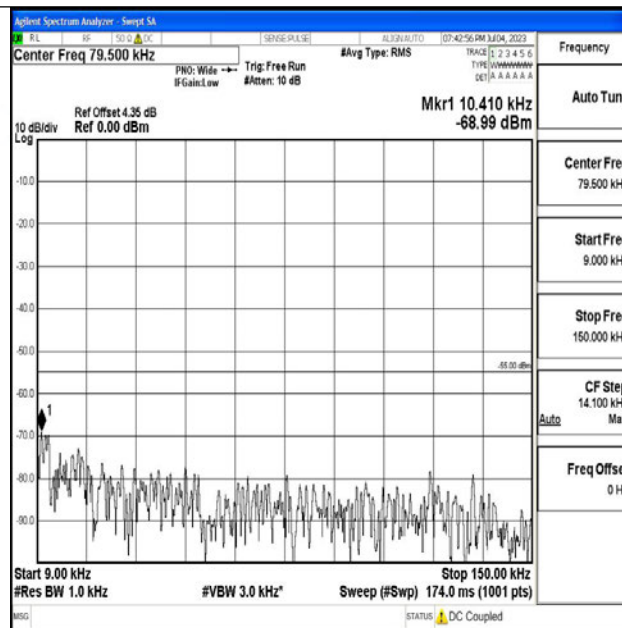
Band7_10MHz_QPSK_20800_1RB#0_0.009~0.15_0.009~0.15
