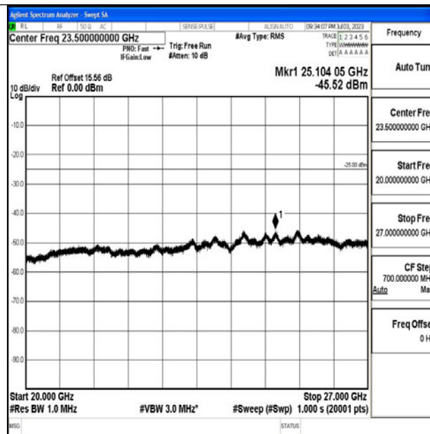
Band7_15MHz_QPSK_21375_1RB#0_20000~27000_20000~27000
