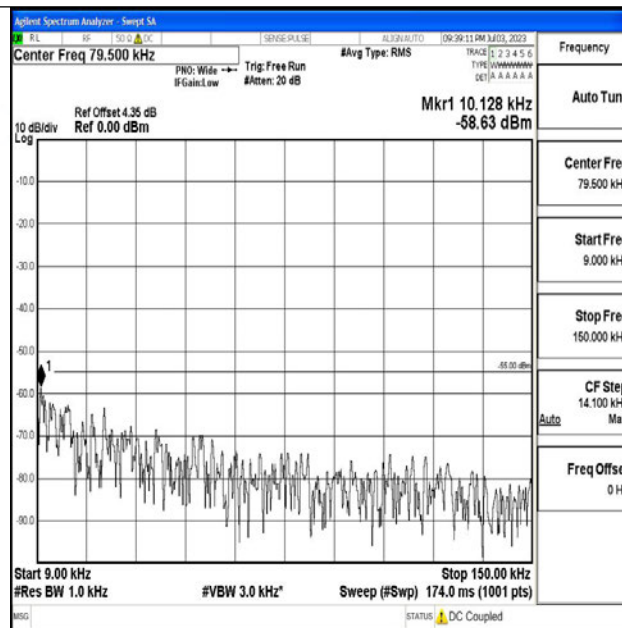
Band7_20MHz_QPSK_21100_1RB#0_0.009~0.15_0.009~0.15
