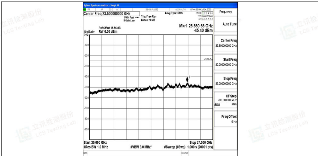
Band7_10MHz_QPSK_21100_1RB#0_20000~27000_20000~27000
