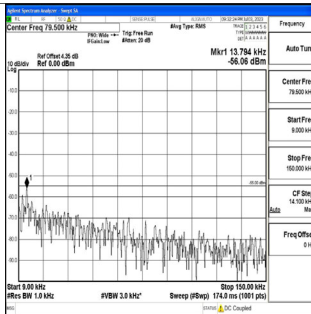
Band7_15MHz_QPSK_21100_1RB#0_0.009~0.15_0.009~0.15
