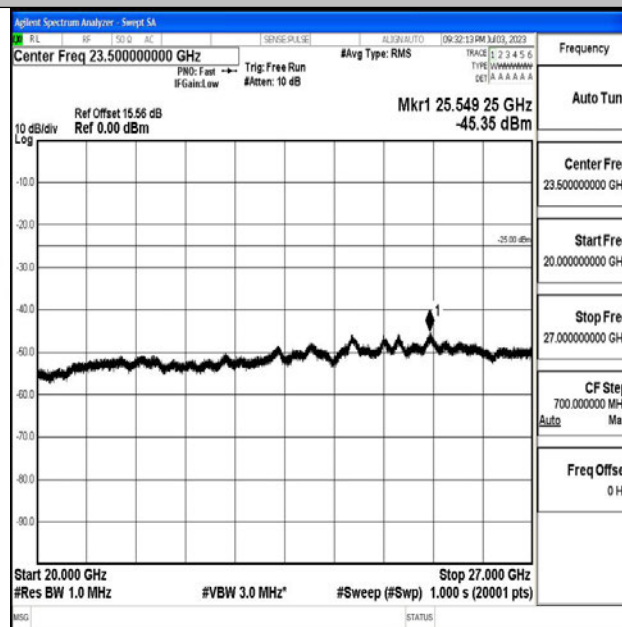
Band7_15MHz_16QAM_20825_1RB#0_20000~27000_20000~27000
