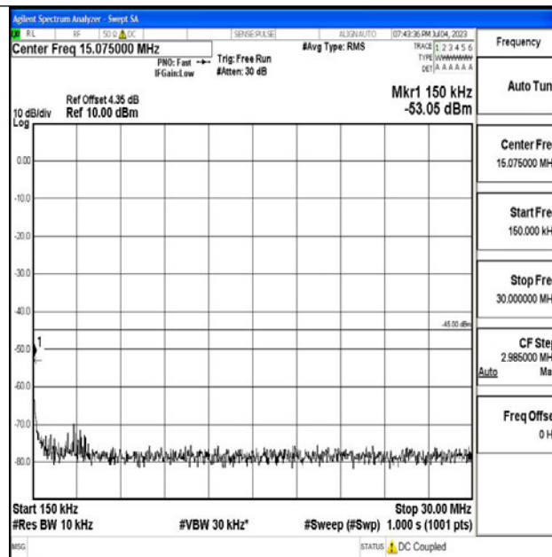
Band7_10MHz_16QAM_20800_1RB#0_0.15~30_0.15~30
