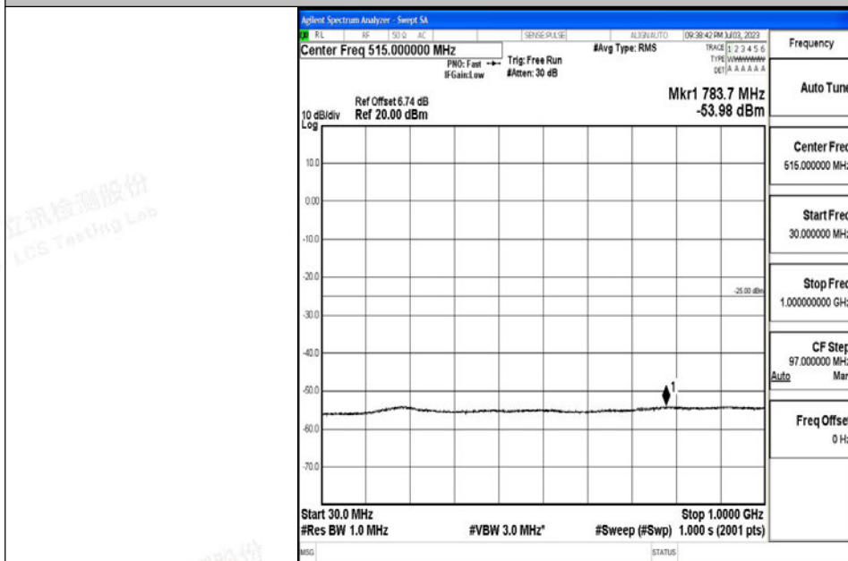
Band7_20MHz_16QAM_20850_1RB#0_30~1000_30~1000
