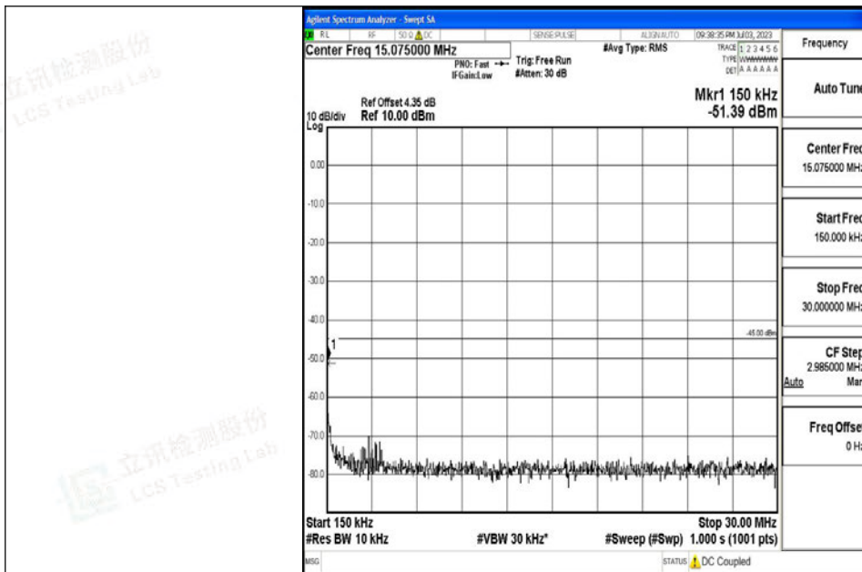
Band7_20MHz_16QAM_20850_1RB#0_0.15~30_0.15~30
