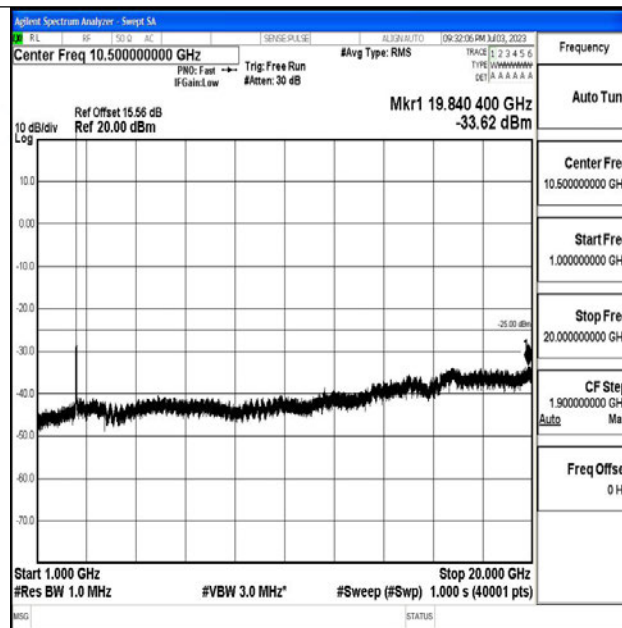
Band7_15MHz_16QAM_20825_1RB#0_1000~20000_1000~20000
