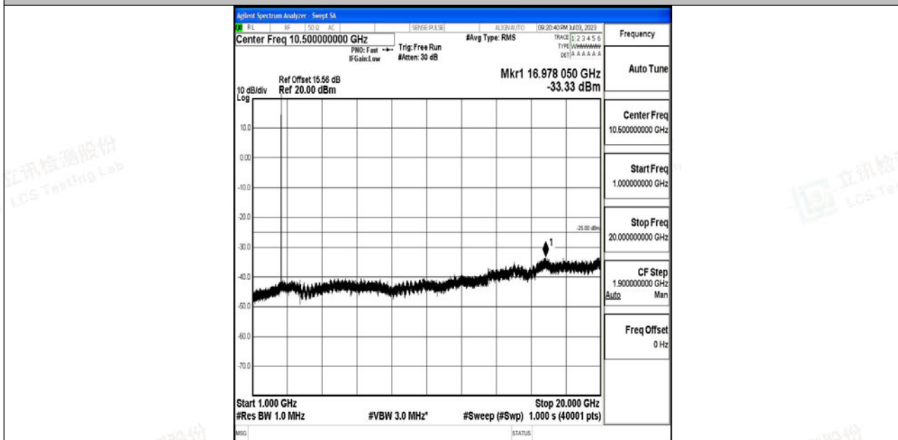
Band7_5MHz_QPSK_21425_1RB#0_1000~20000_1000~20000
