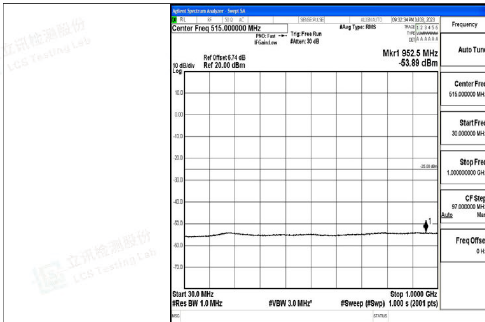
Band7_15MHz_QPSK_21100_1RB#0_30~1000_30~1000
