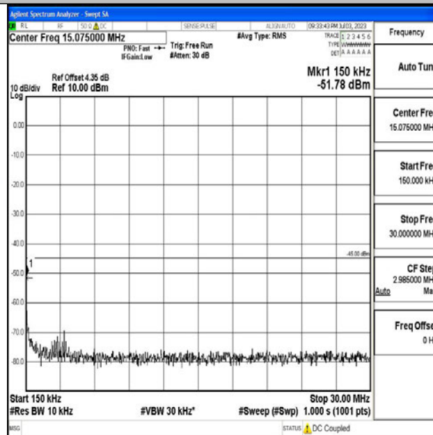
Band7_15MHz_QPSK_21375_1RB#0_0.15~30_0.15~30
