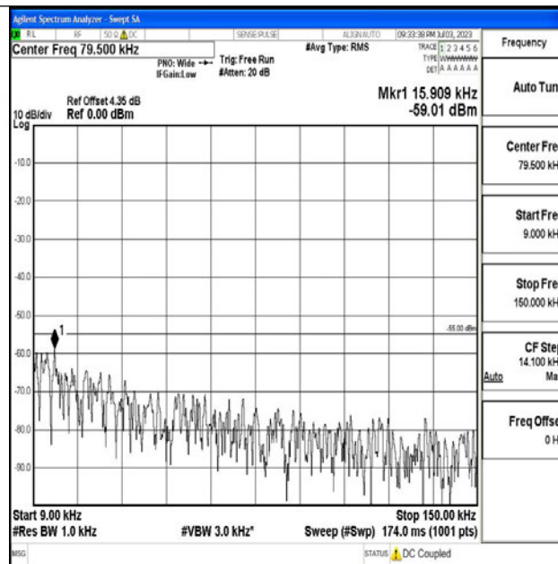
Band7_15MHz_QPSK_21375_1RB#0_0.009~0.15_0.009~0.15
