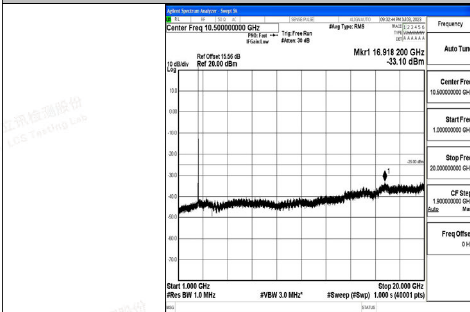
Band7_15MHz_QPSK_21100_1RB#0_1000~20000_1000~20000
