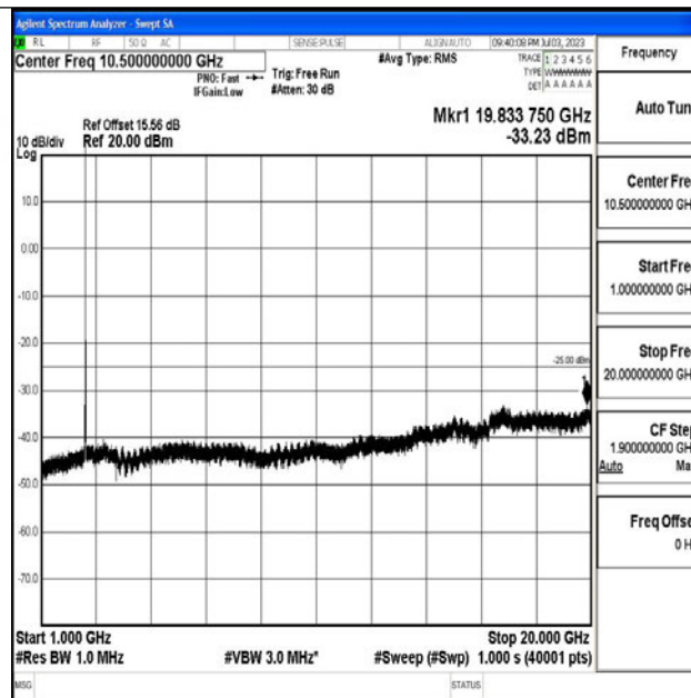
Band7_20MHz_16QAM_21100_1RB#0_1000~20000_1000~20000
