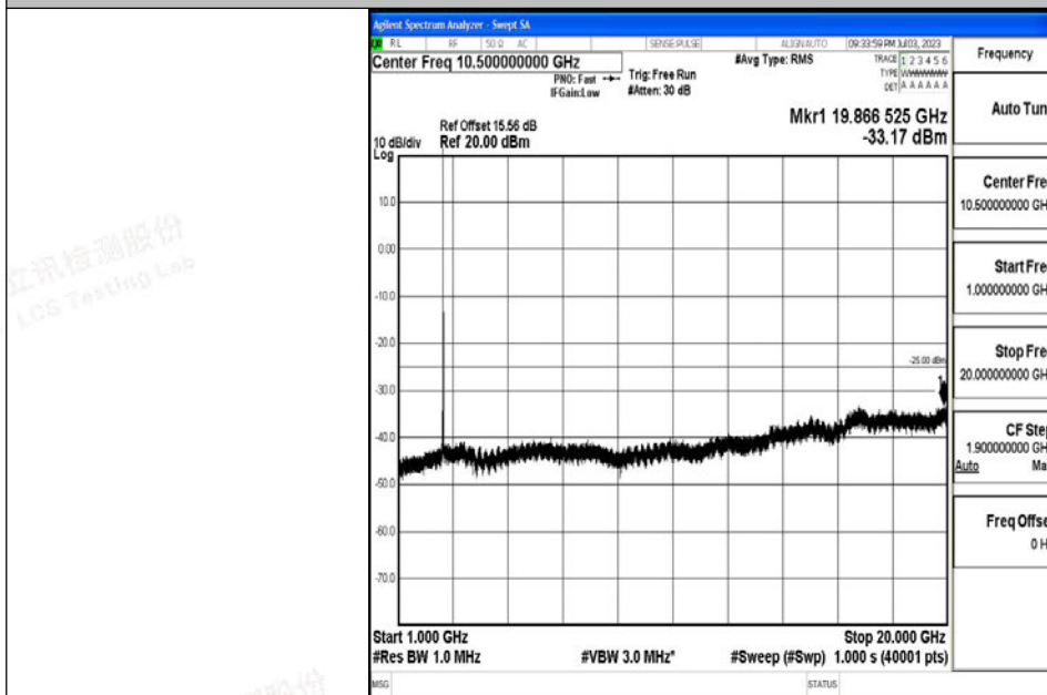
Band7_15MHz_QPSK_21375_1RB#0_1000~20000_1000~20000
