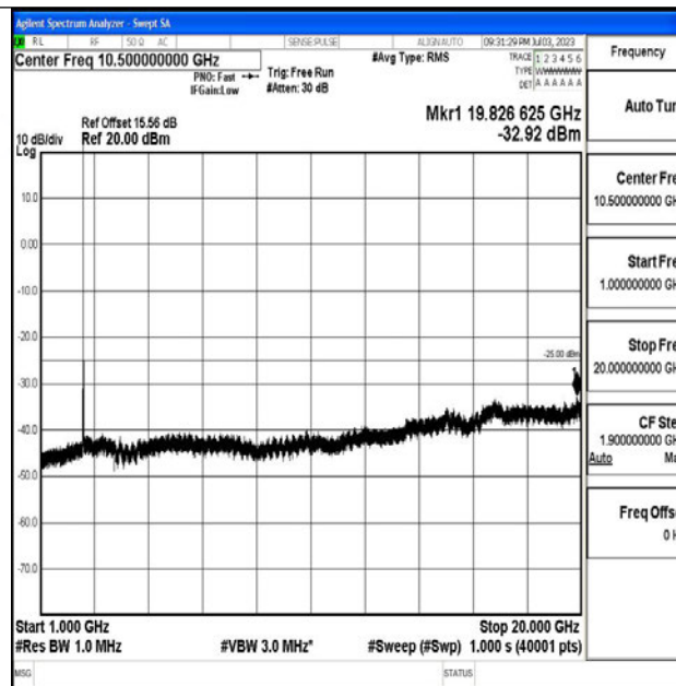
Band7_15MHz_QPSK_20825_1RB#0_1000~20000_1000~20000
