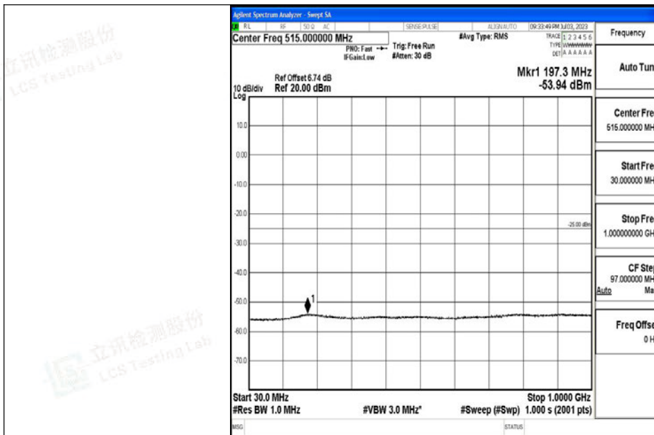
Band7_15MHz_QPSK_21375_1RB#0_30~1000_30~1000
