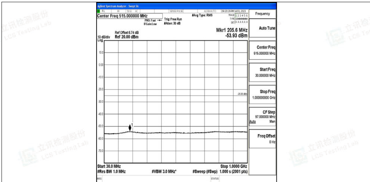
Band7_5MHz_QPSK_21425_1RB#0_30~1000_30~1000
