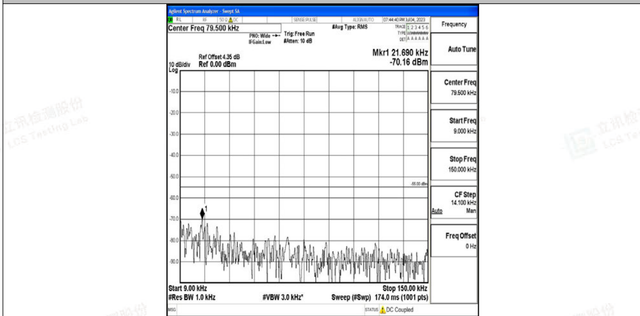
Band7_10MHz_16QAM_21100_1RB#0_0.009~0.15_0.009~0.15
