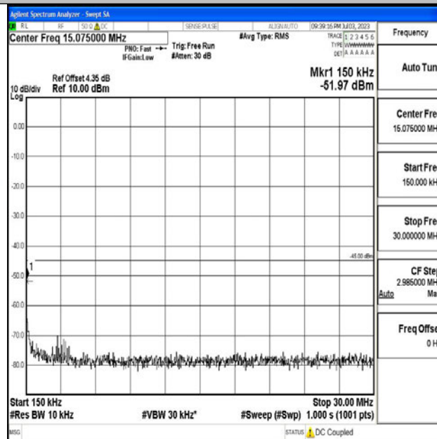
Band7_20MHz_QPSK_21100_1RB#0_0.15~30_0.15~30
