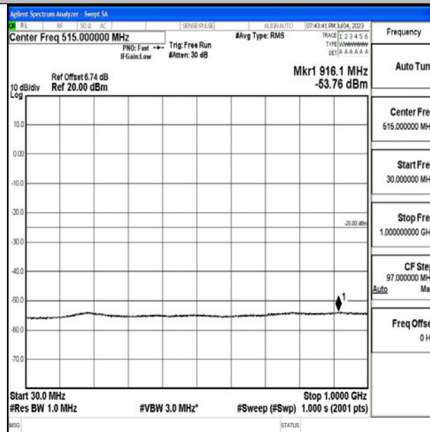
Band7_10MHz_16QAM_20800_1RB#0_30~1000_30~1000
