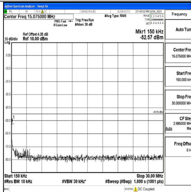
Band7_10MHz_QPSK_20800_1RB#0_0.15~30_0.15~30
