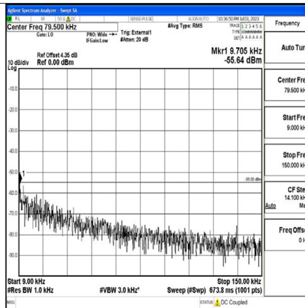
Band38_5MHz_QPSK_38000_1RB#0_0.009~0.15_0.009~0.15
