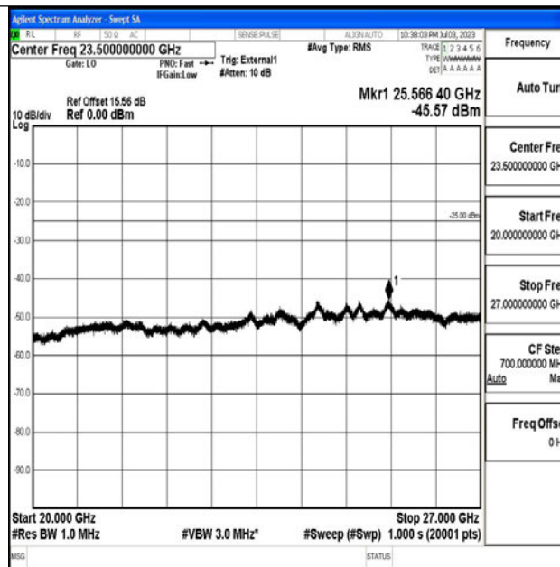
Band38_5MHz_QPSK_38000_1RB#0_20000~27000_20000~27000
