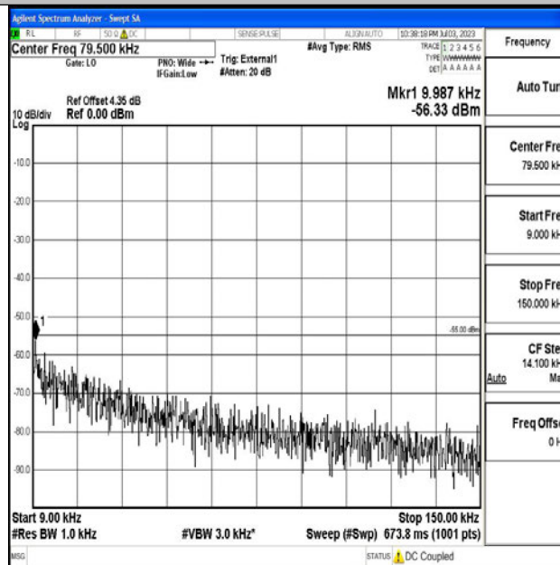
Band38_5MHz_16QAM_38000_1RB#0_0.009~0.15_0.009~0.15
