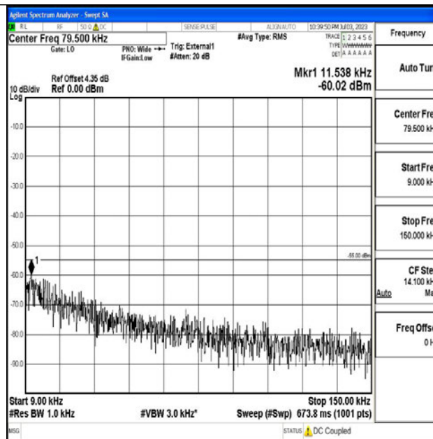
Band38_5MHz_QPSK_38225_1RB#0_0.009~0.15_0.009~0.15
