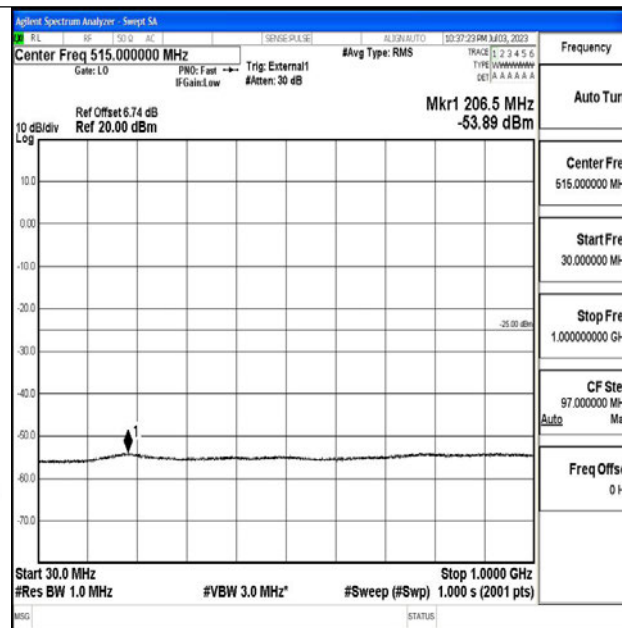
Band38_5MHz_QPSK_38000_1RB#0_30~1000_30~1000
