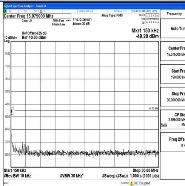
Band38_5MHz_QPSK_38225_1RB#0_0.15~30_0.15~30
