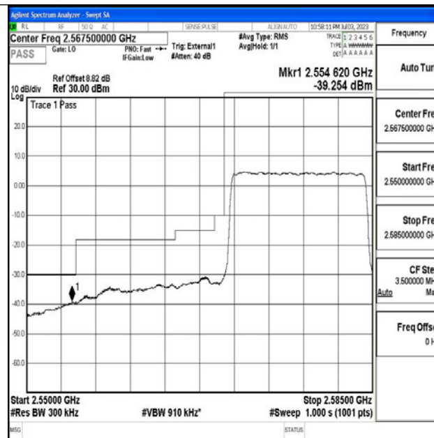
Band38_15MHz_16QAM_37825_75RB#0
