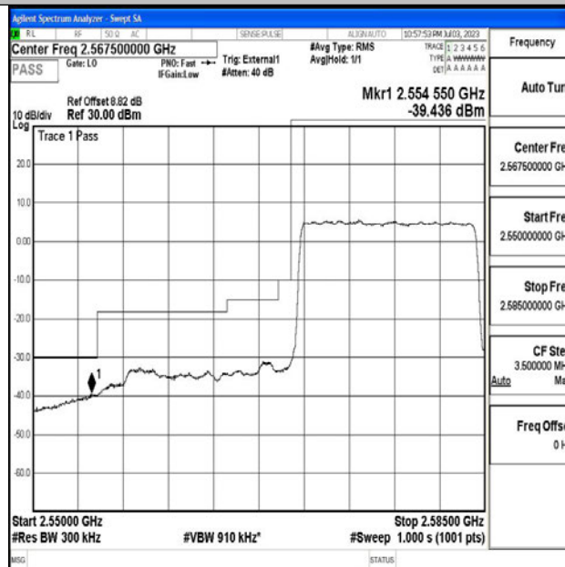
Band38_15MHz_QPSK_37825_75RB#0
