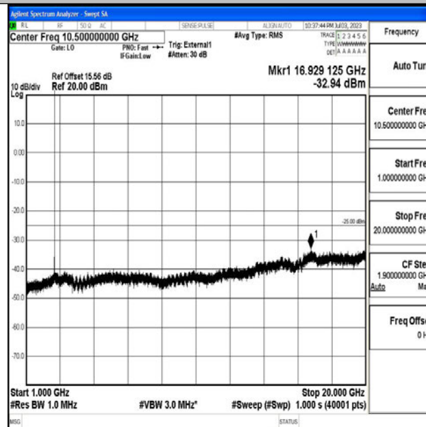
Band38_5MHz_QPSK_38000_1RB#0_1000~20000_1000~20000
