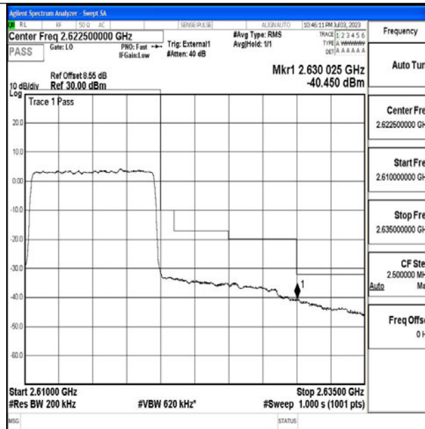
Band38_10MHz_16QAM_38200_50RB#0
