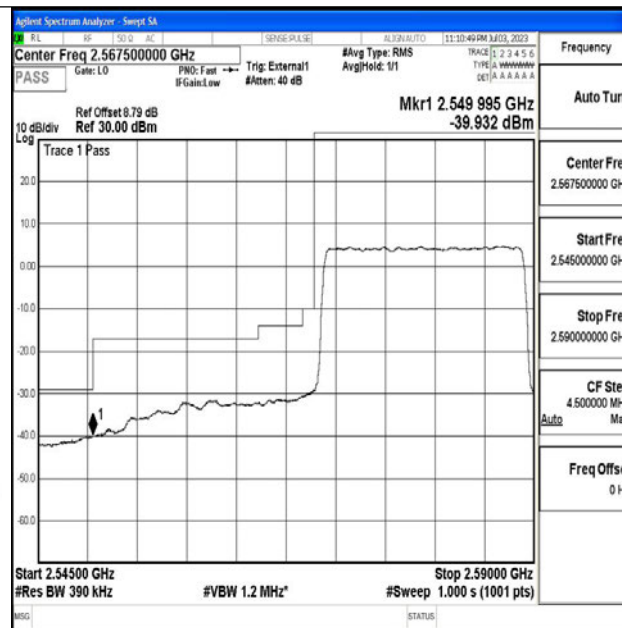
Band38_20MHz_16QAM_37850_100RB#0
