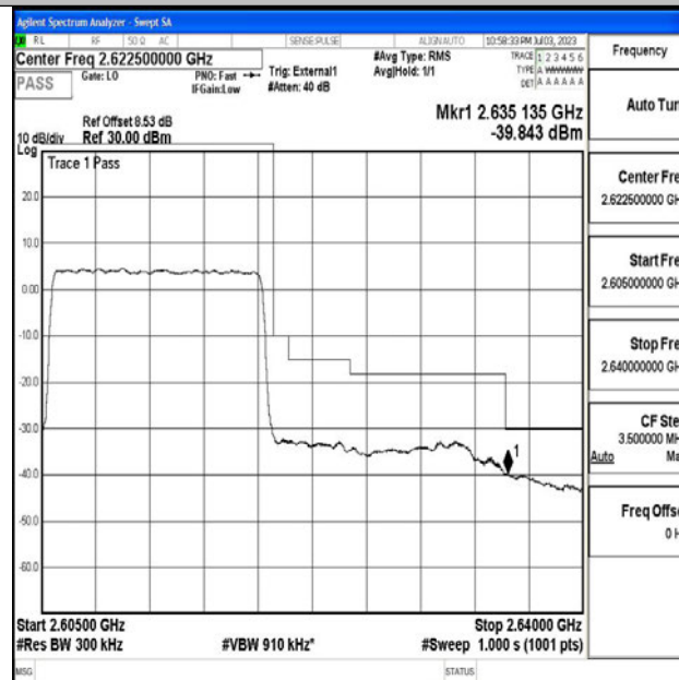
Band38_15MHz_QPSK_38175_75RB#0
