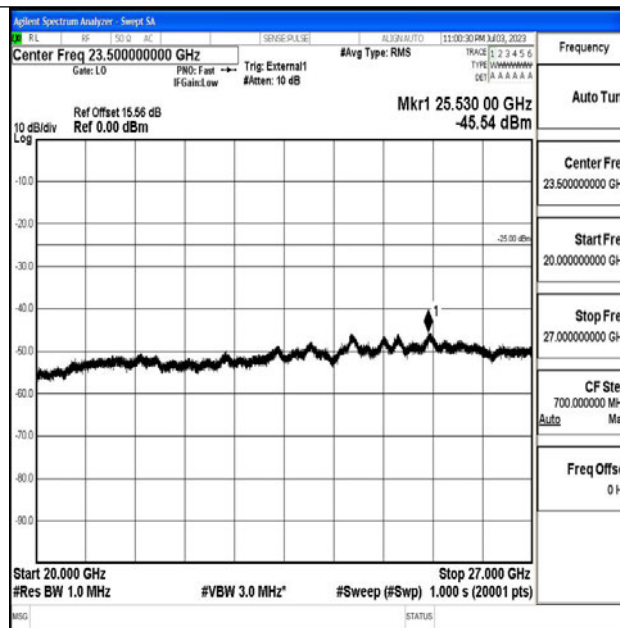
Band38_15MHz_QPSK_37825_1RB#0_20000~27000_20000~27000
