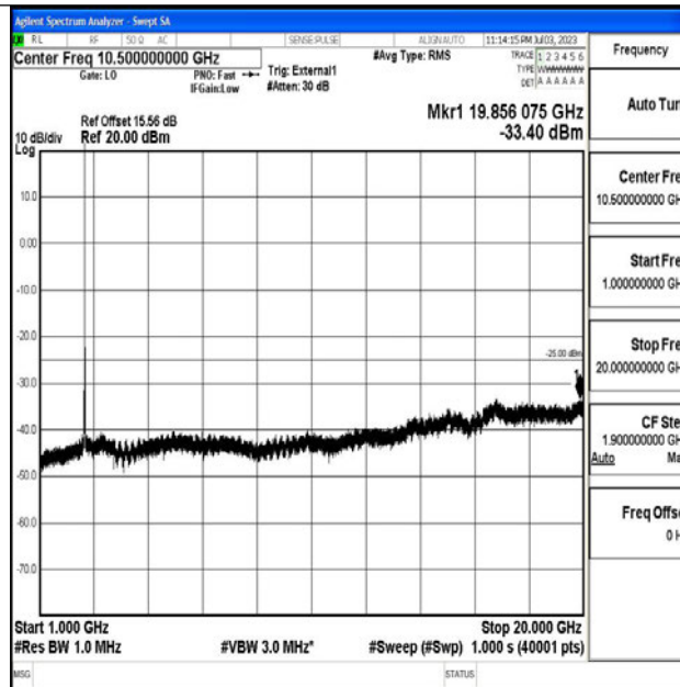
Band38_20MHz_16QAM_37850_1RB#0_1000~20000_1000~20000
