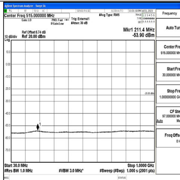
Band38_15MHz_16QAM_37825_1RB#0_30~1000_30~1000
