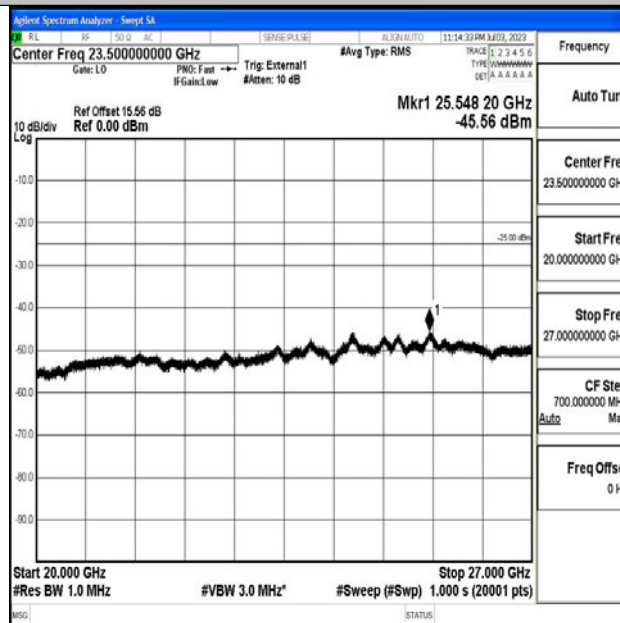
Band38_20MHz_16QAM_37850_1RB#0_20000~27000_20000~27000
