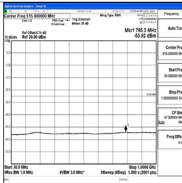
Band38_15MHz_QPSK_37825_1RB#0_30~1000_30~1000
