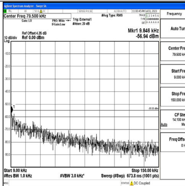
Band38_15MHz_16QAM_37825_1RB#0_0.009~0.15_0.009~0.15
