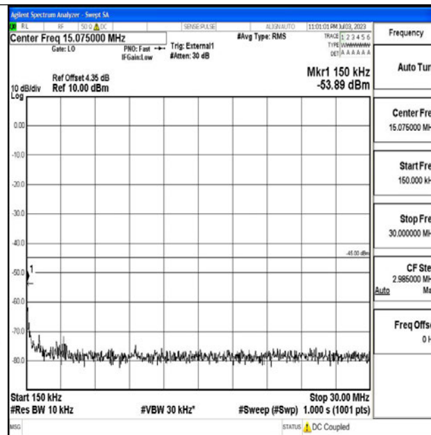
Band38_15MHz_16QAM_37825_1RB#0_0.15~30_0.15~30
