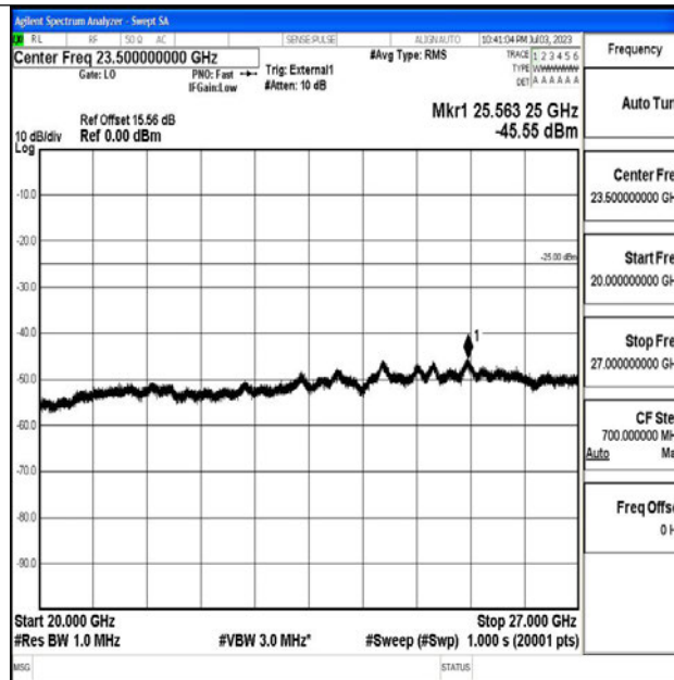
Band38_5MHz_QPSK_38225_1RB#0_20000~27000_20000~27000
