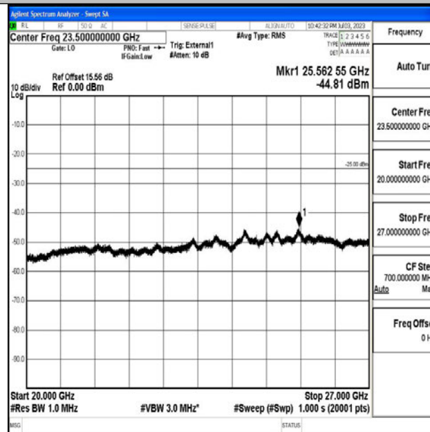
Band38_5MHz_16QAM_38225_1RB#0_20000~27000_20000~27000
