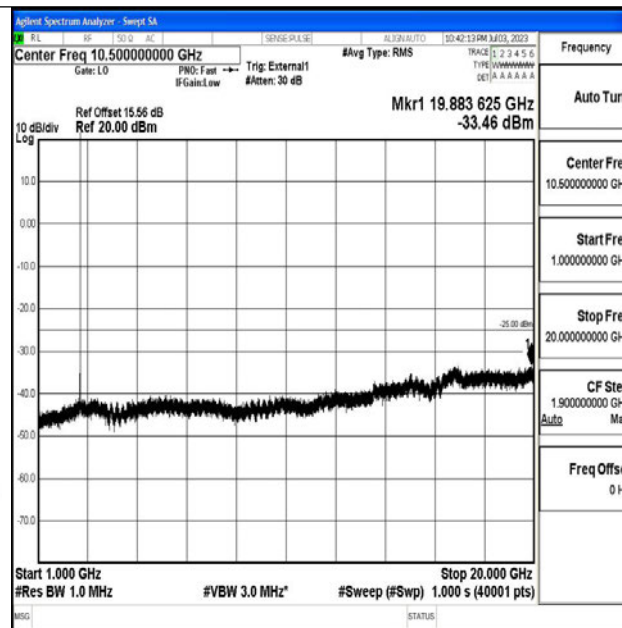
Band38_5MHz_16QAM_38225_1RB#0_1000~20000_1000~20000
