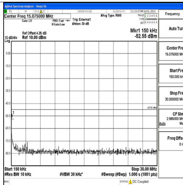
Band38_20MHz_16QAM_37850_1RB#0_0.15~30_0.15~30
