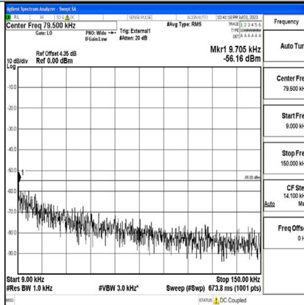
Band38_5MHz_16QAM_38225_1RB#0_0.009~0.15_0.009~0.15
