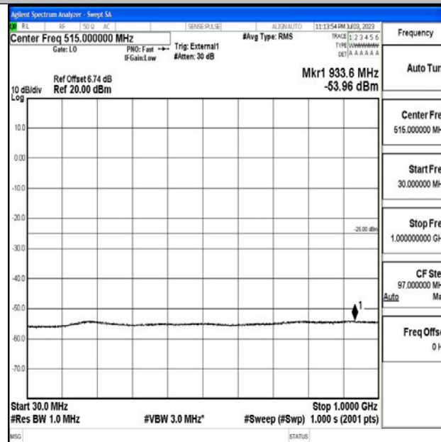
Band38_20MHz_16QAM_37850_1RB#0_30~1000_30~1000
