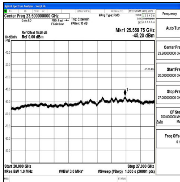
Band38_15MHz_QPSK_38000_1RB#0_20000~27000_20000~27000
