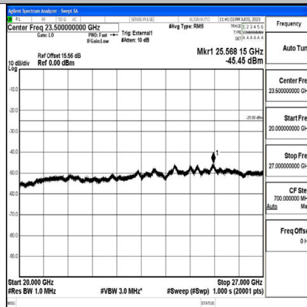
Band41_10MHz_16QAM_39700_1RB#0_20000~27000_20000~27000
