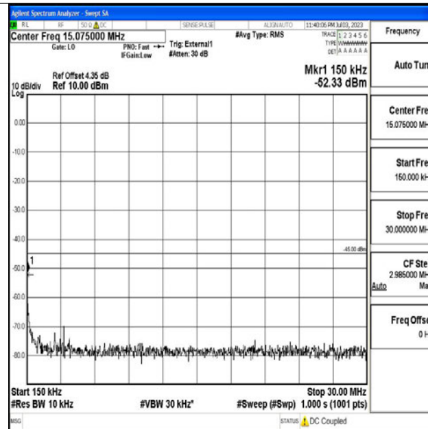
Band41_10MHz_16QAM_39700_1RB#0_0.15~30_0.15~30
