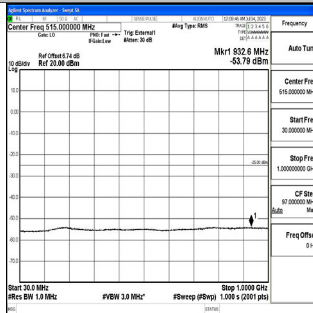
Band41_20MHz_16QAM_40620_1RB#0_30~1000_30~1000
