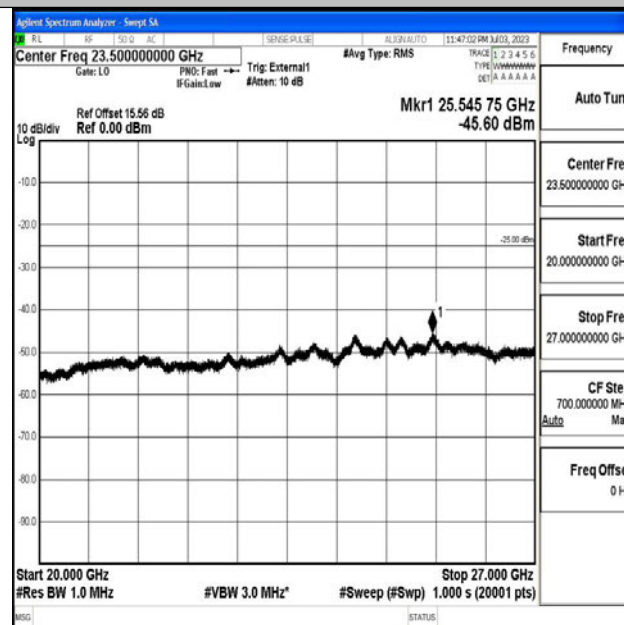
Band41_10MHz_16QAM_41540_1RB#0_20000~27000_20000~27000
