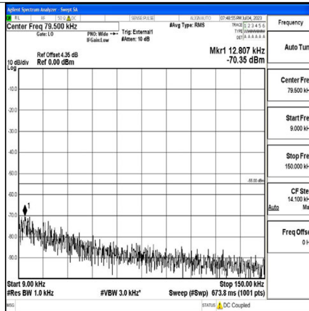
Band41_15MHz_QPSK_39725_1RB#0_0.009~0.15_0.009~0.15
