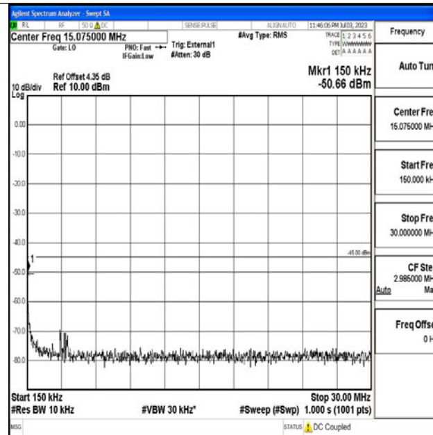
Band41_10MHz_16QAM_41540_1RB#0_0.15~30_0.15~30
