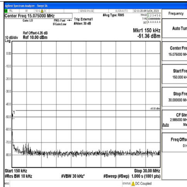
Band41_20MHz_16QAM_41490_1RB#0_0.15~30_0.15~30
