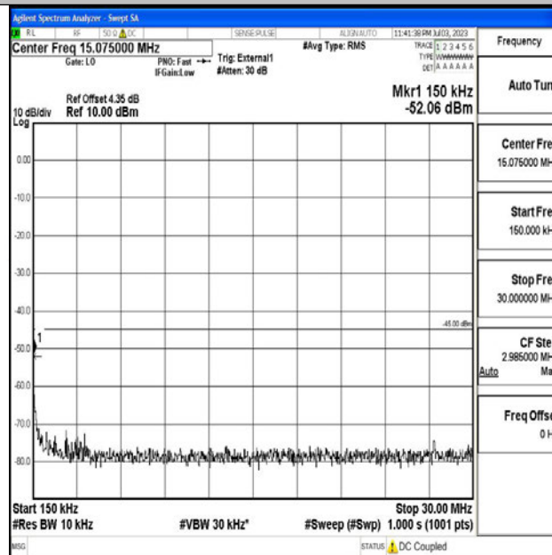
Band41_10MHz_QPSK_40620_1RB#0_0.15~30_0.15~30
