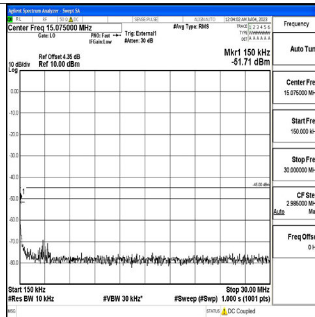
Band41_20MHz_QPSK_39750_1RB#0_0.15~30_0.15~30
