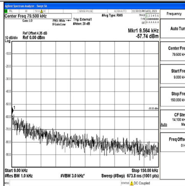
Band41_5MHz_16QAM_41565_1RB#0_0.009~0.15_0.009~0.15
