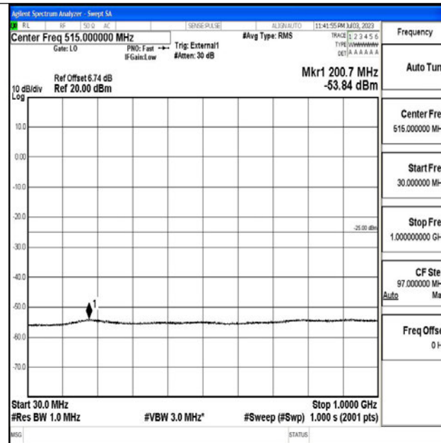
Band41_10MHz_QPSK_40620_1RB#0_30~1000_30~1000
