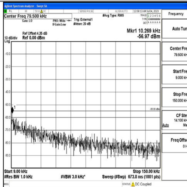
Band41_20MHz_16QAM_40620_1RB#0_0.009~0.15_0.009~0.15
