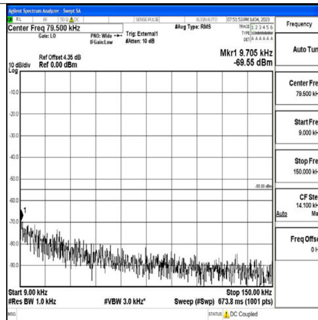
Band41_15MHz_QPSK_40620_1RB#0_0.009~0.15_0.009~0.15
