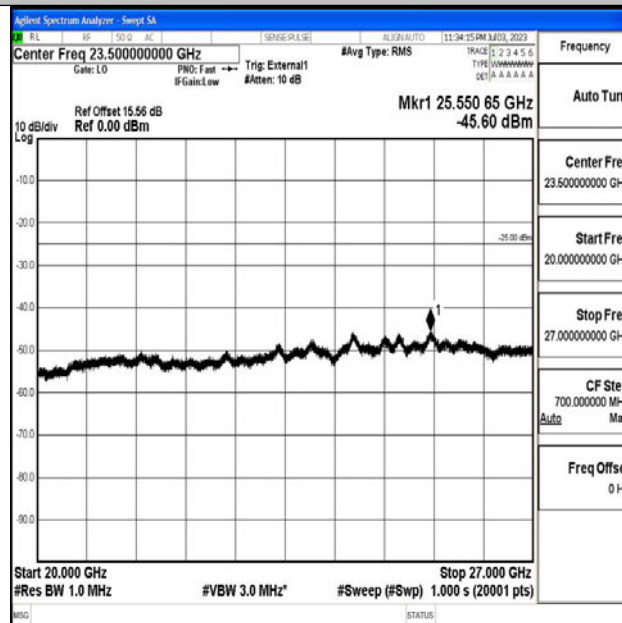
Band41_5MHz_16QAM_41565_1RB#0_20000~27000_20000~27000
