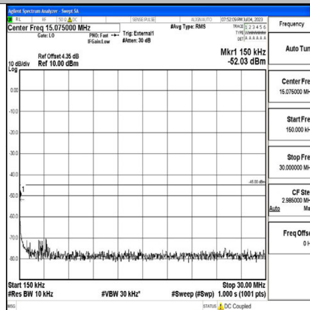
Band41_15MHz_QPSK_40620_1RB#0_0.15~30_0.15~30
