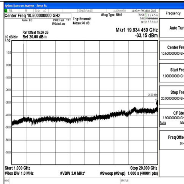
Band41_10MHz_16QAM_40620_1RB#0_1000~20000_1000~20000
