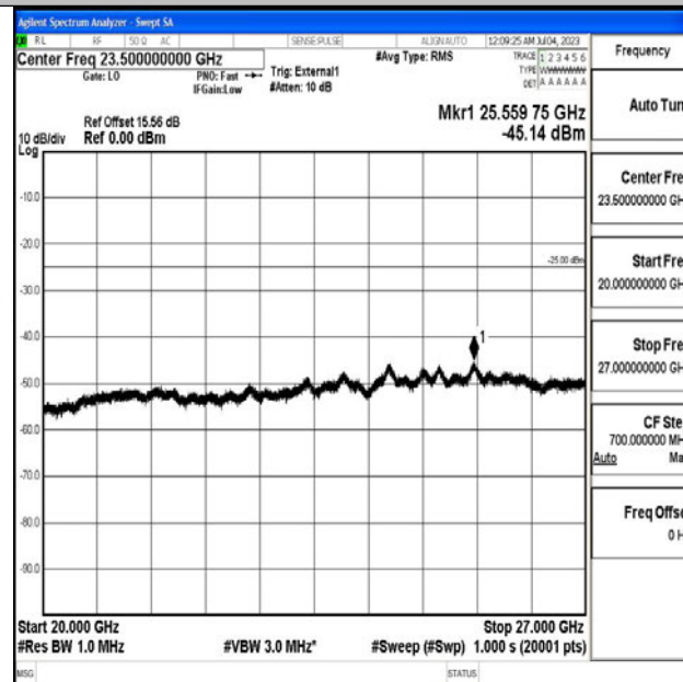
Band41_20MHz_16QAM_40620_1RB#0_20000~27000_20000~27000
