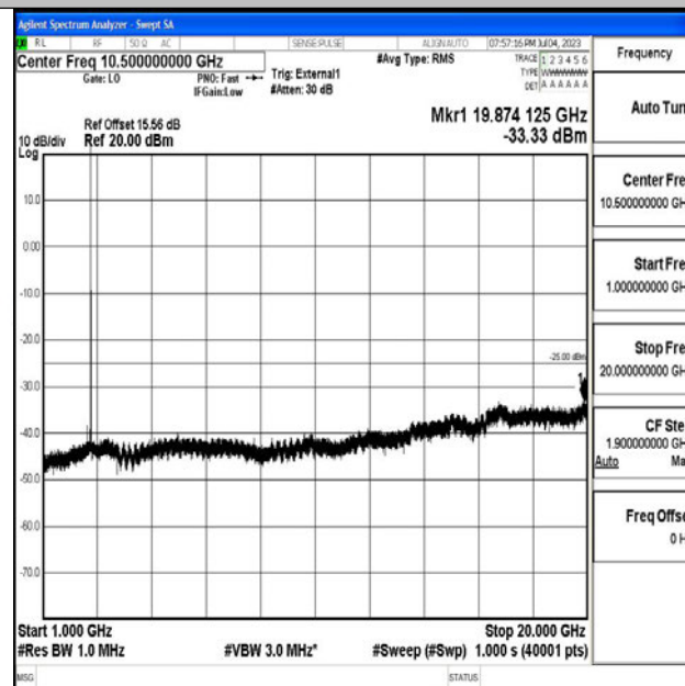
Band41_15MHz_16QAM_41515_1RB#0_1000~20000_1000~20000
