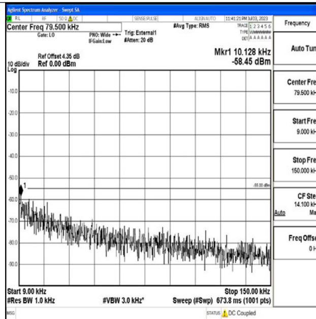
Band41_10MHz_QPSK_40620_1RB#0_0.009~0.15_0.009~0.15
