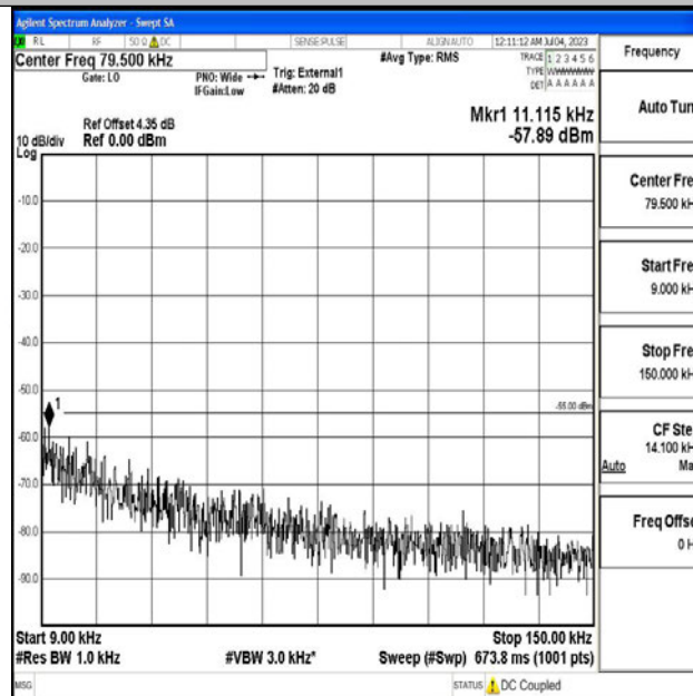
Band41_20MHz_16QAM_41490_1RB#0_0.009~0.15_0.009~0.15
