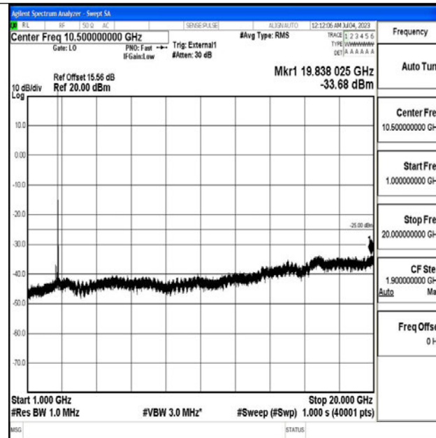
Band41_20MHz_16QAM_41490_1RB#0_1000~20000_1000~20000
