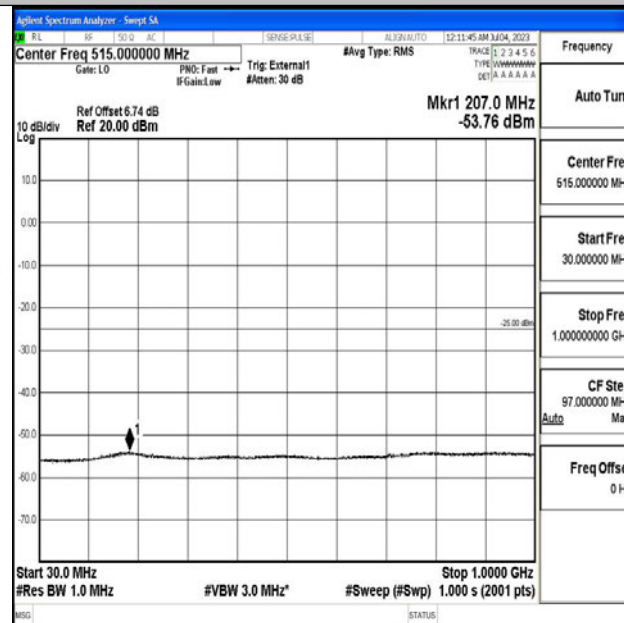
Band41_20MHz_16QAM_41490_1RB#0_30~1000_30~1000
