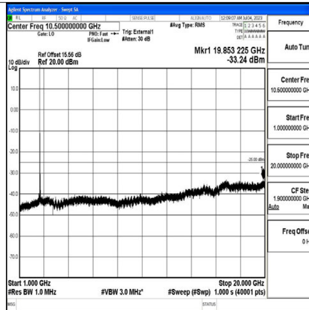
Band41_20MHz_16QAM_40620_1RB#0_1000~20000_1000~20000
