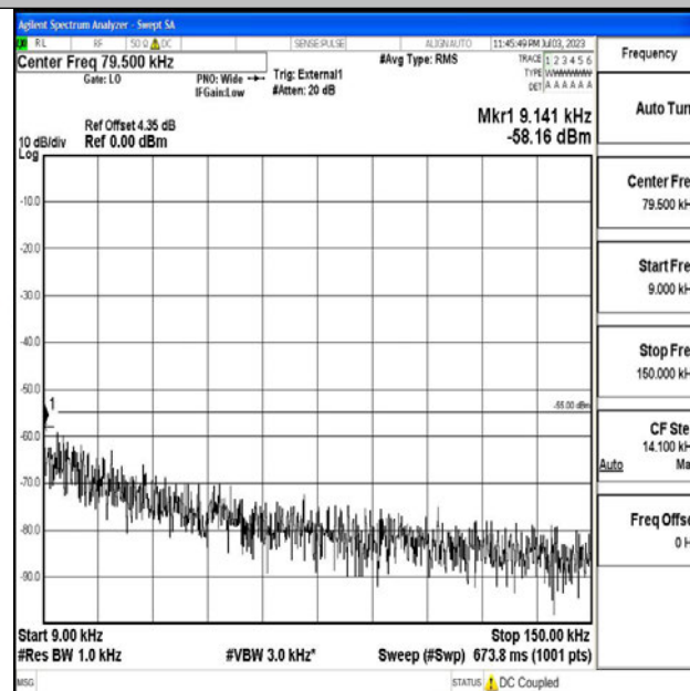
Band41_10MHz_16QAM_41540_1RB#0_0.009~0.15_0.009~0.15
