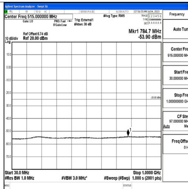
Band41_15MHz_16QAM_41515_1RB#0_30~1000_30~1000
