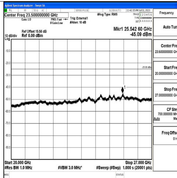
Band41_10MHz_QPSK_40620_1RB#0_20000~27000_20000~27000
