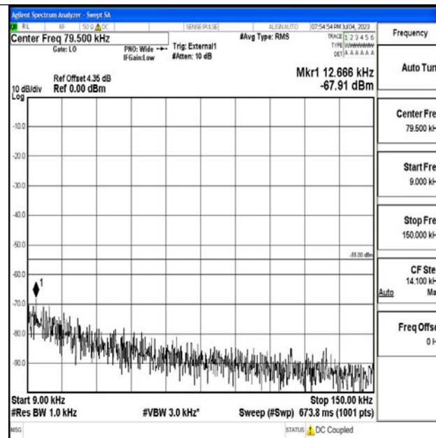
Band41_15MHz_QPSK_41515_1RB#0_0.009~0.15_0.009~0.15
