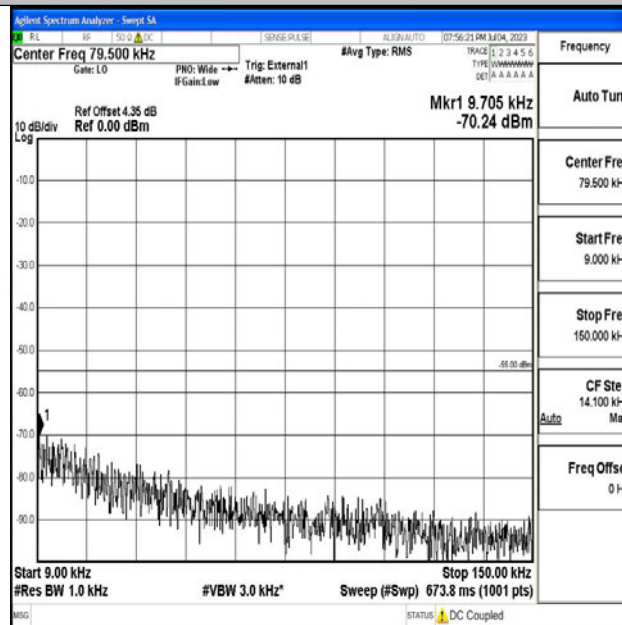
Band41_15MHz_16QAM_41515_1RB#0_0.009~0.15_0.009~0.15
