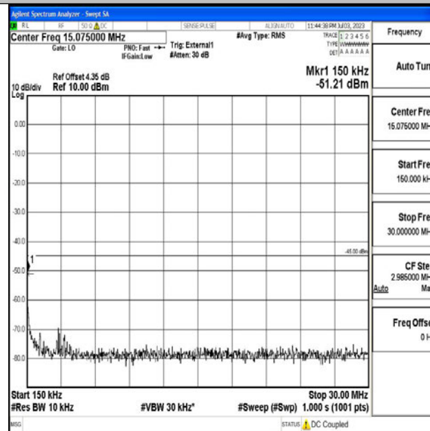
Band41_10MHz_QPSK_41540_1RB#0_0.15~30_0.15~30
