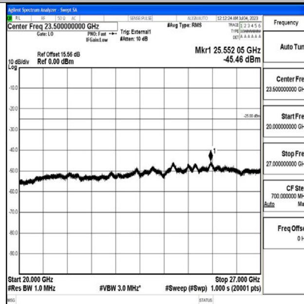
Band41_20MHz_16QAM_41490_1RB#0_20000~27000_20000~27000
