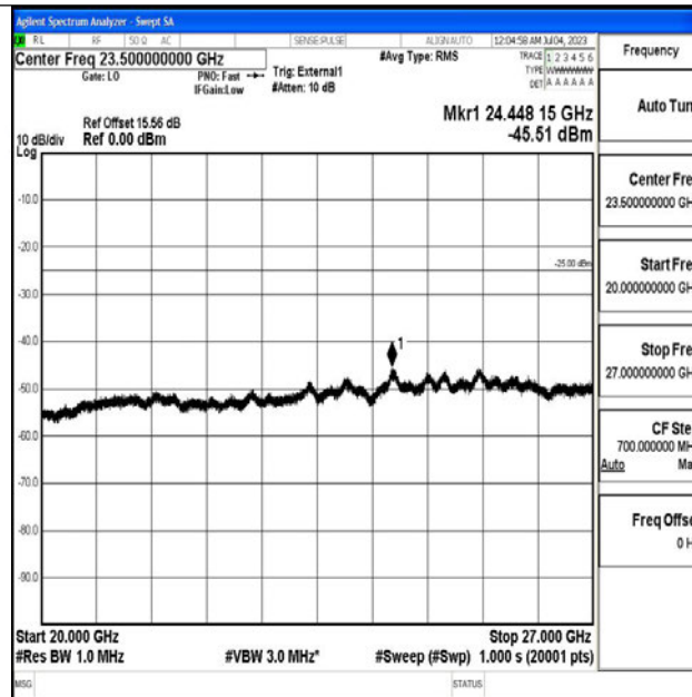
Band41_20MHz_QPSK_39750_1RB#0_20000~27000_20000~27000
