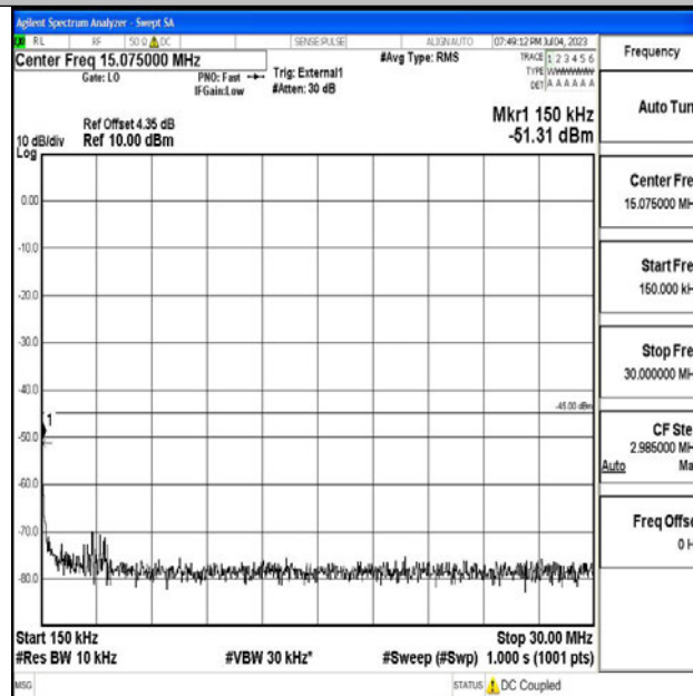
Band41_15MHz_QPSK_39725_1RB#0_0.15~30_0.15~30
