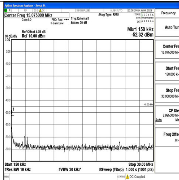
Band41_20MHz_16QAM_40620_1RB#0_0.15~30_0.15~30
