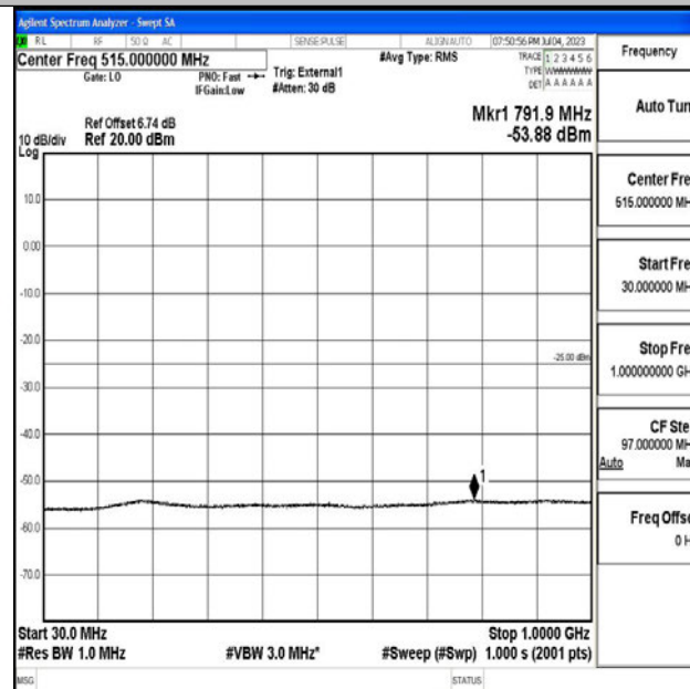
Band41_15MHz_16QAM_39725_1RB#0_30~1000_30~1000
