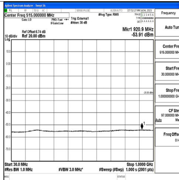
Band41_15MHz_QPSK_40620_1RB#0_30~1000_30~1000
