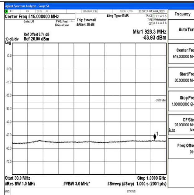
Band41_20MHz_QPSK_41490_1RB#0_30~1000_30~1000
