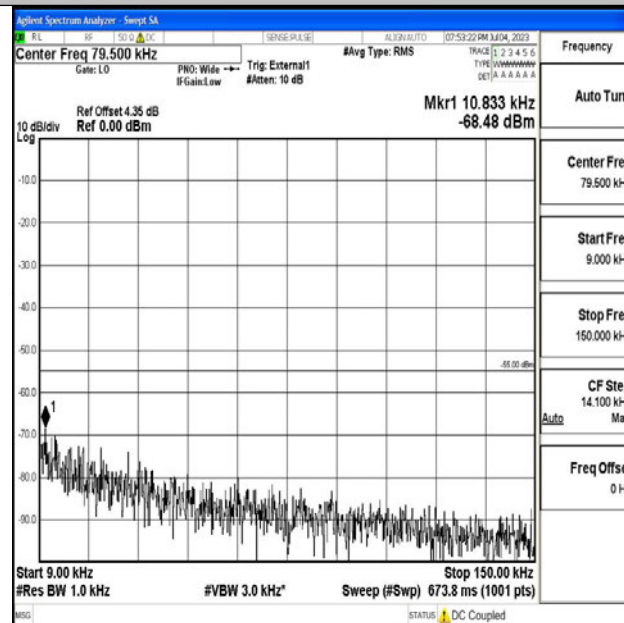
Band41_15MHz_16QAM_40620_1RB#0_0.009~0.15_0.009~0.15
