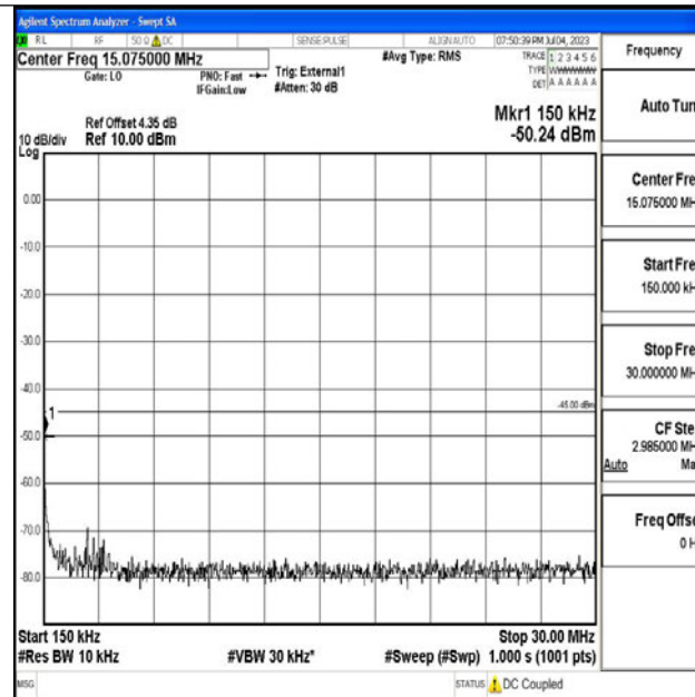
Band41_15MHz_16QAM_39725_1RB#0_0.15~30_0.15~30
