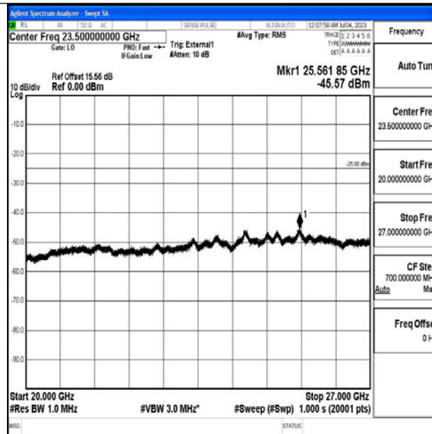
Band41_20MHz_QPSK_40620_1RB#0_20000~27000_20000~27000
