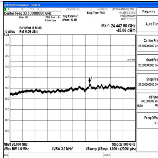
Band41_5MHz_QPSK_41565_1RB#0_20000~27000_20000~27000
