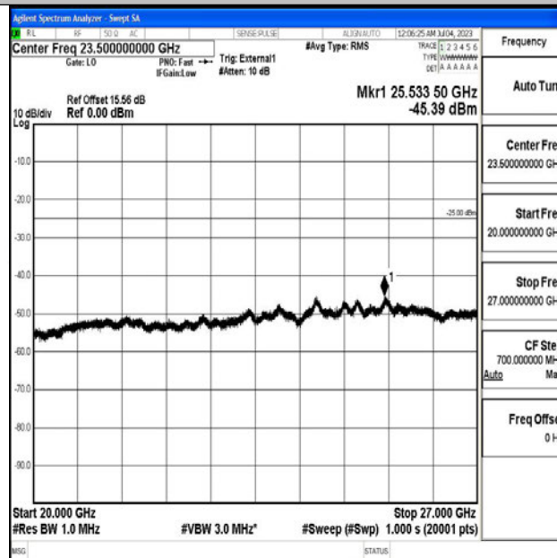
Band41_20MHz_16QAM_39750_1RB#0_20000~27000_20000~27000
