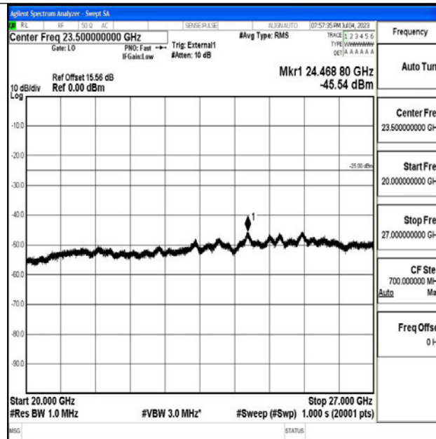
Band41_15MHz_16QAM_41515_1RB#0_20000~27000_20000~27000
