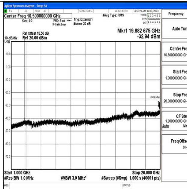
Band41_5MHz_16QAM_41565_1RB#0_1000~20000_1000~20000
