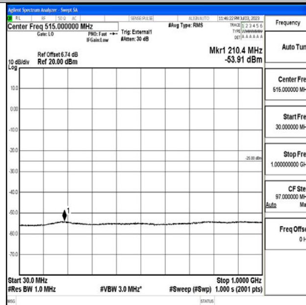
Band41_10MHz_16QAM_41540_1RB#0_30~1000_30~1000
