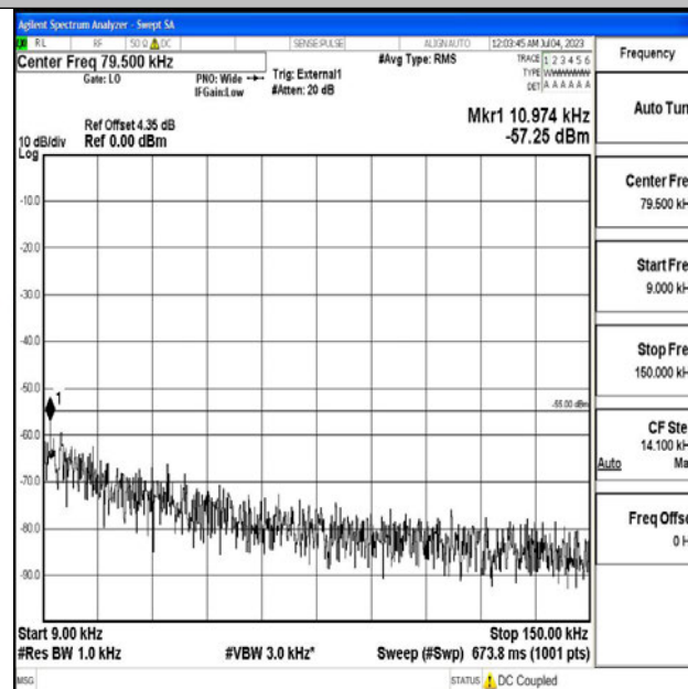
Band41_20MHz_QPSK_39750_1RB#0_0.009~0.15_0.009~0.15
