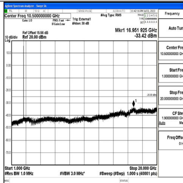
Band41_10MHz_QPSK_40620_1RB#0_1000~20000_1000~20000
