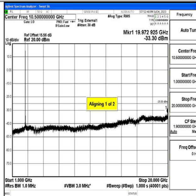
Band41_15MHz_QPSK_40620_1RB#0_1000~20000_1000~20000
