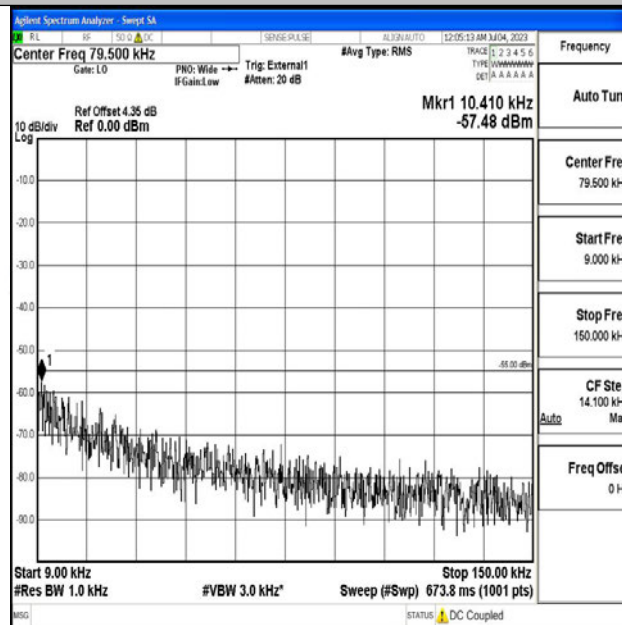
Band41_20MHz_16QAM_39750_1RB#0_0.009~0.15_0.009~0.15
