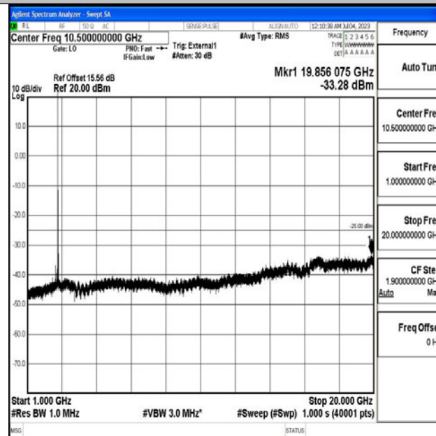
Band41_20MHz_QPSK_41490_1RB#0_1000~20000_1000~20000
