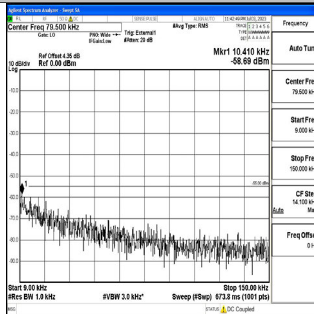
Band41_10MHz_16QAM_40620_1RB#0_0.009~0.15_0.009~0.15
