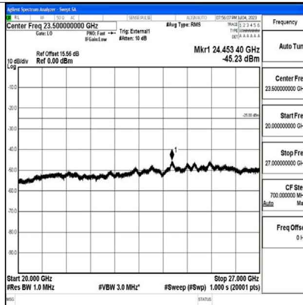
Band41_15MHz_QPSK_41515_1RB#0_20000~27000_20000~27000
