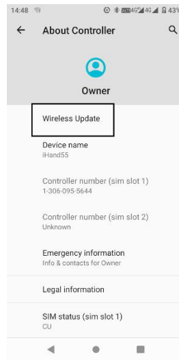
Figure 1-5-15 Update App
