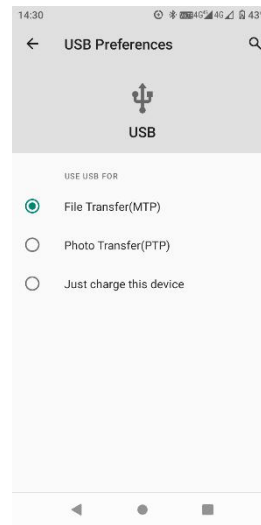
Figure 1-5-3 File transfers
