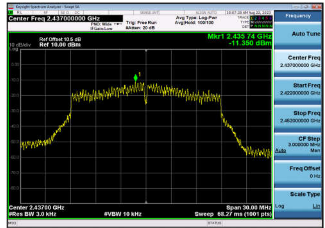
Power spectral density-802.11n(HT20) ,2437MHz,Ant0
