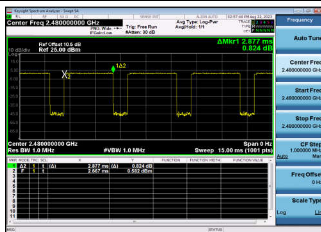
DQPSK,2480,2DH5,Transmission Time
