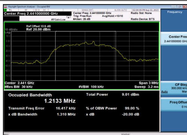
20dB Bandwidth: 8DPSK,2441MHz,3DH5
