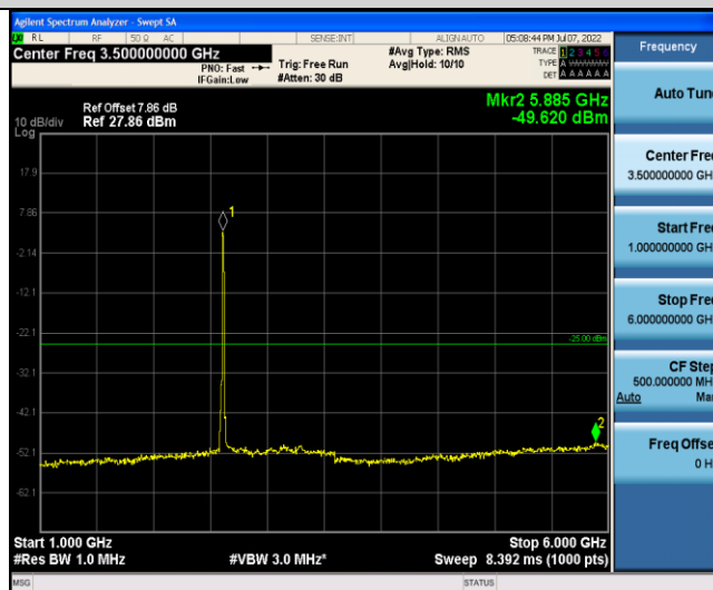
Band38-15MHz-QPSK-38175-75RB#0-Range3:6000~27000MHz
