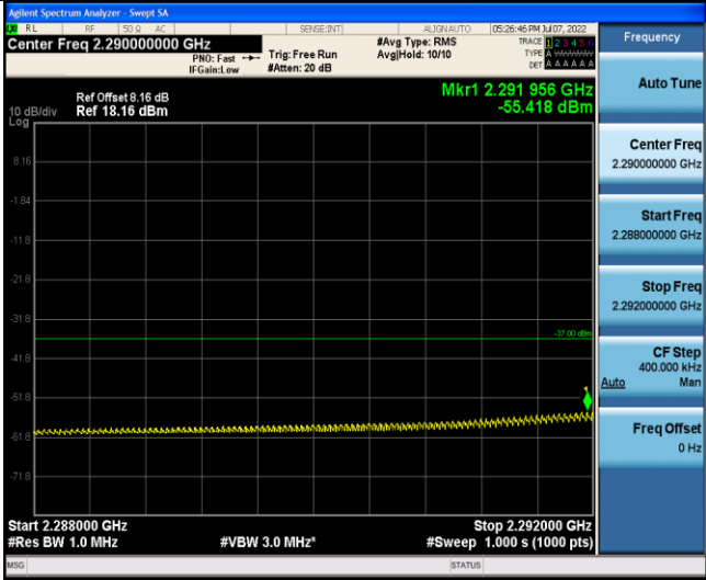
Band40-5MHz-QPSK-38725-25RB#0-Range3:2288~2292MHz
