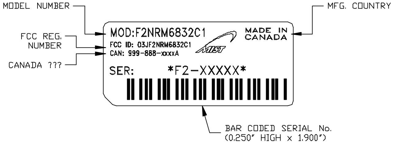
FIGURE 2 FCC ID LBL FOR CDPD MODEM
