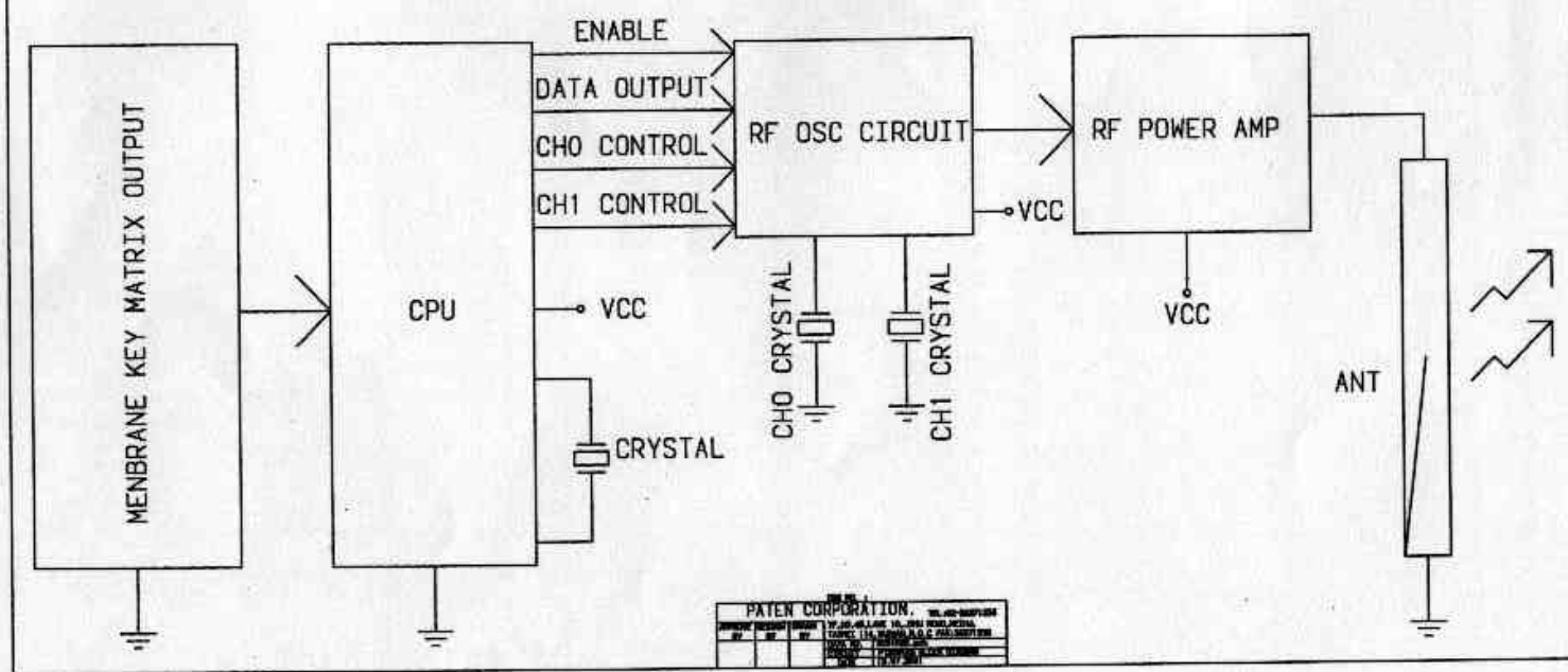
PT2001 CORDLESS KEYBOARD BLOCK DIAGRAM
