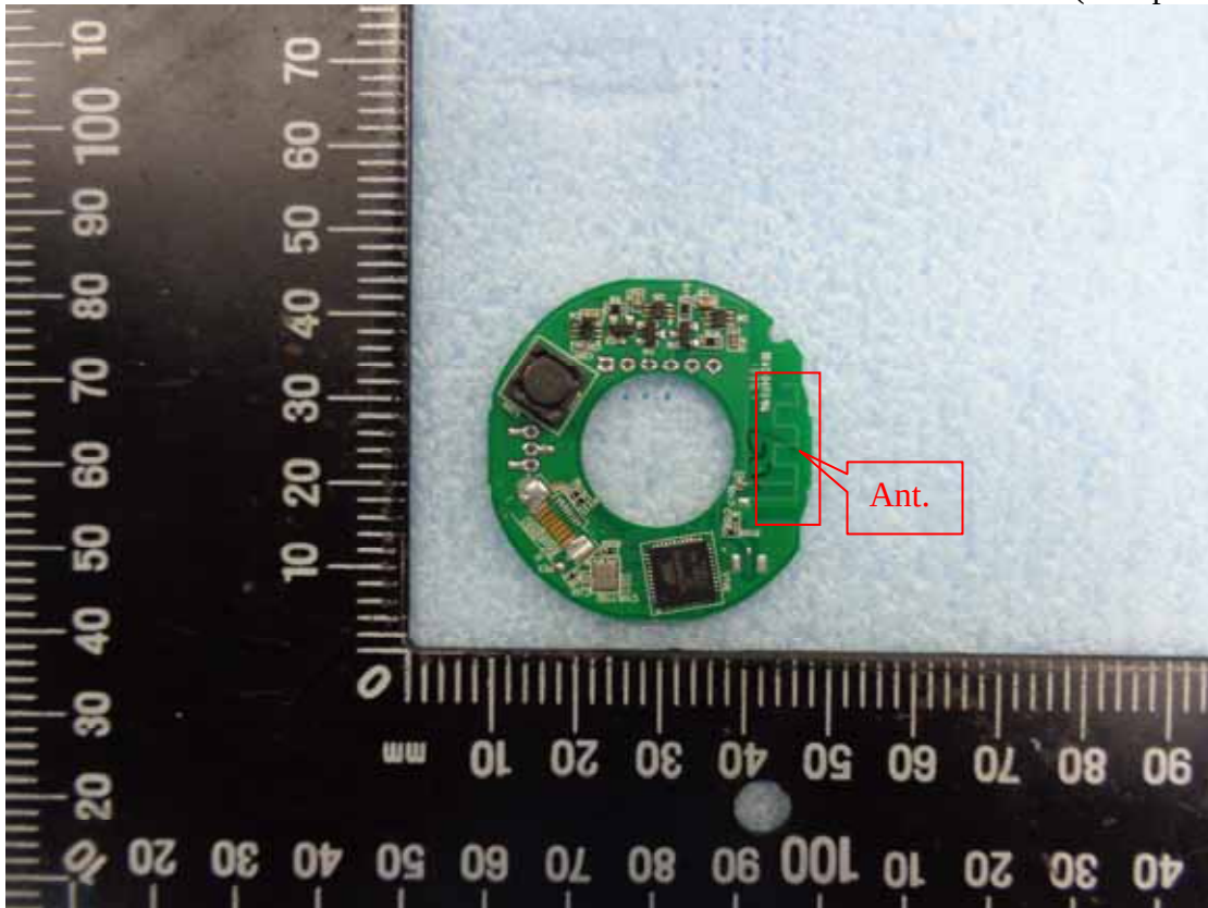
Figure 7 Wireless Board (Component Side)
