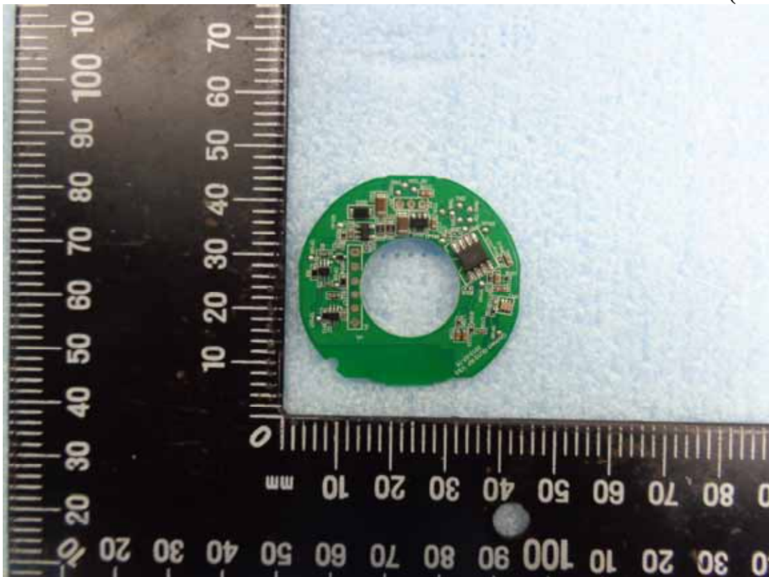
Figure 8 Wireless Board (Solder Side)
