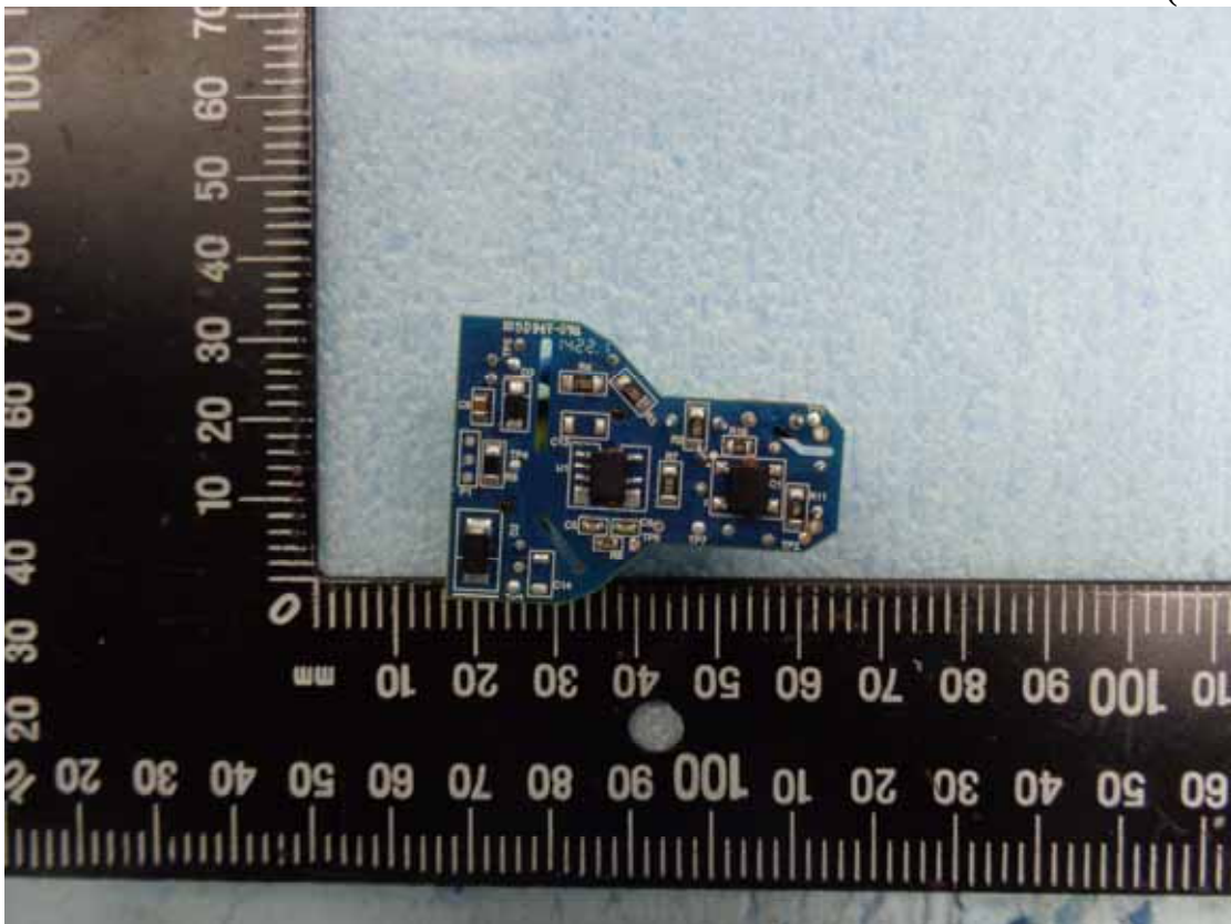
Figure 6 Power Board (Solder Side)
