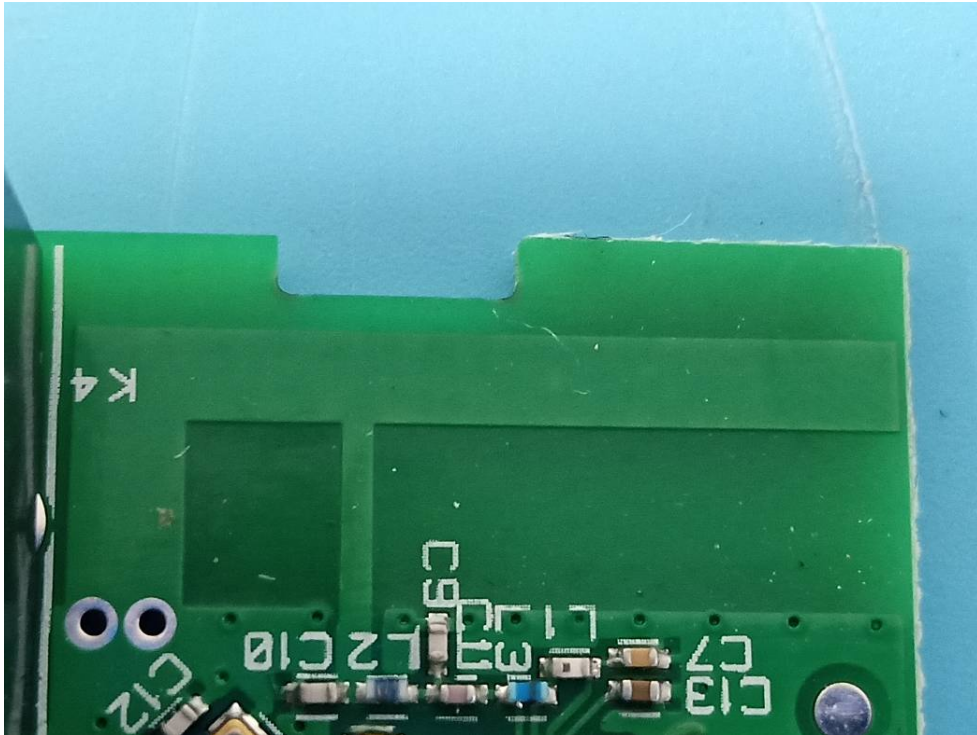
BLE&2.4G SRD Antenna
