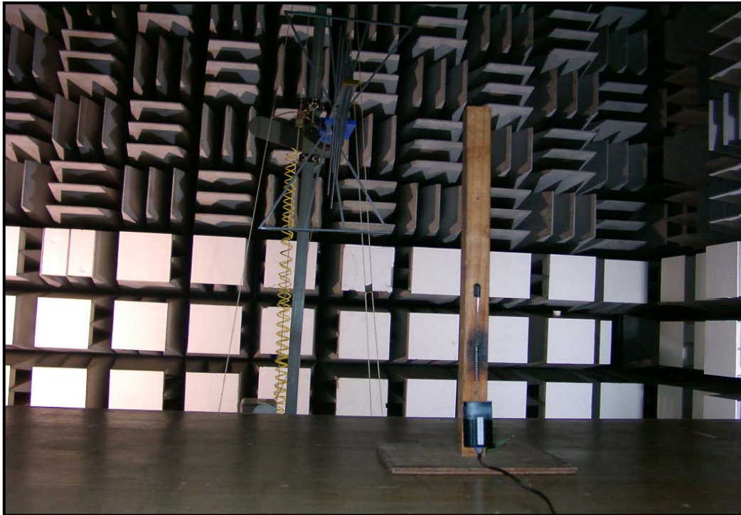
Photograph of the test configuration
