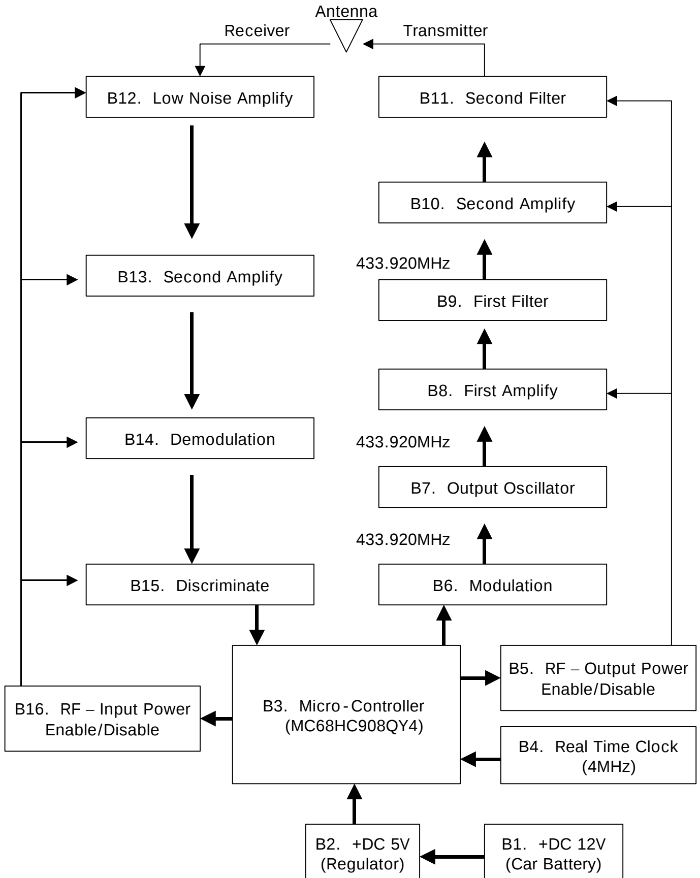
O44J2WAMANT Block Diagram (B1<Block1> ~ B16<Block16>)
