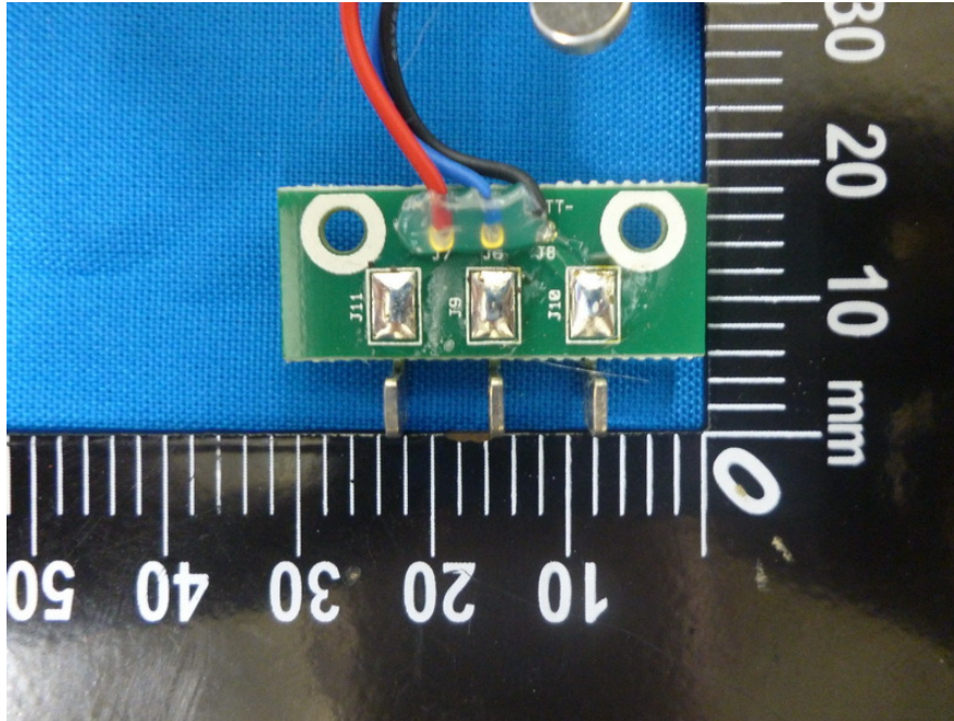
EUT – Main Board 2 Bottom View (Handset)
