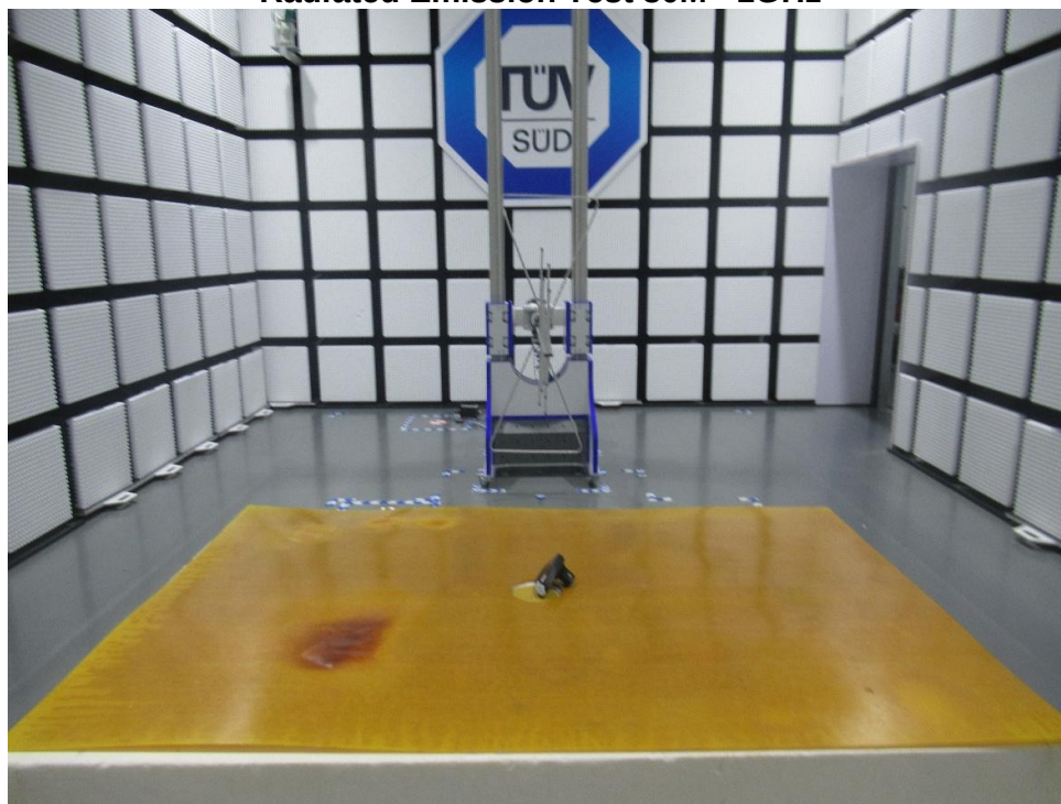
Radiated Emission Test 30M - 1GHz
