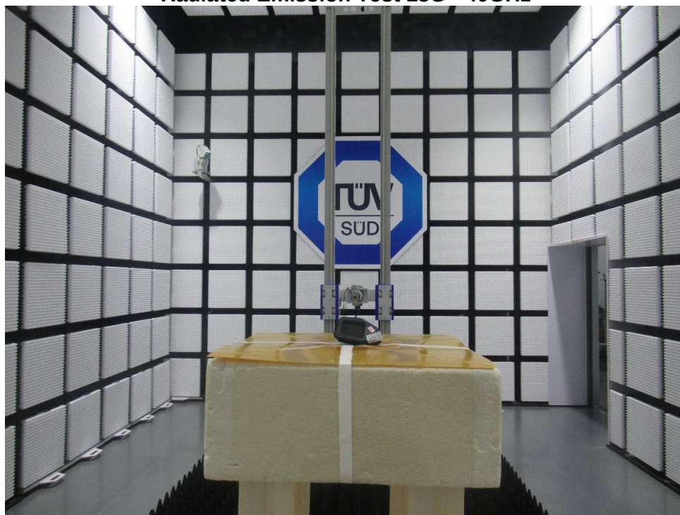
Radiated Emission Test 18G - 40GHz
