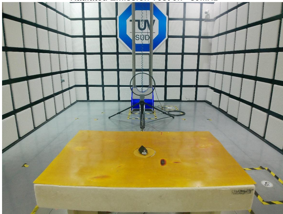
Radiated Emission Test 9k - 30MHz
