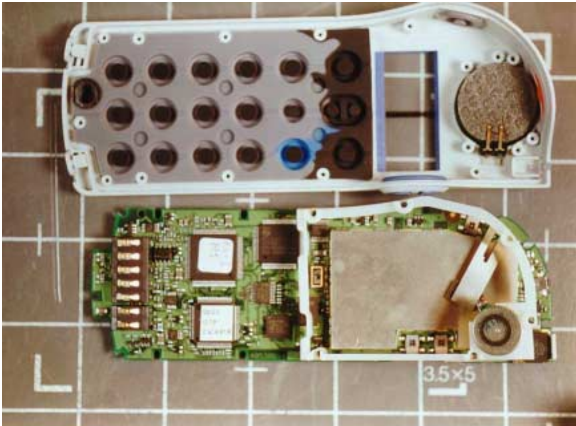
PCB Removed
