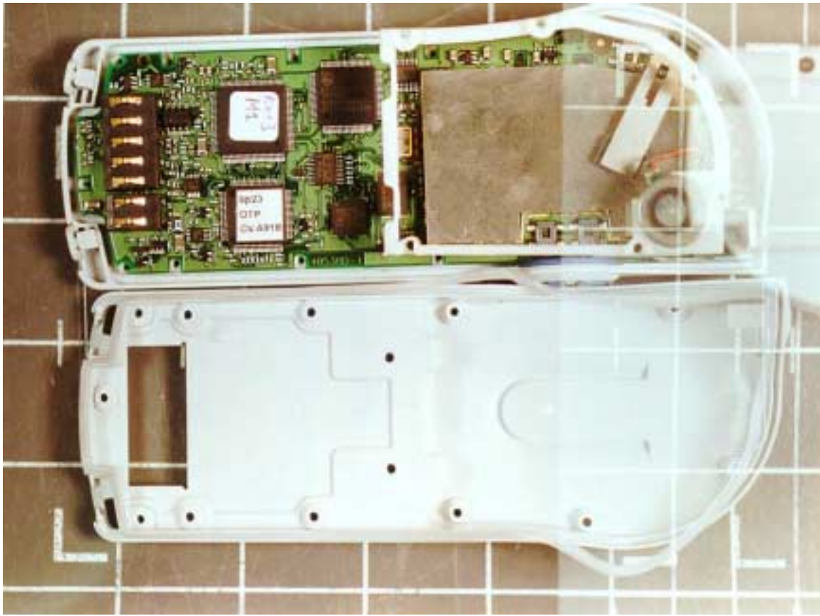
Cover Removed
