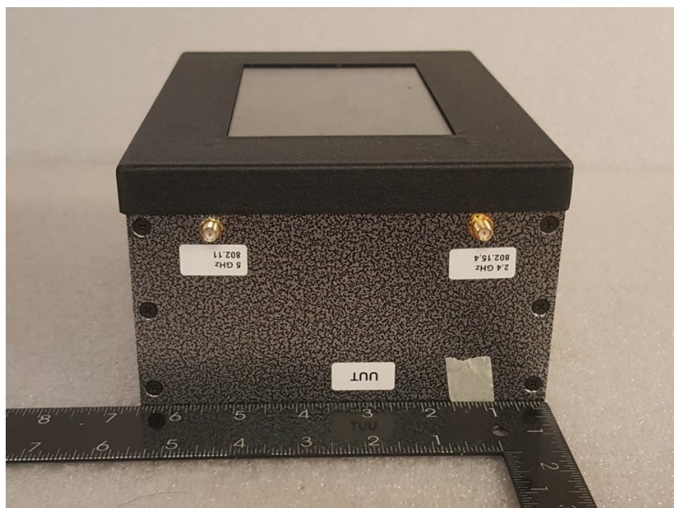
Figure 2 Front View
